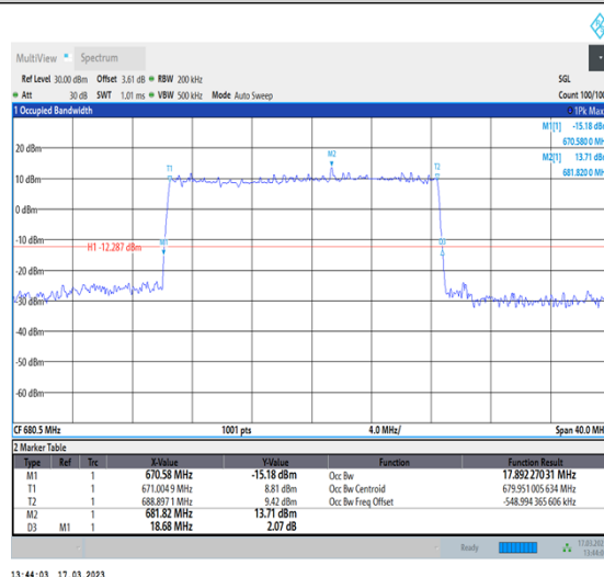
1-N71-PC3-15-20-M-3-DFT-16QAM-Outer_Full-100@0-Ant7-17.892-18.680-≤20-PASS
