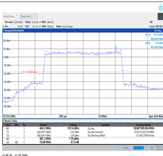
1-N71-PC3-15-20-L-9-CP-256QAM-Outer_Full-106@0-Ant7-18.848-19.680-≤20-PASS
