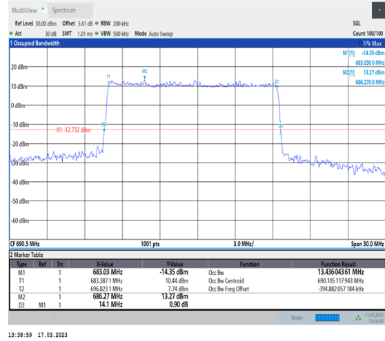
1-N71-PC3-15-15-H-3-DFT-16QAM-Outter_Full-75@0-Ant7-13.436-14.100-≤15-PASS
