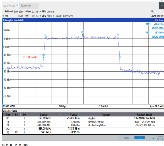
1-N71-PC3-15-15-M-3-DFT-16QAM-Outer_Full-75@0-Ant7-13.424-14.100-≤15-PASS
