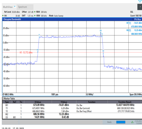
1-N71-PC3-15-15-M-5-DFT-256QAM-Outer_Full-75@0-Ant7-13.437-14.010-≤15-PASS
