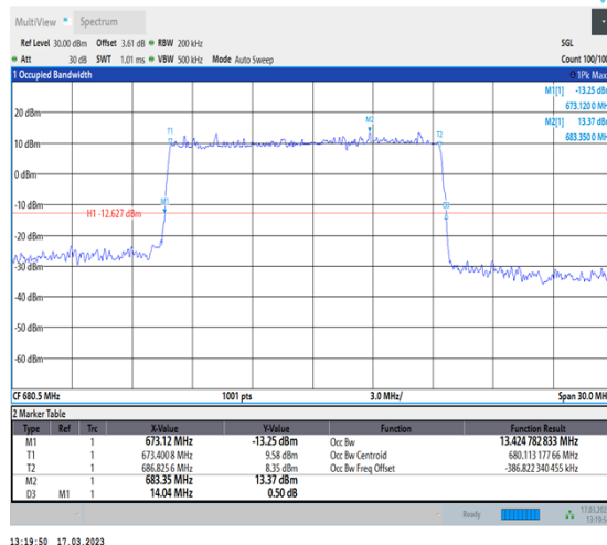
1-N71-PC3-15-15-M-4-DFT-64QAM-Outer_Full-75@0-Ant7-13.425-14.040-≤15-PASS
