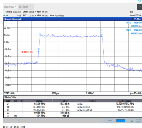
1-N71-PC3-15-15-H-5-DFT-256QAM-Outter_Full-75@0-Ant7-13.422-14.040-≤15-PASS
