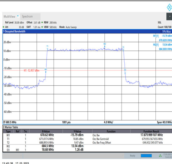
1-N71-PC3-15-20-M-2-DFT-PI2BPSK-Outer_Full-100@0-Ant7-17.876-18.680-≤20-PASS
