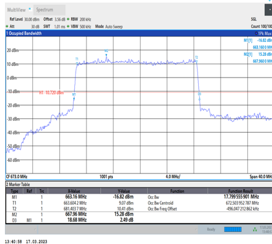
1-N71-PC3-15-20-L-2-DFT-PI2BPSK-Outer_Full-100@0-Ant7-17.8-18.680-≤20-PASS
