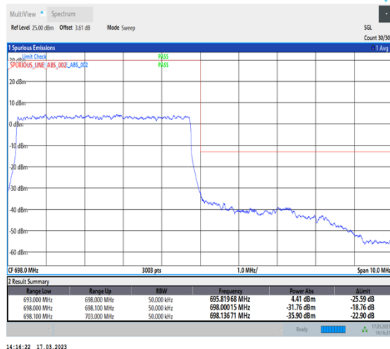
1-N71-PC3-15-5-H-3-DFT-PI2BPSK-Outer_Full-25@0-Ant7-1--PASS-see graph
