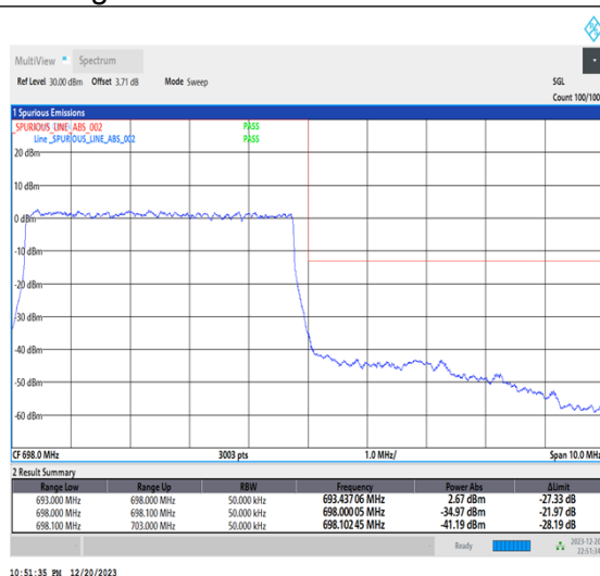
1-N71-15-5-H-3-DFT-PI2BPSK-Outer_Full-25@0-Ant7-1--PASS-see graph
