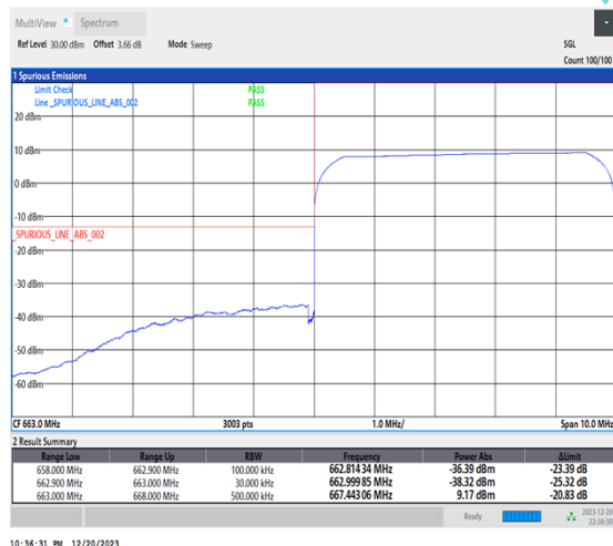
1-N71-15-5-L-6-CP-QPSK-Outer_Full-25@0-Ant7-1--PASS-see graph
