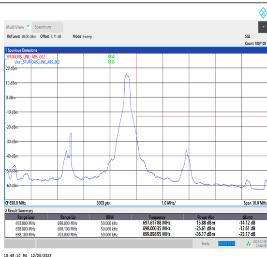
1-N71-15-5-H-2-DFT-PI2BPSK-Edge_1RB_Right-1@24-Ant7-1--PASS-see graph
