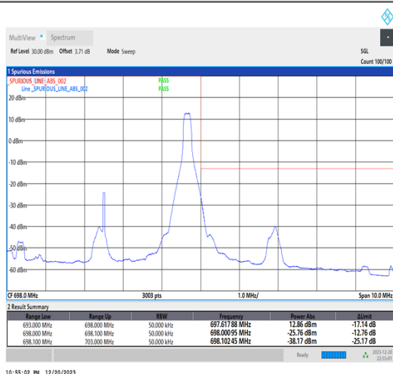
1-N71-15-5-H-5-CP-QPSK-Edge_1RB_Right-1@24-Ant7-1--PASS-see graph
