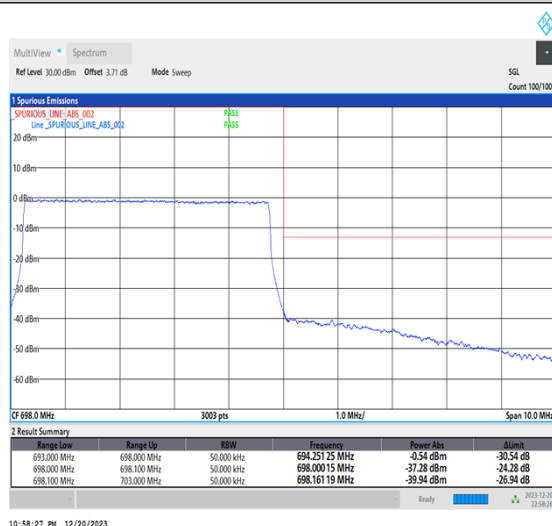
1-N71-15-5-H-6-CP-QPSK-Outer_Full-25@0-Ant7-1--PASS-see graph
