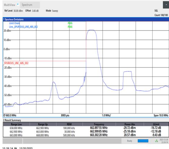
1-N71-15-5-L-1-DFT-PI2BPSK-Edge_1RB_Left-1@0-Ant7-1--PASS-see graph
