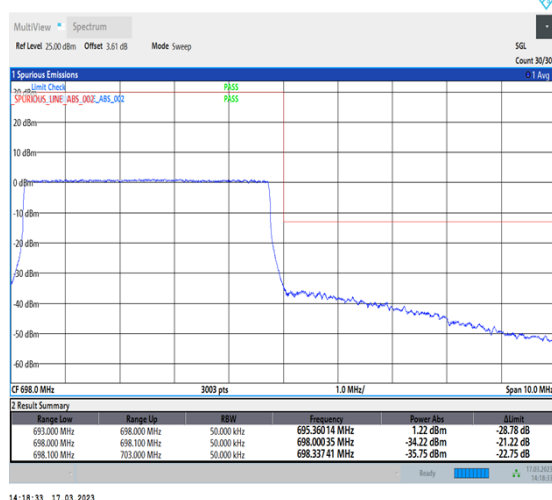
1-N71-PC3-15-5-H-6-CP-QPSK-Outer_Full-25@0-Ant7-1--PASS-see graph
