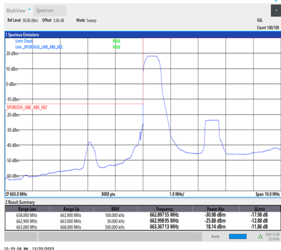
1-N71-15-5-L-4-CP-QPSK-Edge_1RB_Left-1@0-Ant7-1--PASS-see graph
