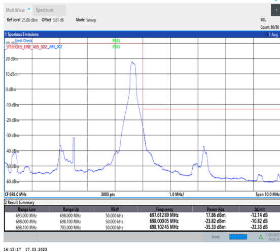
1-N71-PC3-15-5-H-2-DFT-PI2BPSK-Edge_1RB_Right-1@24-Ant7-1--PASS-see graph
