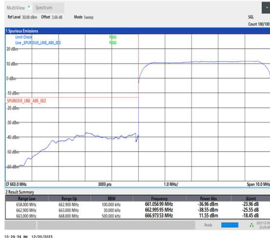
1-N71-15-5-L-3-DFT-PI2BPSK-Outer_Full-25@0-Ant7-1--PASS-see graph
