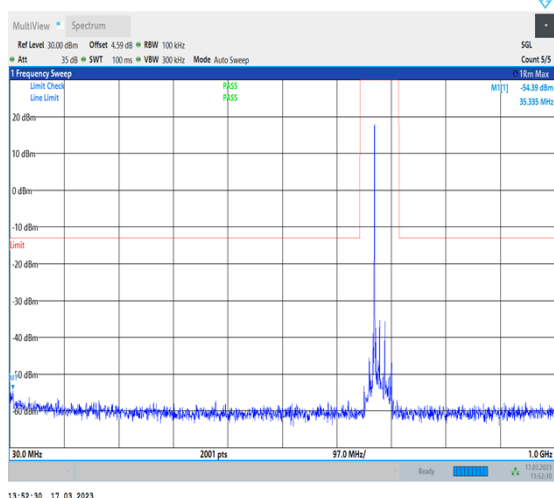
1-N71-PC3-15-20-H-1-DFT-PI2BPSK- Inner_1RB_Left-1@1-30-1000-Ant7-35.34--54.39-- 13-PASS
