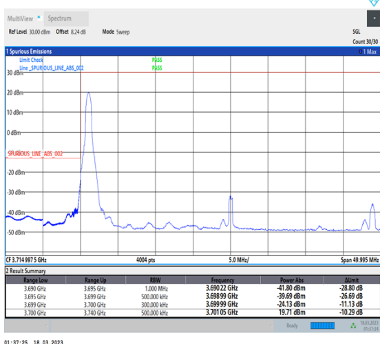
1-N77-3700-3980-30-40-L-4-CP-QPSK-Edge_1RB_Left-1@0-Ant0-1--PASS-see graph
