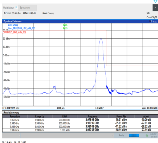
1-N77-3700-3980-30-20-H-5-CP-QPSK-Edge_1RB_Right-1@50-Ant0-1--PASS-see graph
