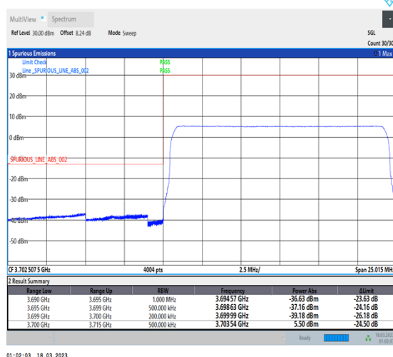
1-N77-3700-3980-30-15-L-6-CP-QPSK-Outer_Full-38@0-Ant0-1--PASS-see graph
