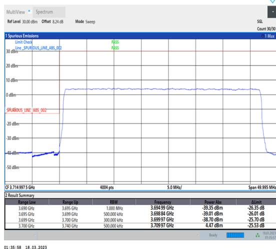
1-N77-3700-3980-30-40-L-3-DFT-PI2BPSK-Outer_Full-100@0-Ant0-1--PASS-see graph
