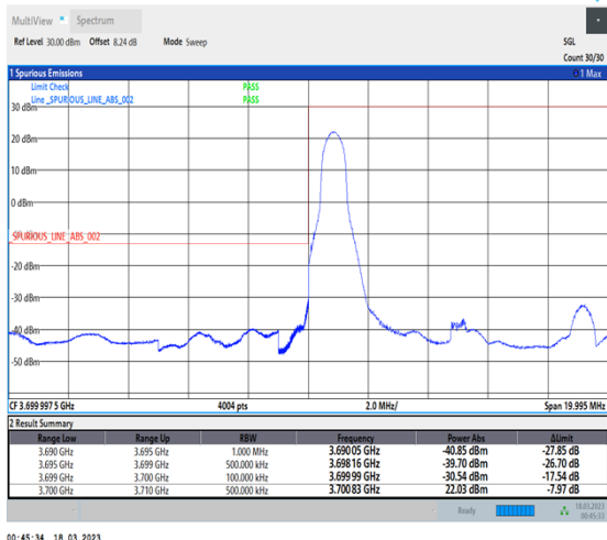
1-N77-3700-3980-30-10-L-1-DFT-PI2BPSK-Edge_1RB_Left-1@0-Ant0-1--PASS-see graph
