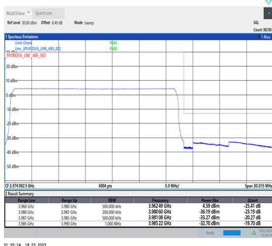
1-N77-3700-3980-30-20-H-6-CP-QPSK-Outer_Full-51@0-Ant0-1--PASS-see graph
