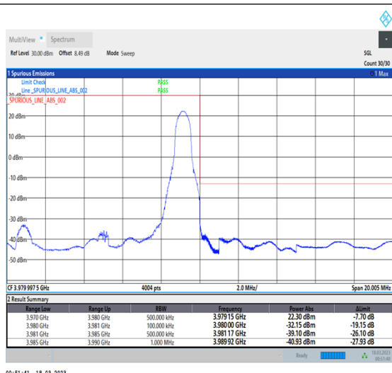
1-N77-3700-3980-30-10-H-2-DFT-PI2BPSK-Edge_1RB_Right-1@23-Ant0-1--PASS-see graph
