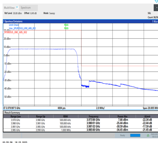
1-N77-3700-3980-30-10-H-6-CP-QPSK-Outer_Full-24@0-Ant0-1--PASS-see graph
