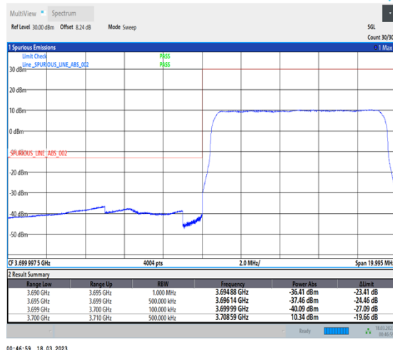
1-N77-3700-3980-30-10-L-3-DFT-PI2BPSK-Outer_Full-24@0-Ant0-1--PASS-see graph
