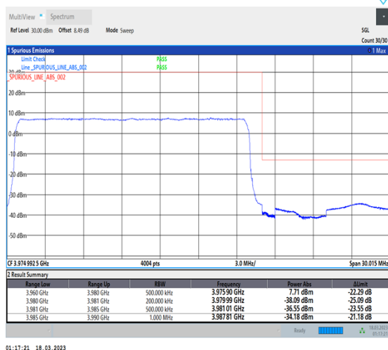
1-N77-3700-3980-30-20-H-3-DFT-PI2BPSK-Outer_Full-50@0-Ant0-1--PASS-see graph
