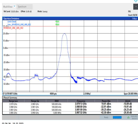
1-N77-3700-3980-30-10-H-5-CP-QPSK-Edge_1RB_Right-1@23-Ant0-1--PASS-see graph
