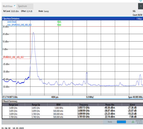
1-N77-3700-3980-30-40-L-1-DFT-PI2BPSK-Edge_1RB_Left-1@0-Ant0-1--PASS-see graph
