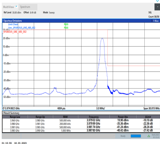
1-N77-3700-3980-30-20-H-2-DFT-PI2BPSK-Edge_1RB_Right-1@50-Ant0-1--PASS-see graph
