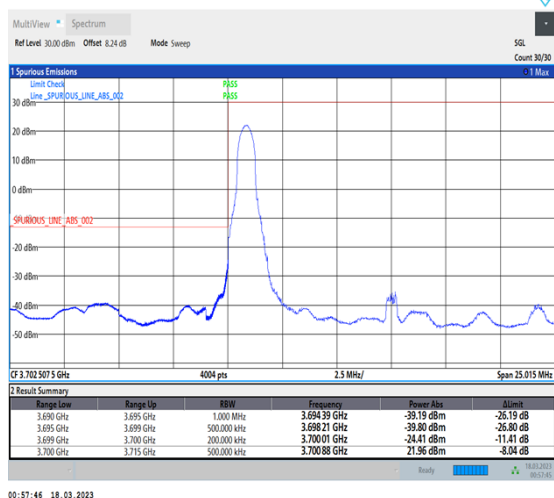
1-N77-3700-3980-30-15-L-1-DFT-PI2BPSK-Edge_1RB_Left-1@0-Ant0-1--PASS-see graph
