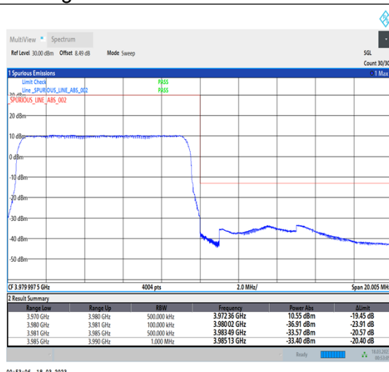
1-N77-3700-3980-30-10-H-3-DFT-PI2BPSK-Outer_Full-24@0-Ant0-1--PASS-see graph
