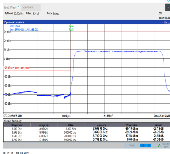
1-N77-3700-3980-30-15-L-3-DFT-PI2BPSK-Outer_Full-36@0-Ant0-1--PASS-see graph
