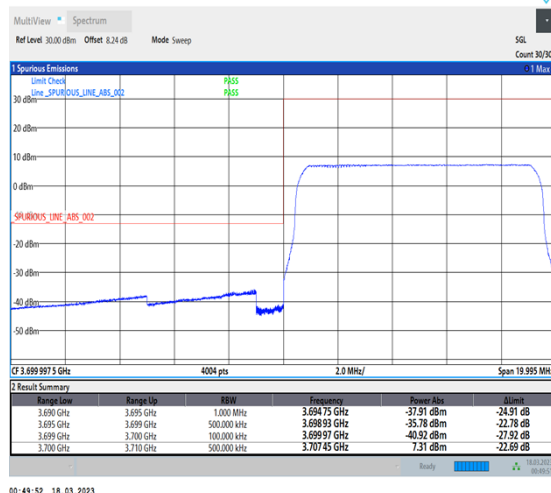
1-N77-3700-3980-30-10-L-6-CP-QPSK-Outer_Full-24@0-Ant0-1--PASS-see graph
