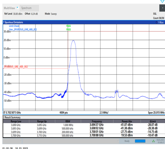
1-N77-3700-3980-30-15-L-4-CP-QPSK-Edge_1RB_Left-1@0-Ant0-1--PASS-see graph
