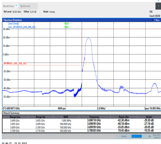
1-N77-3700-3980-30-10-L-4-CP-QPSK-Edge_1RB_Left-1@0-Ant0-1--PASS-see graph
