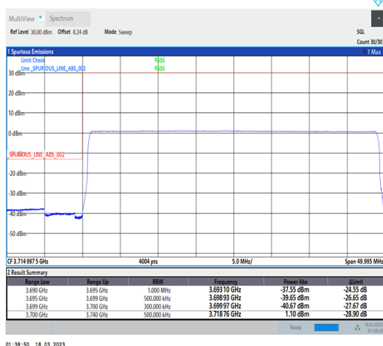
1-N77-3700-3980-30-40-L-6-CP-QPSK-Outer_Full-106@0-Ant0-1--PASS-see graph
