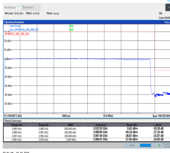
1-N77-3700-3980-30-90-H-3-DFT-PI2BPSK-Outer_Full-240@0-Ant0-1--PASS-see graph
