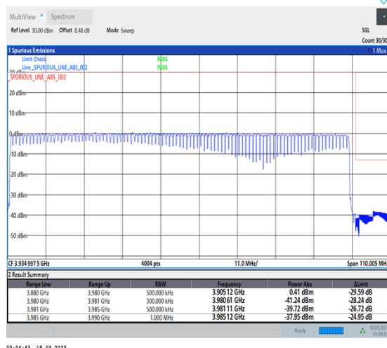
1-N77-3700-3980-30-100-H-3-DFT-PI2BPSK-Outer_Full-270@0-Ant0-1--PASS-see graph
