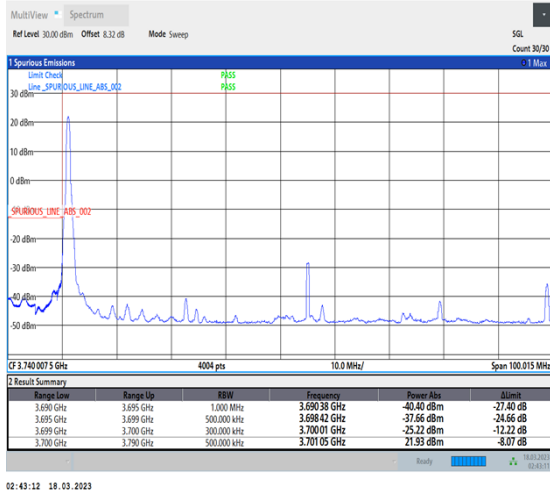
1-N77-3700-3980-30-90-L-1-DFT-PI2BPSK-Edge_1RB_Left-1@0-Ant0-1--PASS-see graph
