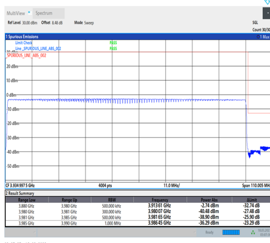
1-N77-3700-3980-30-100-H-6-CP-QPSK-Outer_Full-273@0-Ant0-1--PASS-see graph
