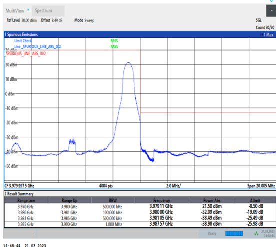
1-N77-3700-3980-30-10-H-5-CP-QPSK-Edge_1RB_Right-1@23-Ant0-1--PASS-see graph
