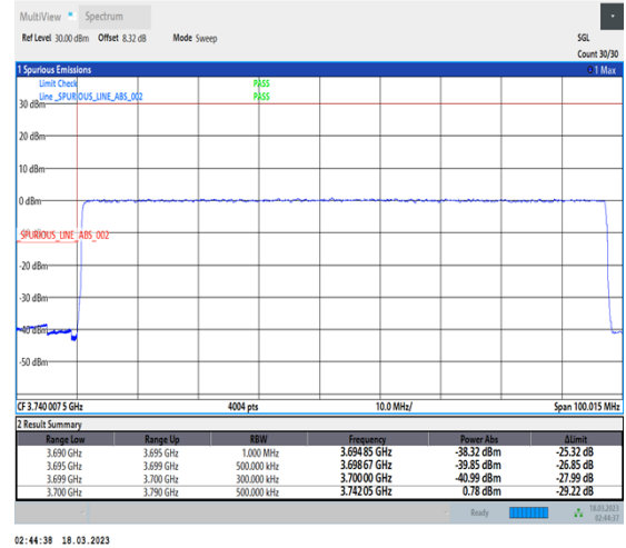
1-N77-3700-3980-30-90-L-3-DFT-PI2BPSK-Outer_Full-240@0-Ant0-1--PASS-see graph
