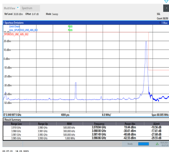
1-N77-3700-3980-30-70-H-5-CP-QPSK-Edge_1RB_Right-1@188-Ant0-1--PASS-see graph
