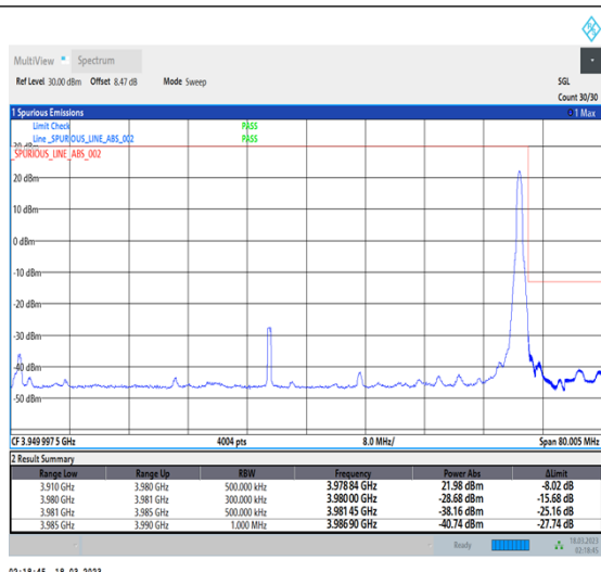
1-N77-3700-3980-30-70-H-2-DFT-PI2BPSK-Edge_1RB_Right-1@188-Ant0-1--PASS-see graph
