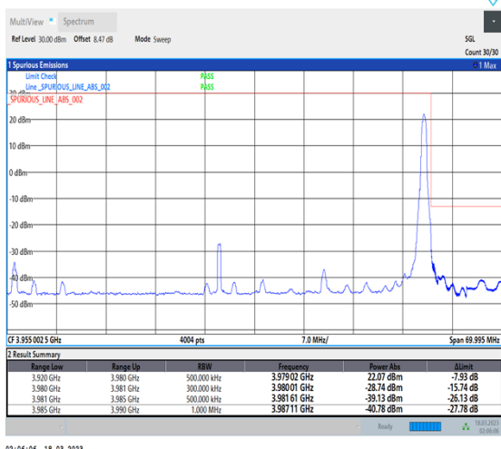
1-N77-3700-3980-30-60-H-2-DFT-PI2BPSK-Edge_1RB_Right-1@161-Ant0-1--PASS-see graph
