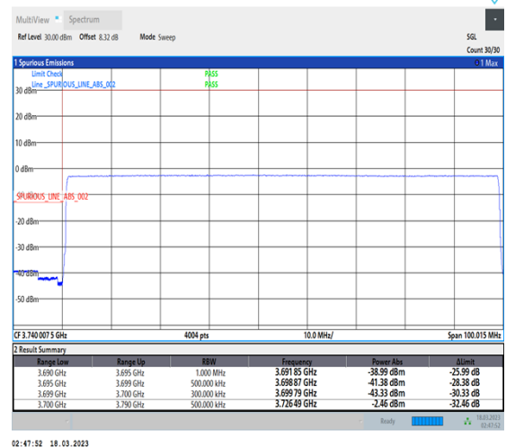
1-N77-3700-3980-30-90-L-6-CP-QPSK-Outer_Full-245@0-Ant0-1--PASS-see graph
