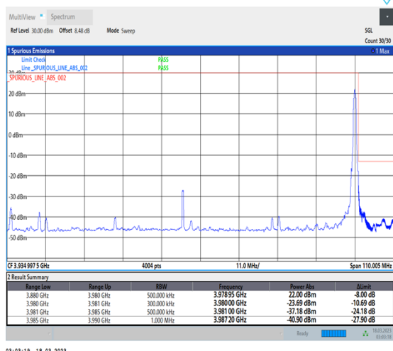
1-N77-3700-3980-30-100-H-2-DFT-PI2BPSK-Edge_1RB_Right-1@272-Ant0-1--PASS-see graph
