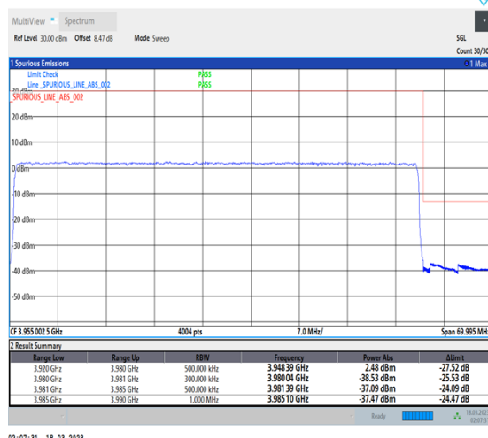
1-N77-3700-3980-30-60-H-3-DFT-PI2BPSK-Outer_Full-162@0-Ant0-1--PASS-see graph
