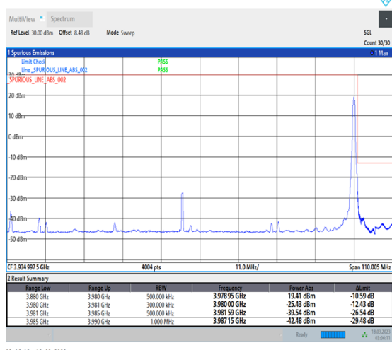
1-N77-3700-3980-30-100-H-5-CP-QPSK-Edge_1RB_Right-1@272-Ant0-1--PASS-see graph
