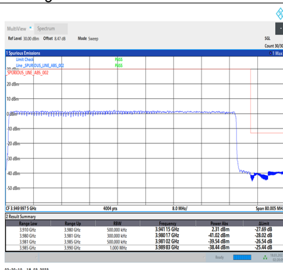
1-N77-3700-3980-30-70-H-3-DFT-PI2BPSK-Outer_Full-180@0-Ant0-1--PASS-see graph
