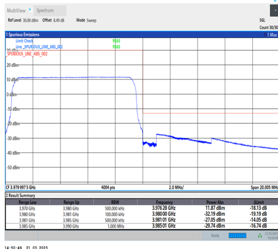
1-N77-3700-3980-30-10-H-6-CP-QPSK-Outer_Full-24@0-Ant0-1--PASS-see graph
