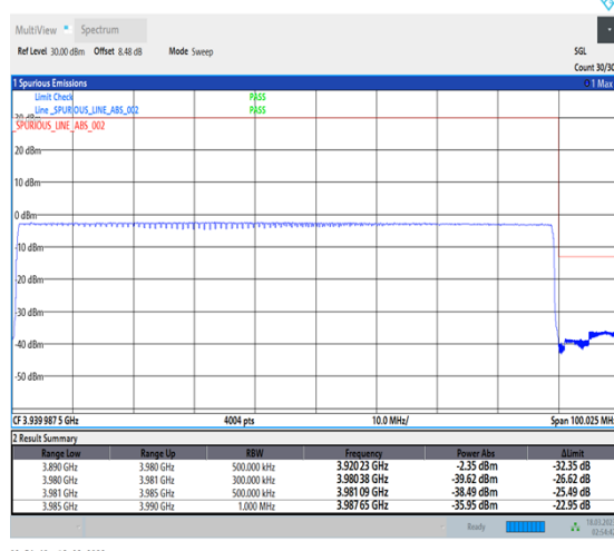
1-N77-3700-3980-30-90-H-6-CP-QPSK-Outer_Full-245@0-Ant0-1--PASS-see graph
