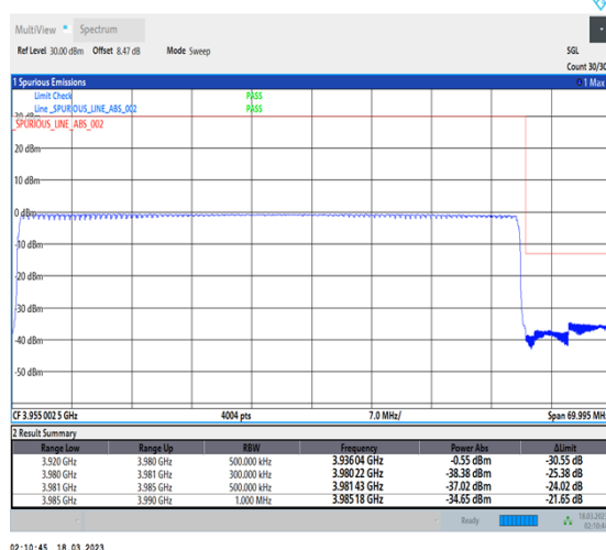
1-N77-3700-3980-30-60-H-6-CP-QPSK-Outer_Full-162@0-Ant0-1--PASS-see graph
