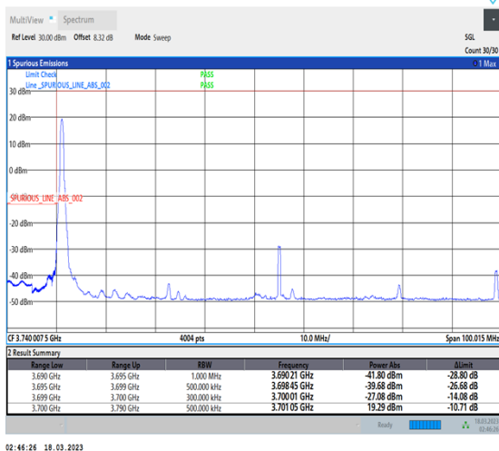
1-N77-3700-3980-30-90-L-4-CP-QPSK-Edge_1RB_Left-1@0-Ant0-1--PASS-see graph
