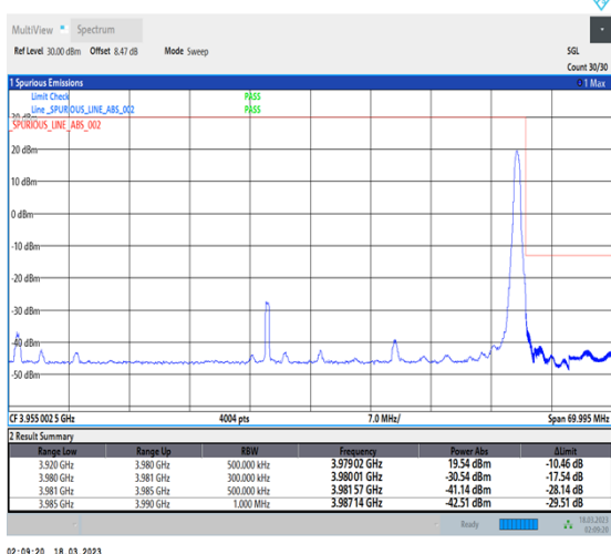
1-N77-3700-3980-30-60-H-5-CP-QPSK-Edge_1RB_Right-1@161-Ant0-1--PASS-see graph
