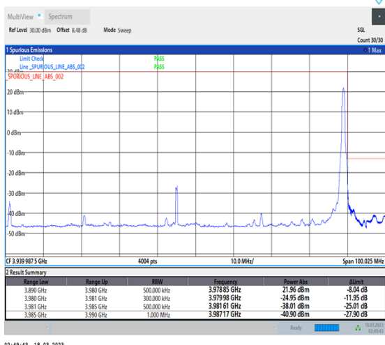
1-N77-3700-3980-30-90-H-2-DFT-PI2BPSK-Edge_1RB_Right-1@244-Ant0-1--PASS-see graph
