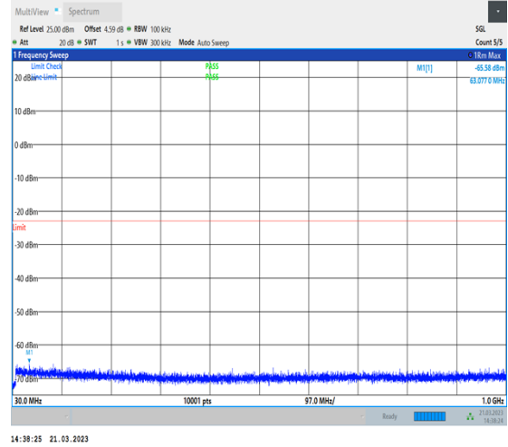
1-N77-3700-3980-30-100-M-1-DFT-QPSK- Edge_1RB_Left-1@0-30-1000-Ant0-63.08--65.58-- 23-PASS
