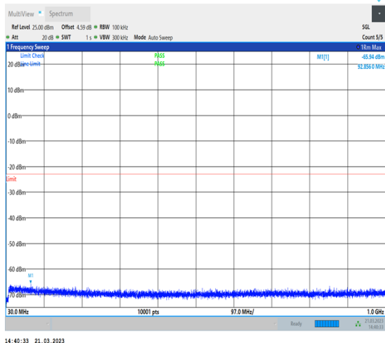
1-N77-3700-3980-30-100-H-1-DFT-QPSK- Edge_1RB_Left-1@0-30-1000-Ant0-92.86--65.94-- 23-PASS
