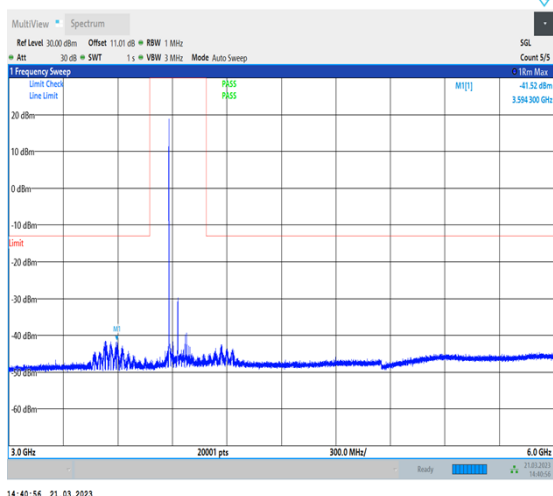
1-N77-3700-3980-30-100-H-1-DFT-QPSK- Edge_1RB_Left-1@0-3000-6000-Ant0-3594.30-- 41.52--13-PASS
