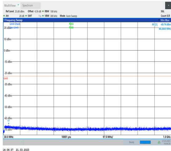
1-N77-3700-3980-30-100-L-1-DFT-QPSK- Edge_1RB_Left-1@0-30-1000-Ant0-60.26--65.74-- 23-PASS
