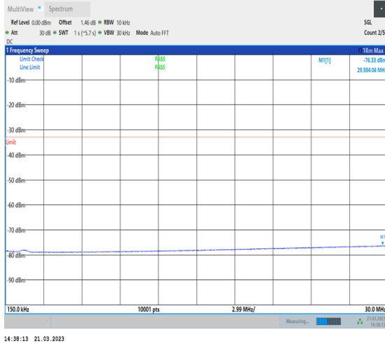
1-N77-3700-3980-30-100-M-1-DFT-QPSK- Edge_1RB_Left-1@0-0.15-30-Ant0-29.59--76.33-- 33-PASS
