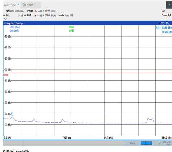
1-N77-3700-3980-30-100-L-1-DFT-QPSK- Edge_1RB_Left-1@0-0.009-0.15-Ant0-0.02--82.89-- 43-PASS
