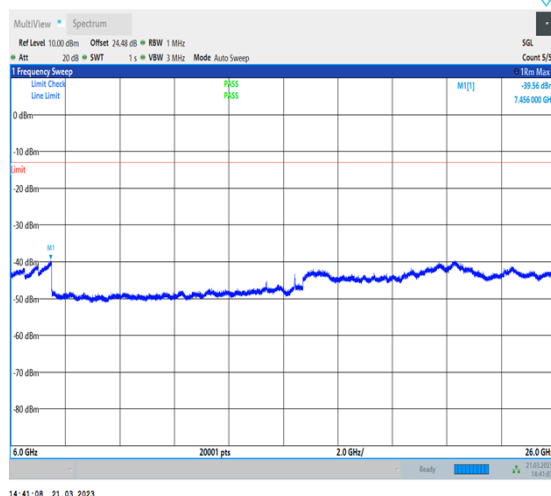
1-N77-3700-3980-30-100-H-1-DFT-QPSK- Edge_1RB_Left-1@0-6000-26000-Ant0-7456.00-- 39.56--13-PASS
