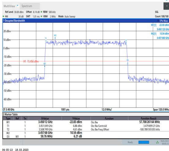
1-N78-3450-3550-30-60-L-3-DFT-16QAM-Outer_Full-162@0-Ant0-57.7-59.760-≤60-PASS
