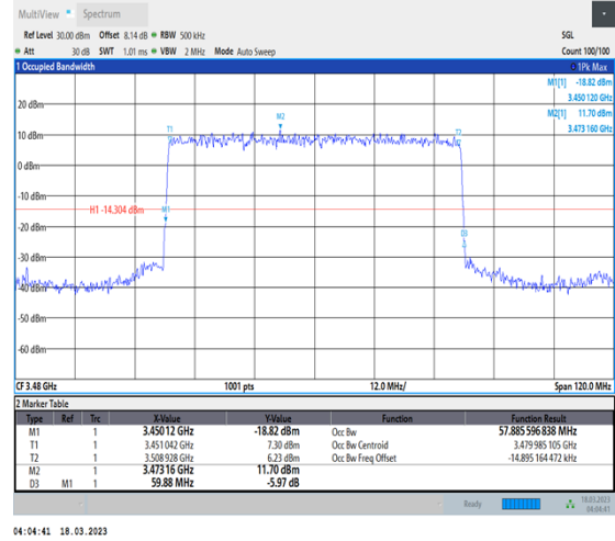
1-N78-3450-3550-30-60-L-2-DFT-PI2BPSK-Outer_Full-162@0-Ant0-57.886-59.880-≤60-PASS
