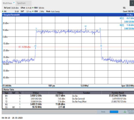
1-N78-3450-3550-30-60-L-1-DFT-QPSK-Outer_Full-162@0-Ant0-57.873-59.760-≤60-PASS
