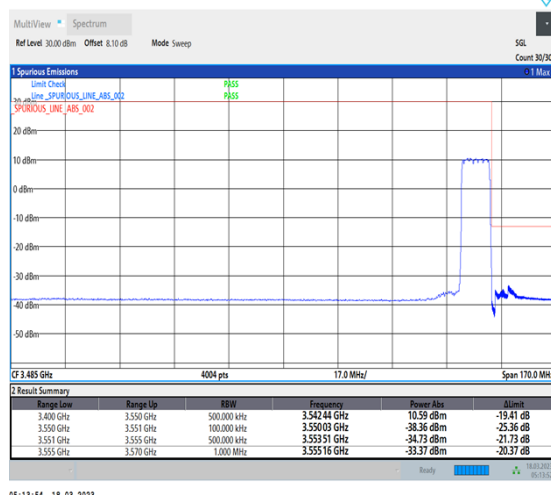
1-N78-3450-3550-30-10-H-3-DFT-PI2BPSK-Outer_Full-24@0-Ant0-1--PASS-see graph
