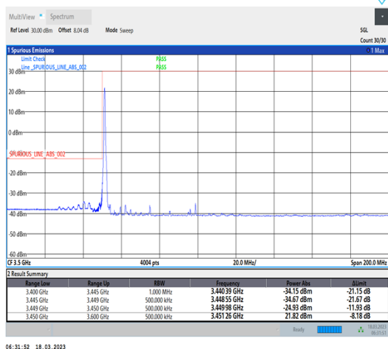
1-N78-3450-3550-30-50-L-1-DFT-PI2BPSK-Edge_1RB_Left-1@0-Ant0-1--PASS-see graph
