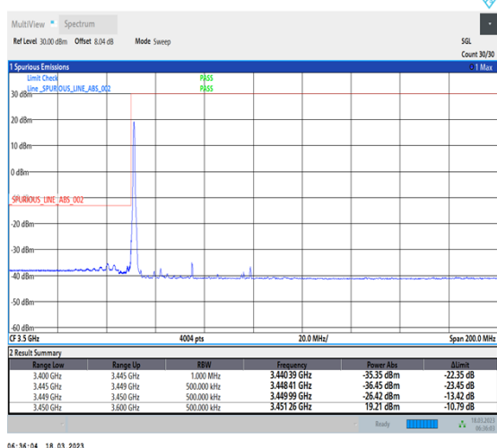
1-N78-3450-3550-30-50-L-4-CP-QPSK-Edge_1RB_Left-1@0-Ant0-1--PASS-see graph
