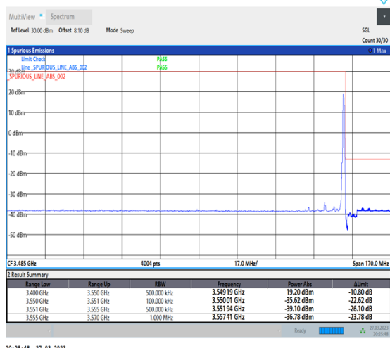
1-N78-3450-3550-30-10-H-2-DFT-PI2BPSK-Edge_1RB_Right-1@23-Ant0-1--PASS-see graph
