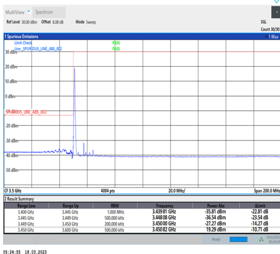
1-N78-3450-3550-30-15-L-4-CP-QPSK-Edge_1RB_Left-1@0-Ant0-1--PASS-see graph
