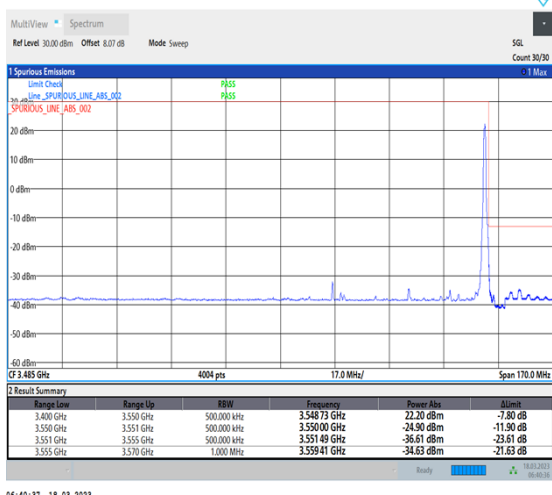
1-N78-3450-3550-30-50-H-2-DFT-PI2BPSK-Edge_1RB_Right-1@132-Ant0-1--PASS-see graph
