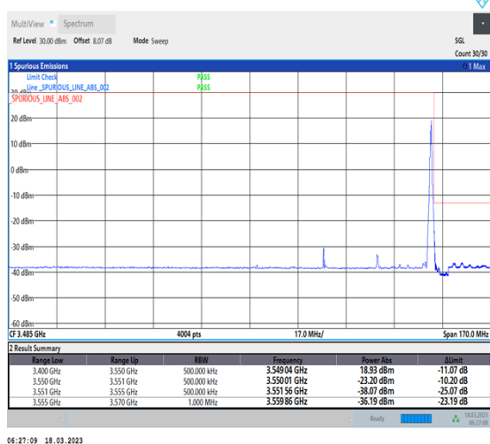
1-N78-3450-3550-30-40-H-5-CP-QPSK-Edge_1RB_Right-1@105-Ant0-1--PASS-see graph
