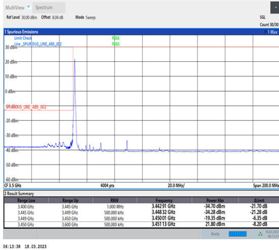
1-N78-3450-3550-30-40-L-1-DFT-PI2BPSK-Edge_1RB_Left-1@0-Ant0-1--PASS-see graph
