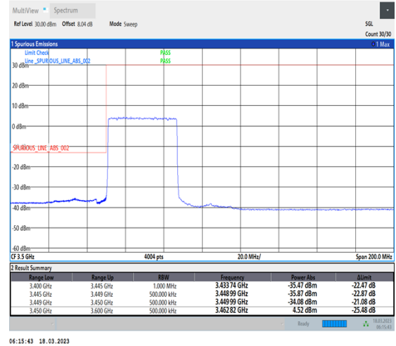
1-N78-3450-3550-30-40-L-3-DFT-PI2BPSK-Outer_Full-100@0-Ant0-1--PASS-see graph
