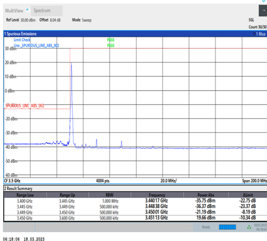
1-N78-3450-3550-30-40-L-4-CP-QPSK-Edge_1RB_Left-1@0-Ant0-1--PASS-see graph
