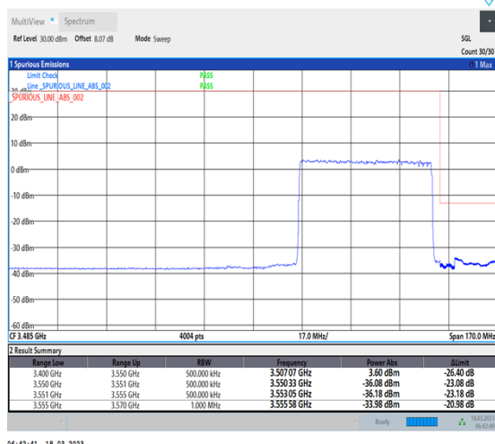
1-N78-3450-3550-30-50-H-3-DFT-PI2BPSK-Outer_Full-128@0-Ant0-1--PASS-see graph
