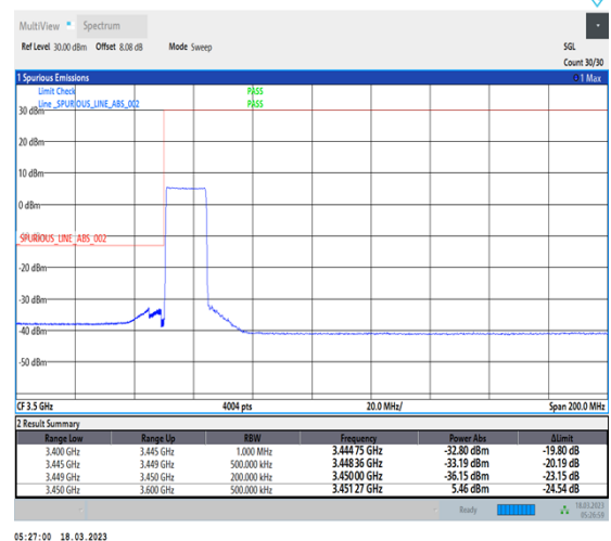
1-N78-3450-3550-30-15-L-6-CP-QPSK-Outer_Full-38@0-Ant0-1--PASS-see graph
