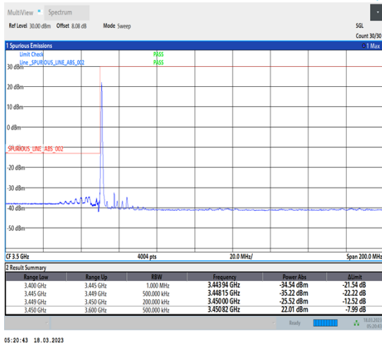
1-N78-3450-3550-30-15-L-1-DFT-PI2BPSK-Edge_1RB_Left-1@0-Ant0-1--PASS-see graph
