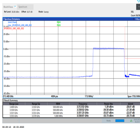
1-N78-3450-3550-30-40-H-6-CP-QPSK-Outer_Full-106@0-Ant0-1--PASS-see graph
