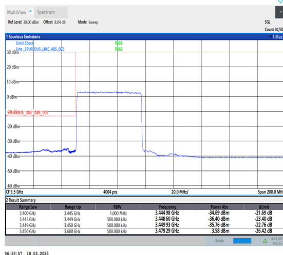
1-N78-3450-3550-30-50-L-3-DFT-PI2BPSK-Outer_Full-128@0-Ant0-1--PASS-see graph
