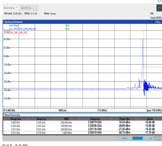
1-N78-3450-3550-30-10-H-5-CP-QPSK-Edge_1RB_Right-1@23-Ant0-1--PASS-see graph
