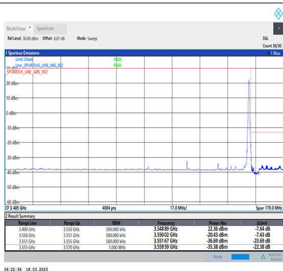
1-N78-3450-3550-30-40-H-2-DFT-PI2BPSK-Edge_1RB_Right-1@105-Ant0-1--PASS-see graph
