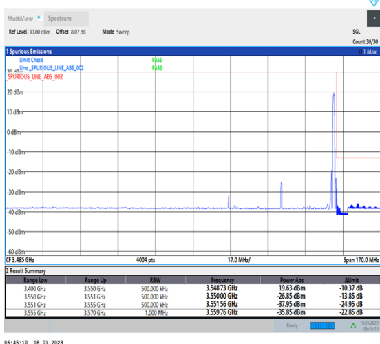
1-N78-3450-3550-30-50-H-5-CP-QPSK-Edge_1RB_Right-1@132-Ant0-1--PASS-see graph
