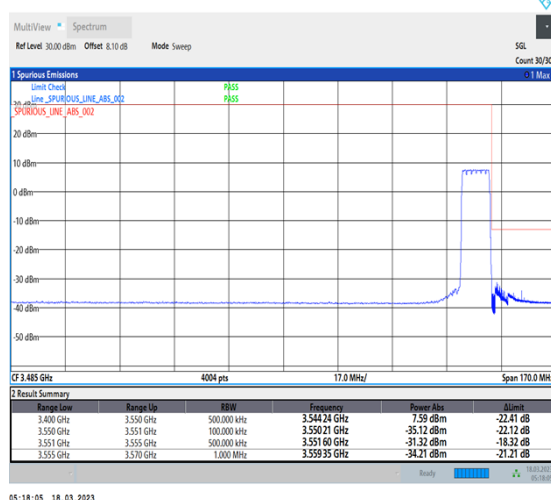
1-N78-3450-3550-30-10-H-6-CP-QPSK-Outer_Full-24@0-Ant0-1--PASS-see graph
