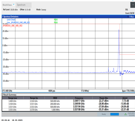
1-N78-3450-3550-30-15-H-2-DFT-PI2BPSK-Edge_1RB_Right-1@37-Ant0-1--PASS-see graph
