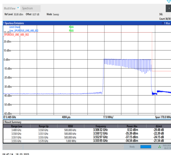
1-N78-3450-3550-30-50-H-6-CP-QPSK-Outer_Full-133@0-Ant0-1--PASS-see graph
