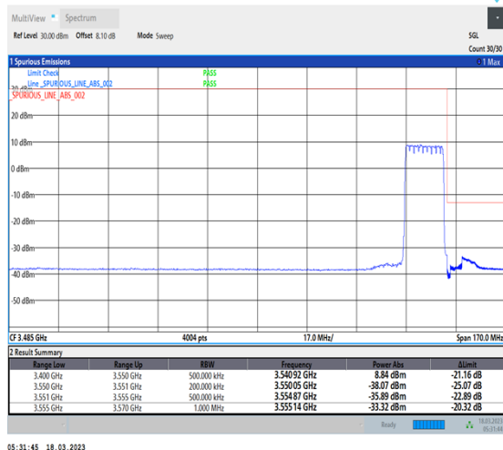
1-N78-3450-3550-30-15-H-3-DFT-PI2BPSK-Outer_Full-36@0-Ant0-1--PASS-see graph
