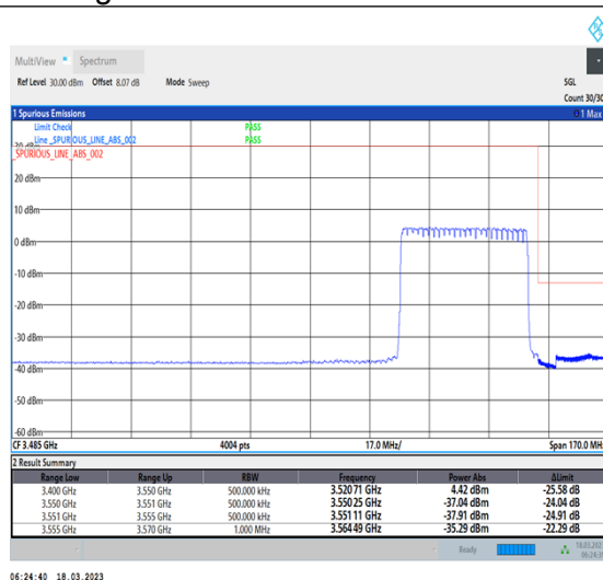
1-N78-3450-3550-30-40-H-3-DFT-PI2BPSK-Outer_Full-100@0-Ant0-1--PASS-see graph
