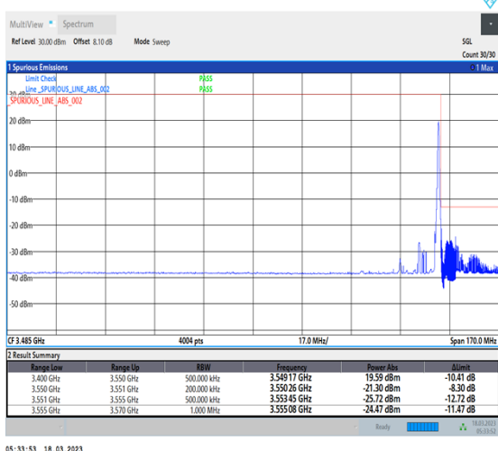
1-N78-3450-3550-30-15-H-5-CP-QPSK-Edge_1RB_Right-1@37-Ant0-1--PASS-see graph
