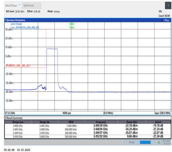
1-N78-3450-3550-30-15-L-3-DFT-PI2BPSK-Outer_Full-36@0-Ant0-1--PASS-see graph
