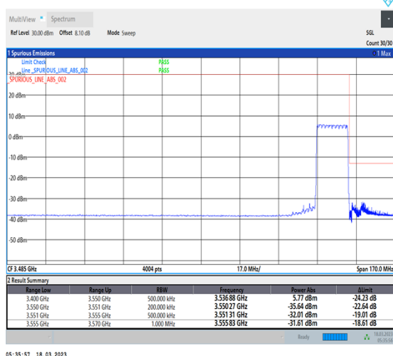
1-N78-3450-3550-30-15-H-6-CP-QPSK-Outer_Full-38@0-Ant0-1--PASS-see graph
