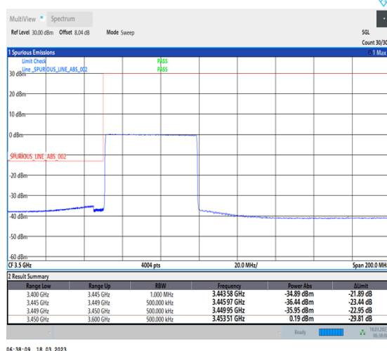
1-N78-3450-3550-30-50-L-6-CP-QPSK-Outer_Full-133@0-Ant0-1--PASS-see graph
