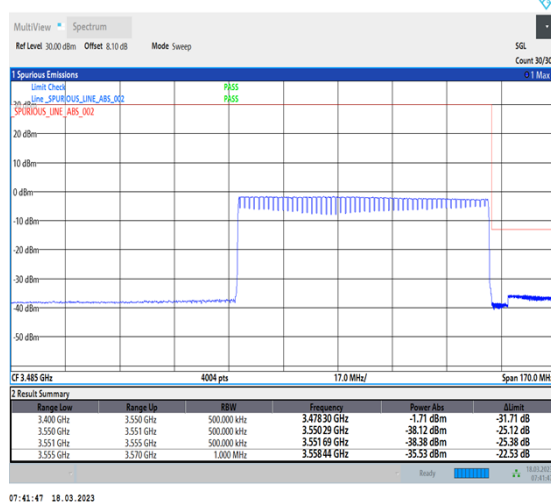
1-N78-3450-3550-30-80-H-6-CP-QPSK-Outer_Full-217@0-Ant0-1--PASS-see graph
