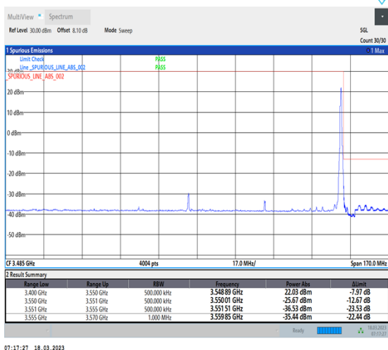
1-N78-3450-3550-30-70-H-2-DFT-PI2BPSK-Edge_1RB_Right-1@188-Ant0-1--PASS-see graph
