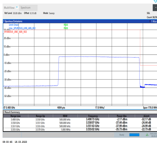
1-N78-3450-3550-30-90-H-6-CP-QPSK-Outer_Full-245@0-Ant0-1--PASS-see graph
