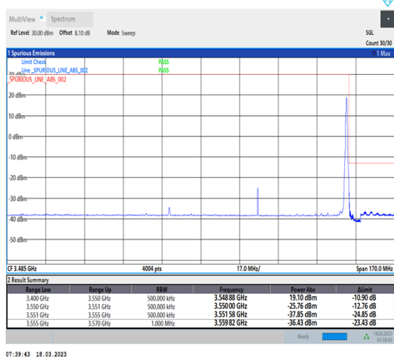
1-N78-3450-3550-30-80-H-5-CP-QPSK-Edge_1RB_Right-1@216-Ant0-1--PASS-see graph
