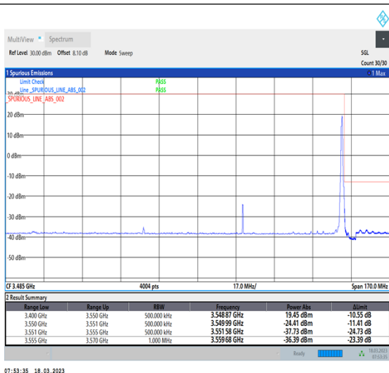
1-N78-3450-3550-30-90-H-2-DFT-PI2BPSK-Edge_1RB_Right-1@244-Ant0-1--PASS-see graph
