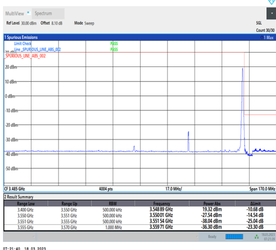
1-N78-3450-3550-30-70-H-5-CP-QPSK-Edge_1RB_Right-1@188-Ant0-1--PASS-see graph
