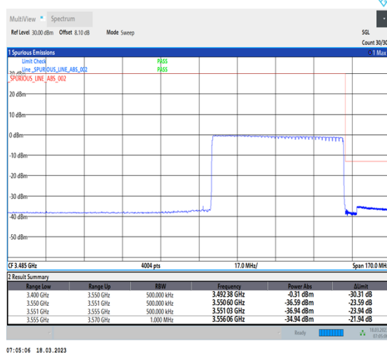
1-N78-3450-3550-30-60-H-6-CP-QPSK-Outer_Full-162@0-Ant0-1--PASS-see graph
