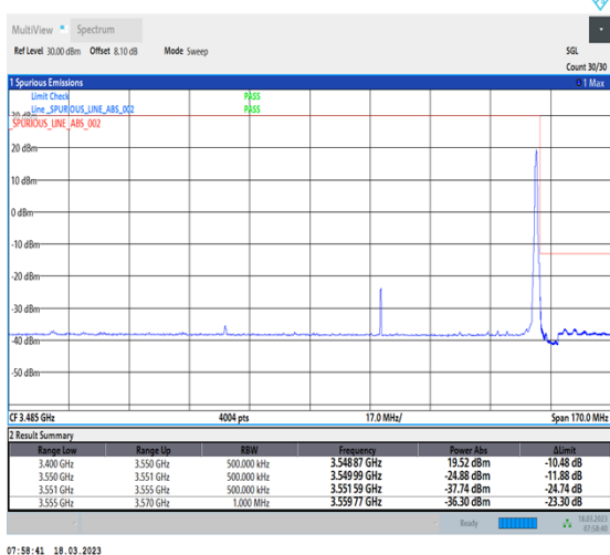
1-N78-3450-3550-30-90-H-5-CP-QPSK-Edge_1RB_Right-1@244-Ant0-1--PASS-see graph
