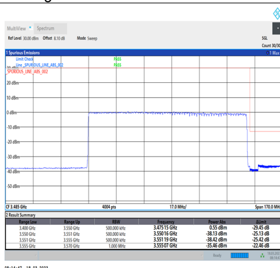
1-N78-3450-3550-30-100-H-3-DFT-PI2BPSK-Outer_Full-270@0-Ant0-1--PASS-see graph
