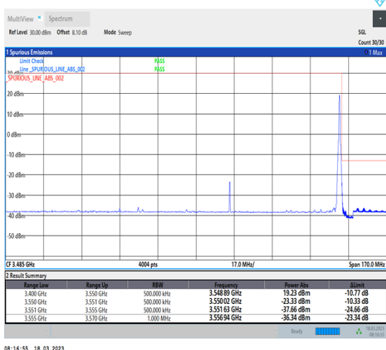
1-N78-3450-3550-30-100-H-5-CP-QPSK-Edge_1RB_Right-1@272-Ant0-1--PASS-see graph
