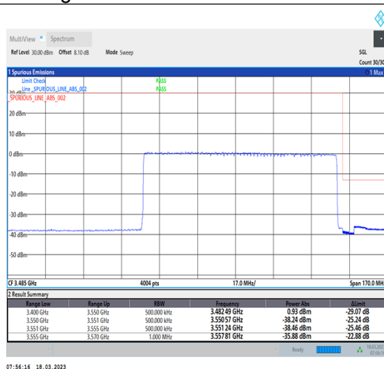
1-N78-3450-3550-30-90-H-3-DFT-PI2BPSK-Outer_Full-240@0-Ant0-1--PASS-see graph
