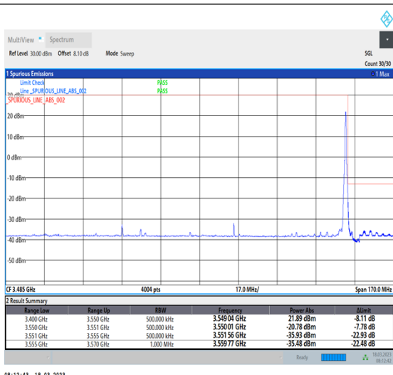
1-N78-3450-3550-30-100-H-2-DFT-PI2BPSK-Edge_1RB_Right-1@272-Ant0-1--PASS-see graph
