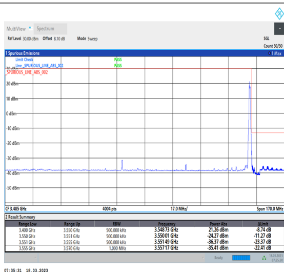
1-N78-3450-3550-30-80-H-2-DFT-PI2BPSK-Edge_1RB_Right-1@216-Ant0-1--PASS-see graph
