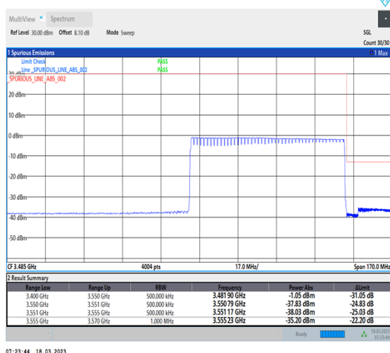
1-N78-3450-3550-30-70-H-6-CP-QPSK-Outer_Full-189@0-Ant0-1--PASS-see graph
