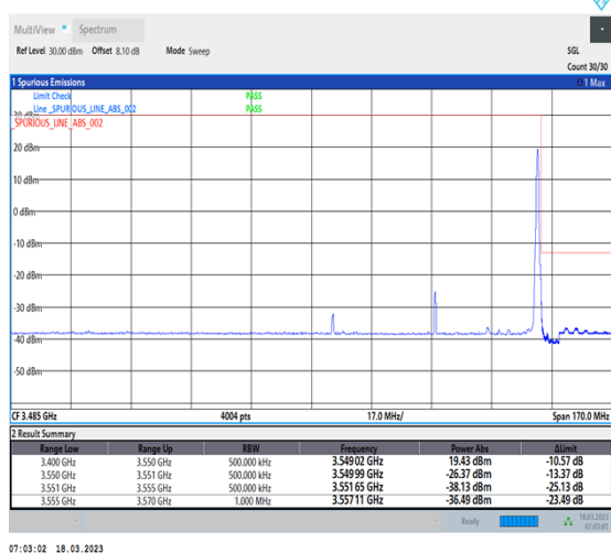
1-N78-3450-3550-30-60-H-5-CP-QPSK-Edge_1RB_Right-1@161-Ant0-1--PASS-see graph
