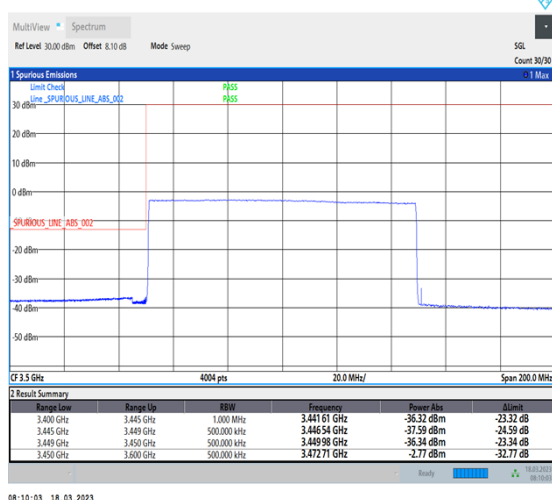
1-N78-3450-3550-30-100-L-6-CP-QPSK-Outer_Full-273@0-Ant0-1--PASS-see graph
