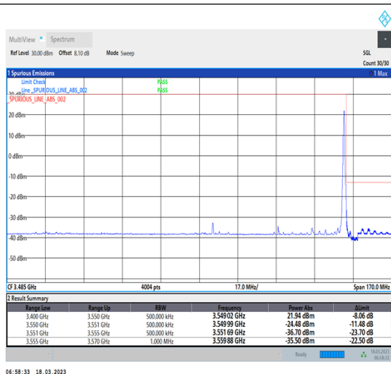
1-N78-3450-3550-30-60-H-2-DFT-PI2BPSK-Edge_1RB_Right-1@161-Ant0-1--PASS-see graph
