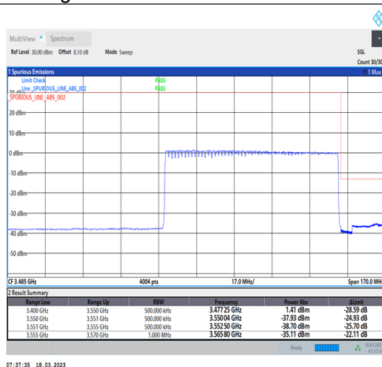
1-N78-3450-3550-30-80-H-3-DFT-PI2BPSK-Outer_Full-216@0-Ant0-1--PASS-see graph
