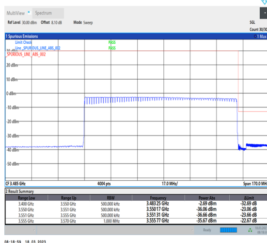
1-N78-3450-3550-30-100-H-6-CP-QPSK-Outer_Full-273@0-Ant0-1--PASS-see graph
