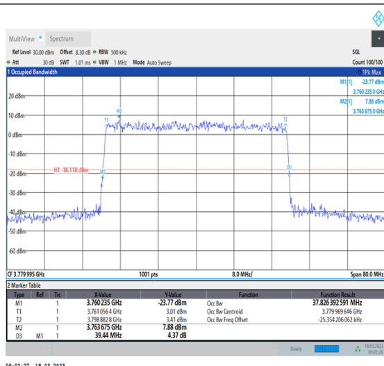
1-N78-3700-3800-30-40-H-9-CP-256QAM-Outer_Full-106@0-Ant0-37.826-39.440-≤40-PASS
