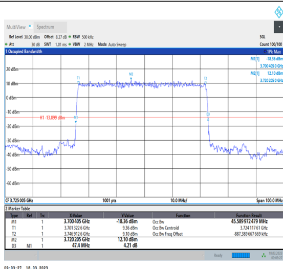
1-N78-3700-3800-30-50-L-2-DFT-PI2BPSK-Outer_Full-128@0-Ant0-45.59-47.400-≤50-PASS
