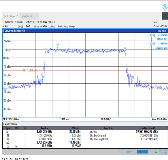
1-N78-3700-3800-30-60-L-3-DFT-16QAM-Outer_Full-162@0-Ant0-8.303-8.760-≤60-PASS
