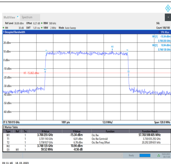
1-N78-3700-3800-30-60-L-1-DFT-QPSK-Outer_Full-162@0-Ant0-57.784-59.520-≤60-PASS
