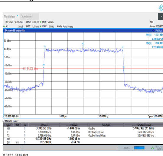
1-N78-3700-3800-30-60-L-2-DFT-PI2BPSK-Outer_Full-162@0-Ant0-57.854-59.520-≤60-PASS
