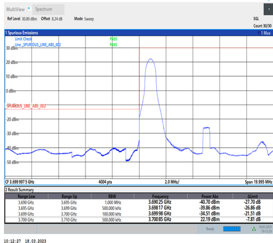
1-N78-3700-3800-30-10-L-1-DFT-PI2BPSK-Edge_1RB_Left-1@0-Ant0-1--PASS-see graph
