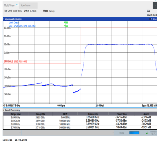
1-N78-3700-3800-30-10-L-3-DFT-PI2BPSK-Outer_Full-24@0-Ant0-1--PASS-see graph
