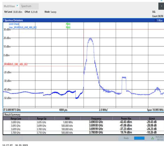
1-N78-3700-3800-30-10-L-4-CP-QPSK-Edge_1RB_Left-1@0-Ant0-1--PASS-see graph
