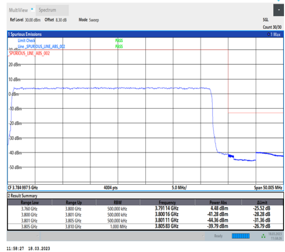
1-N78-3700-3800-30-40-H-3-DFT-PI2BPSK-Outer_Full-100@0-Ant0-1--PASS-see graph
