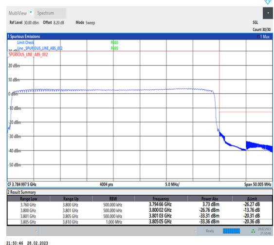
1-N78-3700-3800-30-40-H-6-CP-QPSK-Outer_Full-106@0-Ant0-1--PASS-see graph
