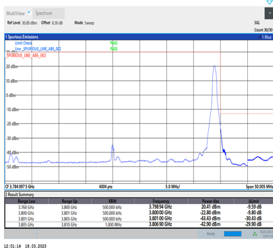
1-N78-3700-3800-30-40-H-5-CP-QPSK-Edge_1RB_Right-1@105-Ant0-1--PASS-see graph
