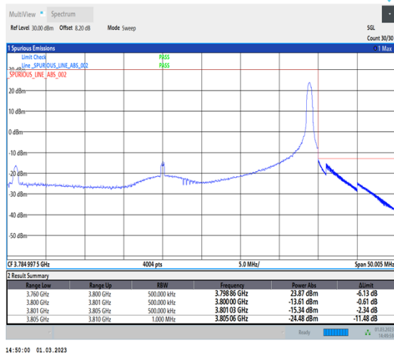
1-N78-3700-3800-30-40-H-2-DFT-PI2BPSK-Edge_1RB_Right-1@105-Ant0-1--PASS-see graph
