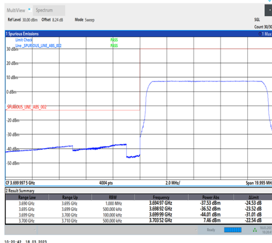
1-N78-3700-3800-30-10-L-6-CP-QPSK-Outer_Full-24@0-Ant0-1--PASS-see graph
