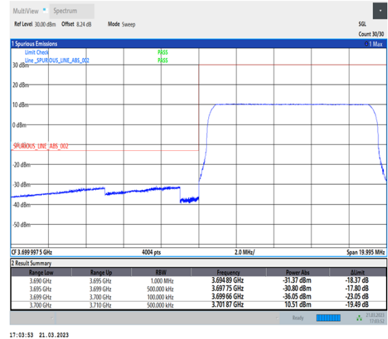
1-N78-3700-3800-30-10-L-6-CP-QPSK-Outer_Full-24@0-Ant0-1--PASS-see graph
