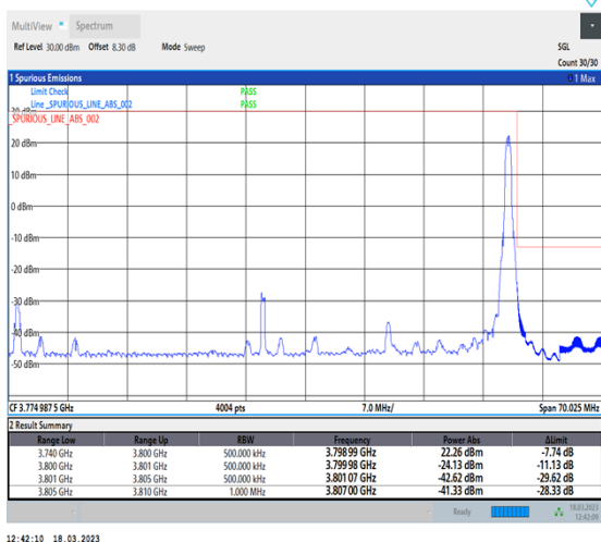
1-N78-3700-3800-30-60-H-2-DFT-PI2BPSK-Edge_1RB_Right-1@161-Ant0-1--PASS-see graph
