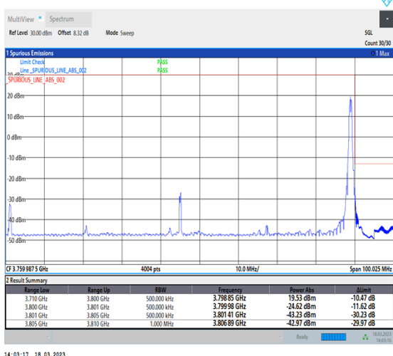
1-N78-3700-3800-30-90-H-5-CP-QPSK-Edge_1RB_Right-1@244-Ant0-1--PASS-see graph
