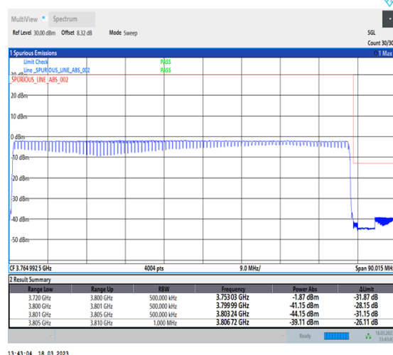
1-N78-3700-3800-30-80-H-6-CP-QPSK-Outer_Full-217@0-Ant0-1--PASS-see graph
