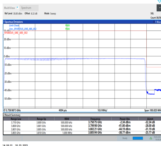
1-N78-3700-3800-30-90-H-6-CP-QPSK-Outer_Full-245@0-Ant0-1--PASS-see graph
