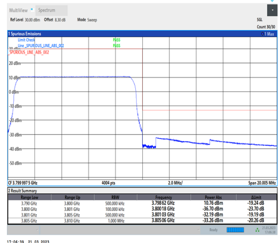
1-N78-3700-3800-30-10-H-6-CP-QPSK-Outer_Full-24@0-Ant0-1--PASS-see graph
