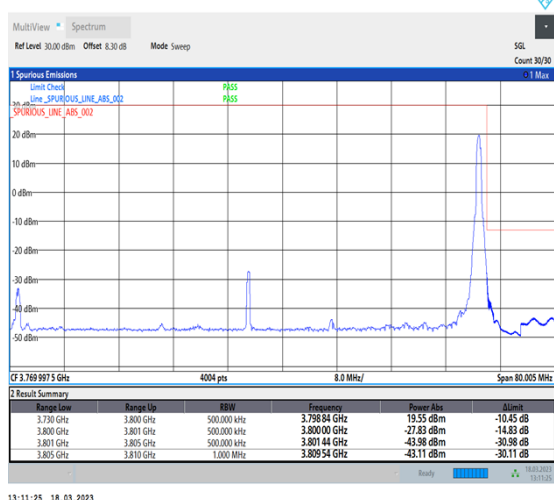
1-N78-3700-3800-30-70-H-5-CP-QPSK-Edge_1RB_Right-1@188-Ant0-1--PASS-see graph
