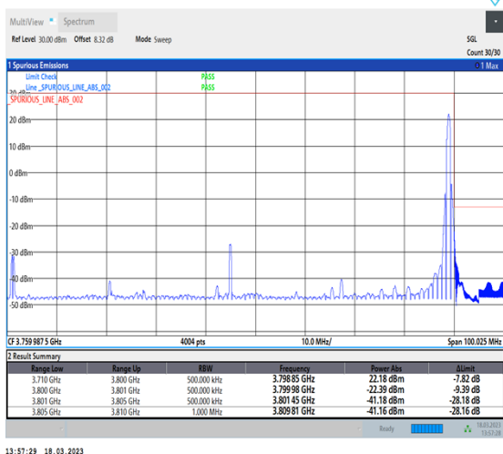
1-N78-3700-3800-30-90-H-2-DFT-PI2BPSK-Edge_1RB_Right-1@244-Ant0-1--PASS-see graph
