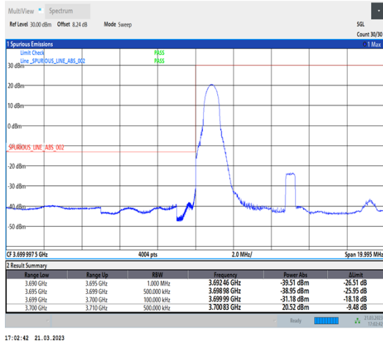
1-N78-3700-3800-30-10-L-4-CP-QPSK-Edge_1RB_Left-1@0-Ant0-1--PASS-see graph
