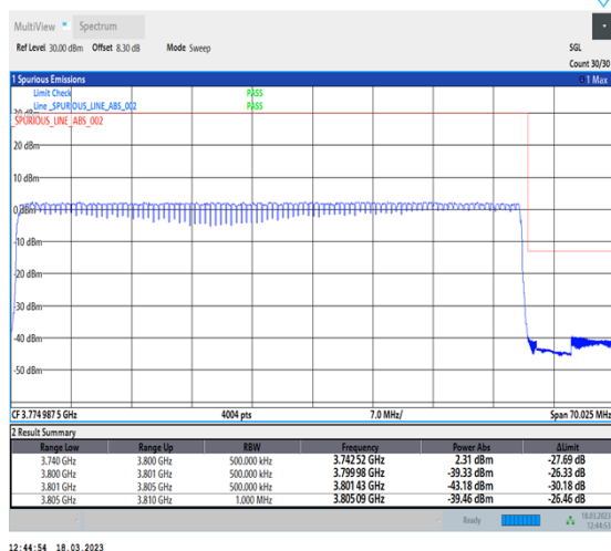
1-N78-3700-3800-30-60-H-3-DFT-PI2BPSK-Outer_Full-162@0-Ant0-1--PASS-see graph
