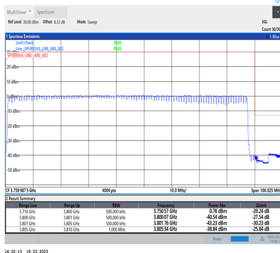
1-N78-3700-3800-30-90-H-3-DFT-PI2BPSK-Outer_Full-240@0-Ant0-1--PASS-see graph
