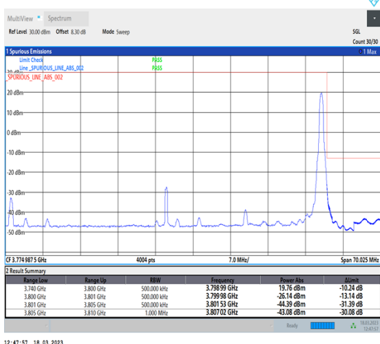
1-N78-3700-3800-30-60-H-5-CP-QPSK-Edge_1RB_Right-1@161-Ant0-1--PASS-see graph
