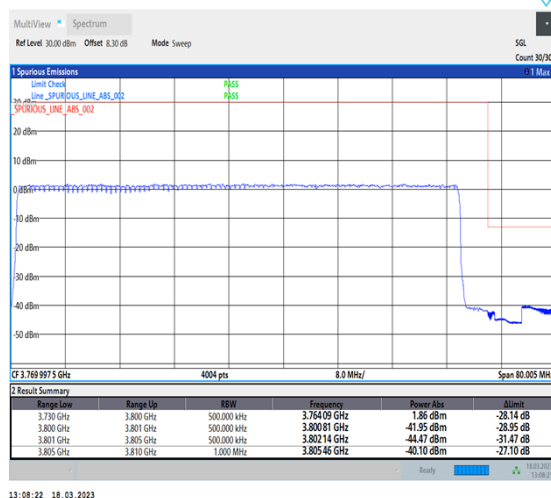
1-N78-3700-3800-30-70-H-3-DFT-PI2BPSK-Outer_Full-180@0-Ant0-1--PASS-see graph
