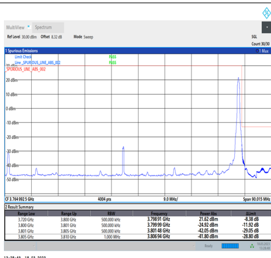
1-N78-3700-3800-30-80-H-2-DFT-PI2BPSK-Edge_1RB_Right-1@216-Ant0-1--PASS-see graph
