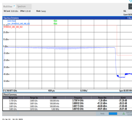
1-N78-3700-3800-30-70-H-6-CP-QPSK-Outer_Full-189@0-Ant0-1--PASS-see graph
