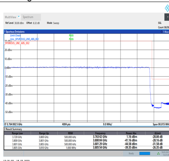
1-N78-3700-3800-30-80-H-3-DFT-PI2BPSK-Outer_Full-216@0-Ant0-1--PASS-see graph
