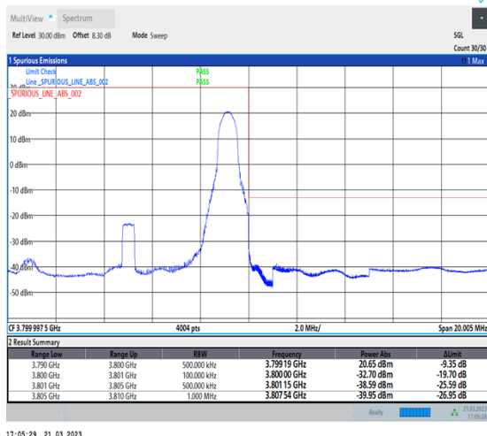
1-N78-3700-3800-30-10-H-5-CP-QPSK-Edge_1RB_Right-1@23-Ant0-1--PASS-see graph
