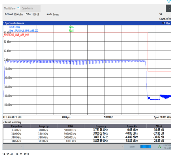
1-N78-3700-3800-30-60-H-6-CP-QPSK-Outer_Full-162@0-Ant0-1--PASS-see graph
