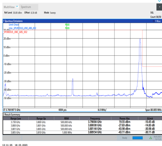
1-N78-3700-3800-30-70-H-2-DFT-PI2BPSK-Edge_1RB_Right-1@188-Ant0-1--PASS-see graph
