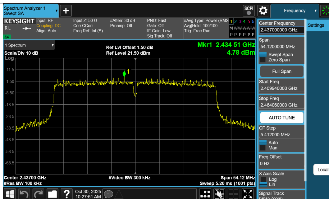
11N40SISO-Ant1-2437-PASS
