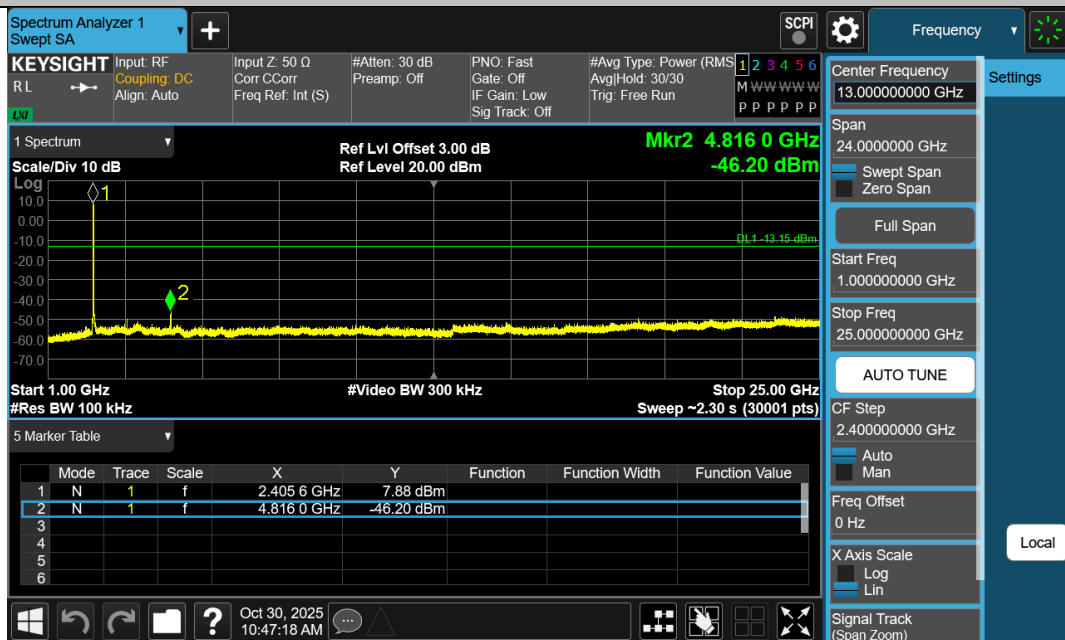
11N20SISO-Ant1-2412-1000~25000-PASS
