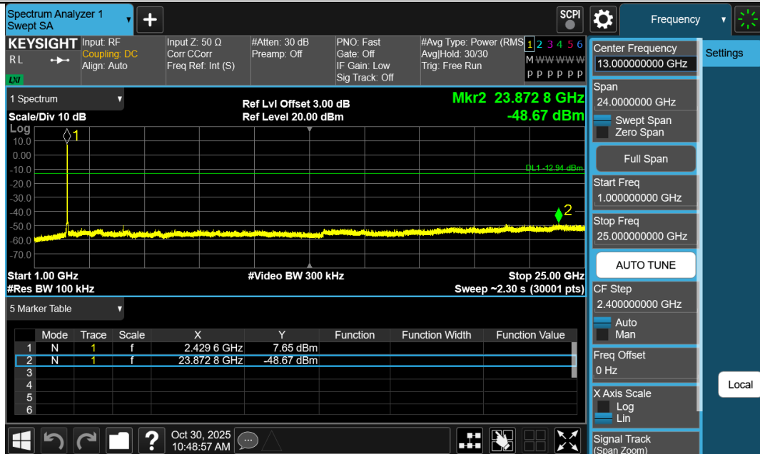
11N20SISO-Ant1-2437-1000~25000-PASS
