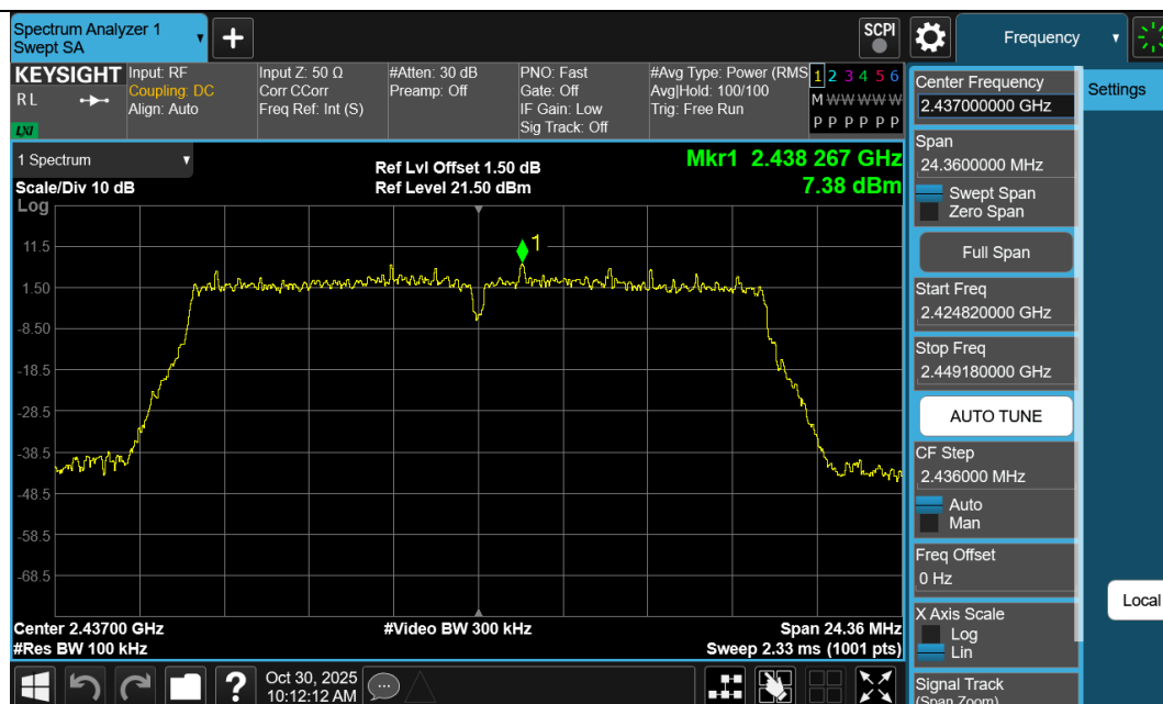
11G-Ant1-2437-PASS
