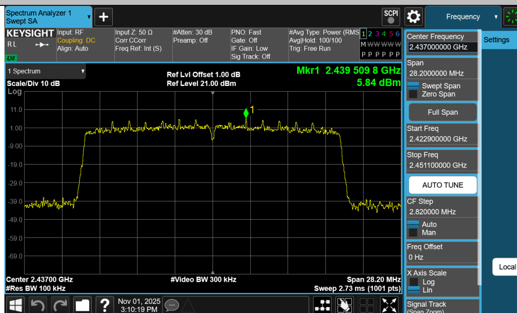
11BE20SISO-Ant1-2437-PASS
