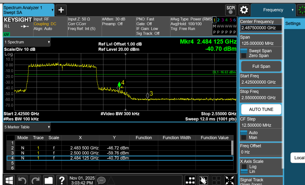
11AX40SISO-Ant1-2452-PASS
