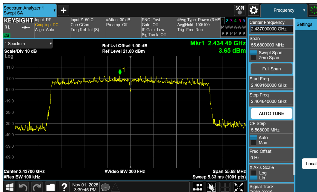
11BE40SISO-Ant1-2437-PASS
