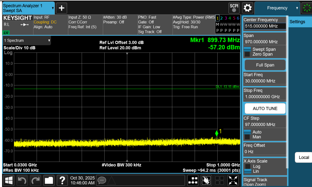
11N20SISO-Ant1-2412-30~1000-PASS
