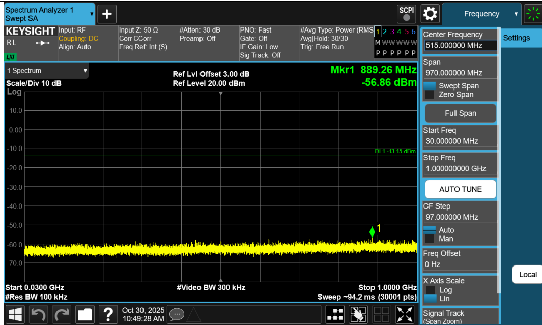
11N20SISO-Ant1-2462-30~1000-PASS
