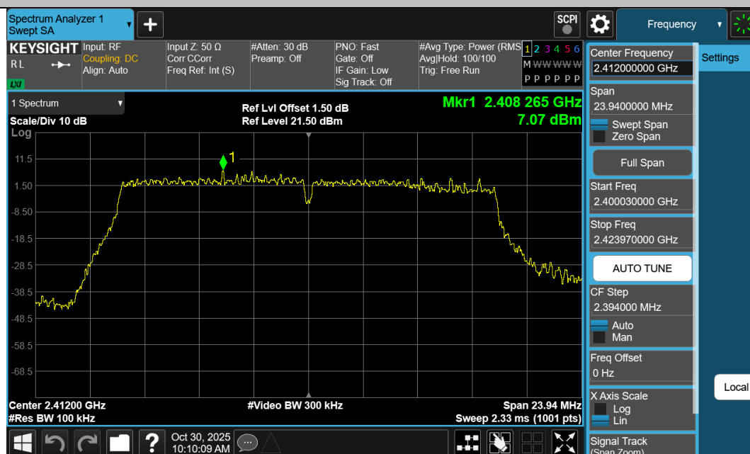
11G-Ant1-2412-PASS
