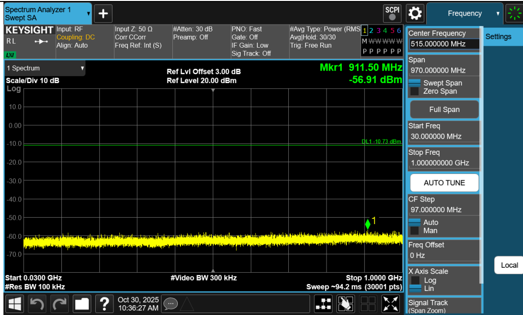
11B-Ant1-2462-30~1000-PASS
