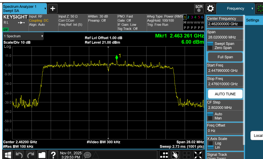
11BE20SISO-Ant1-2462-PASS
