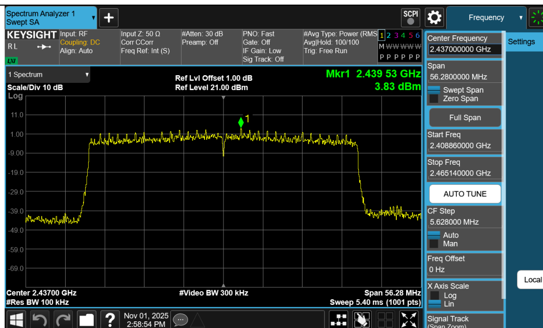
11AX40SISO-Ant1-2437-PASS
