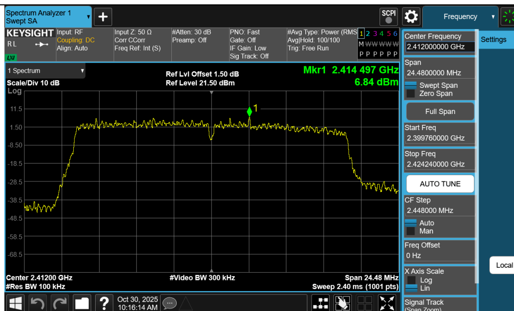
11N20SISO-Ant1-2412-PASS
