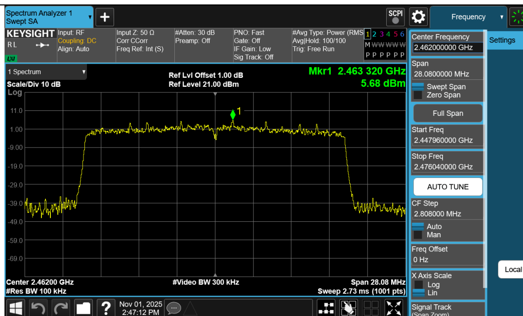
11AX20SISO-Ant1-2462-PASS
