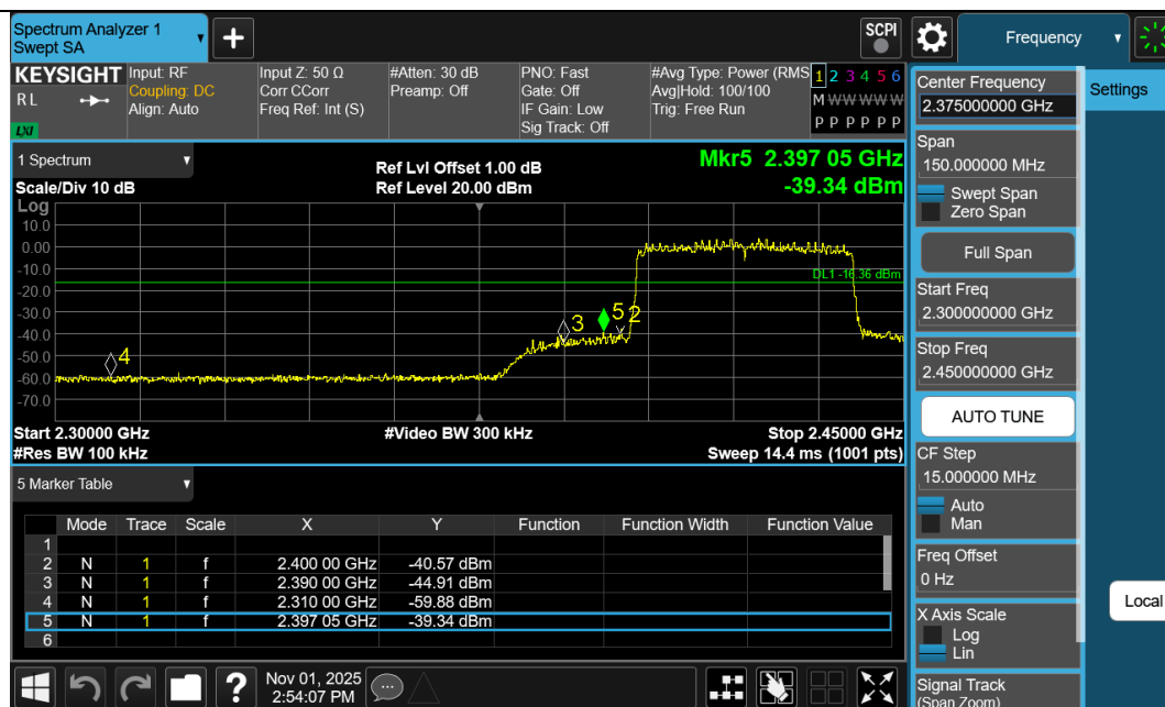
11AX40SISO-Ant1-2422-PASS
