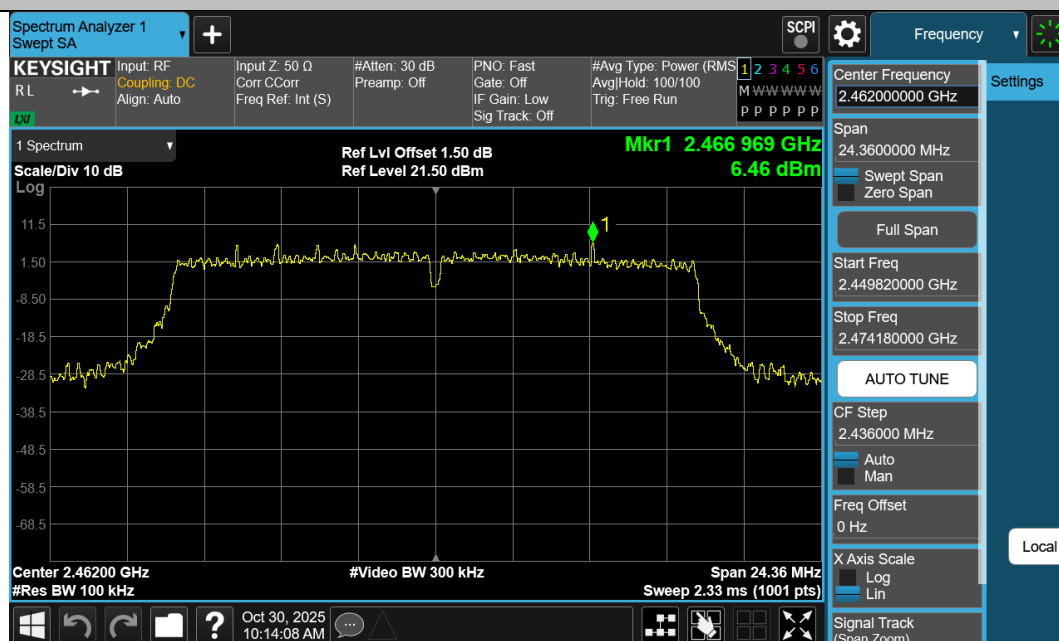
11G-Ant1-2462-PASS
