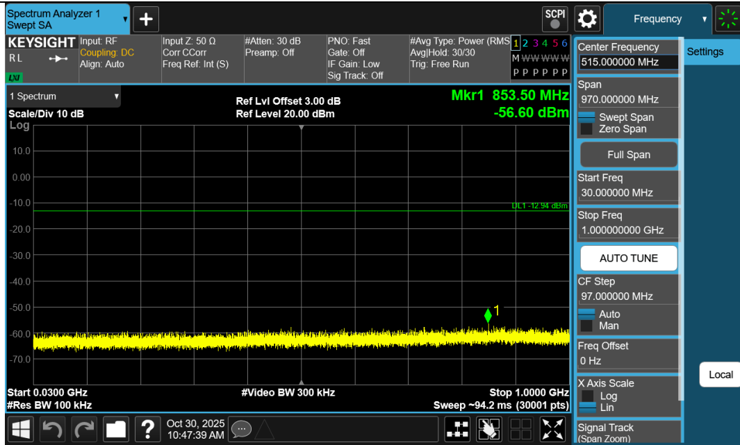
11N20SISO-Ant1-2437-30~1000-PASS
