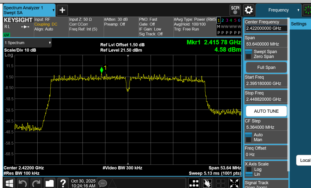
11N40SISO-Ant1-2422-PASS
