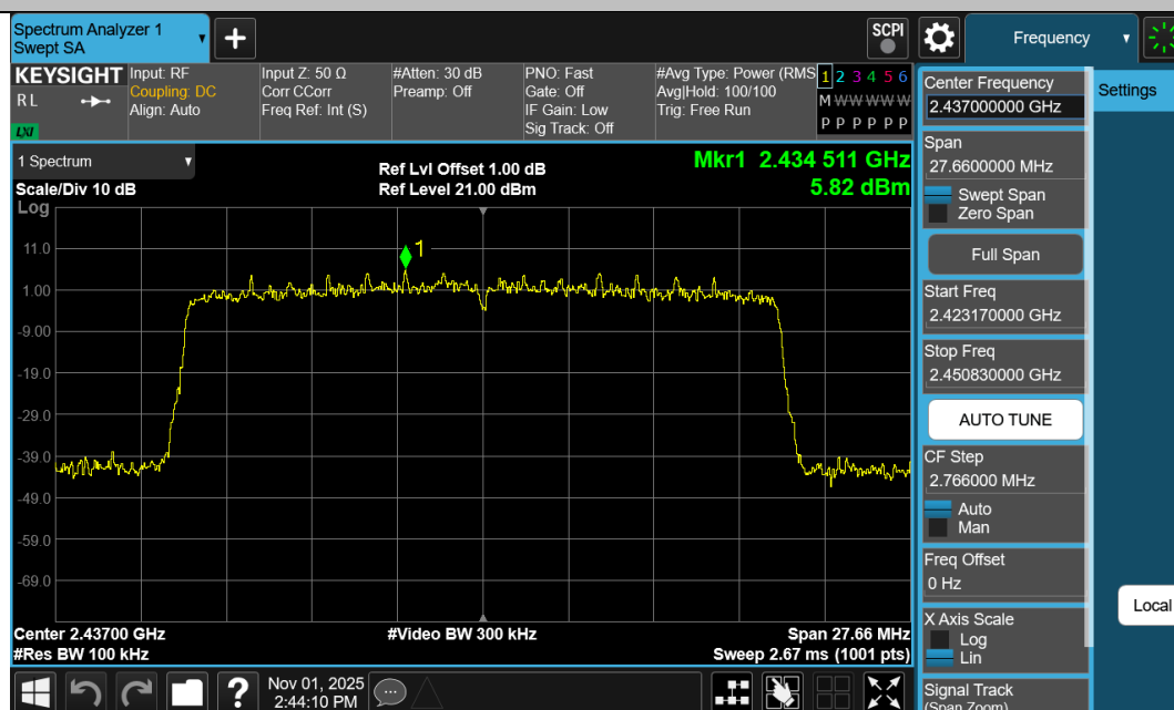
11AX20SISO-Ant1-2437-PASS
