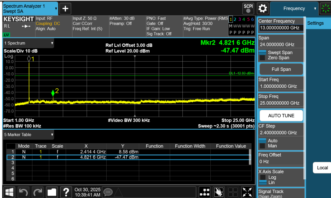
11G-Ant1-2412-1000~25000-PASS
