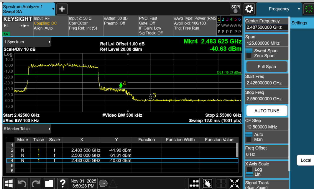
11BE40SISO-Ant1-2452-PASS
