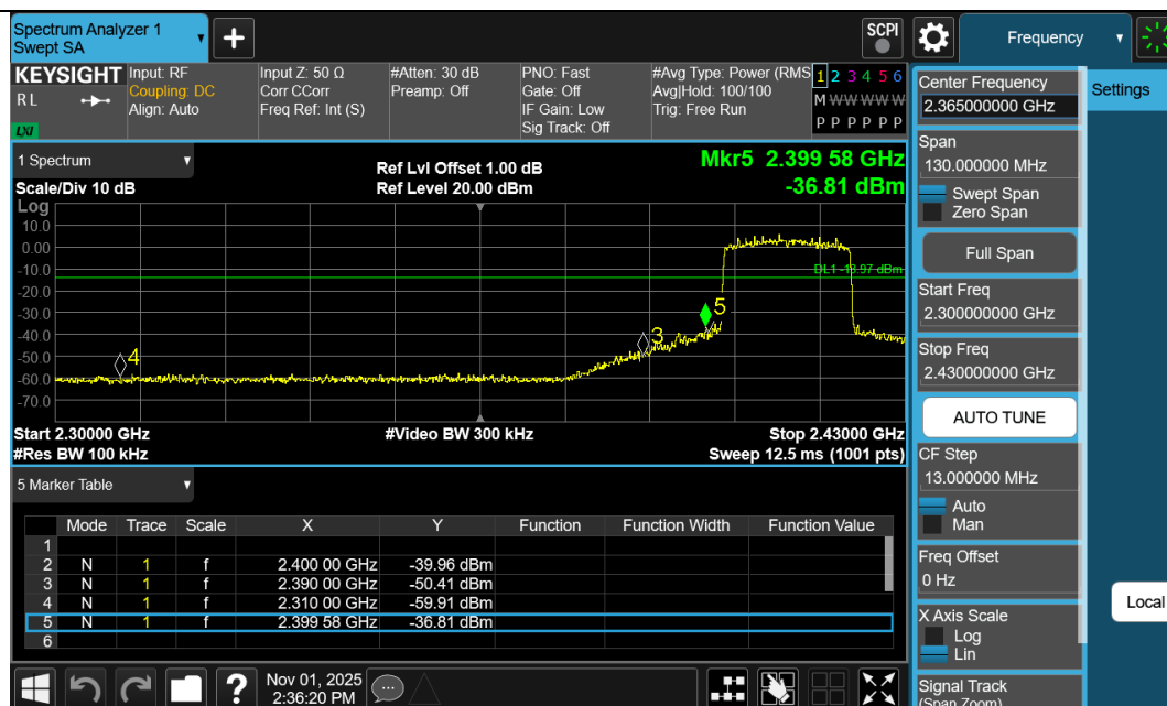
11AX20SISO-Ant1-2412-PASS
