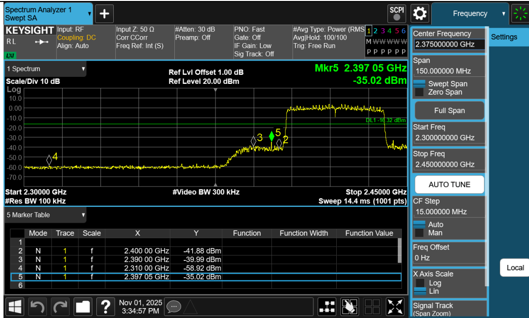
11BE40SISO-Ant1-2422-PASS
