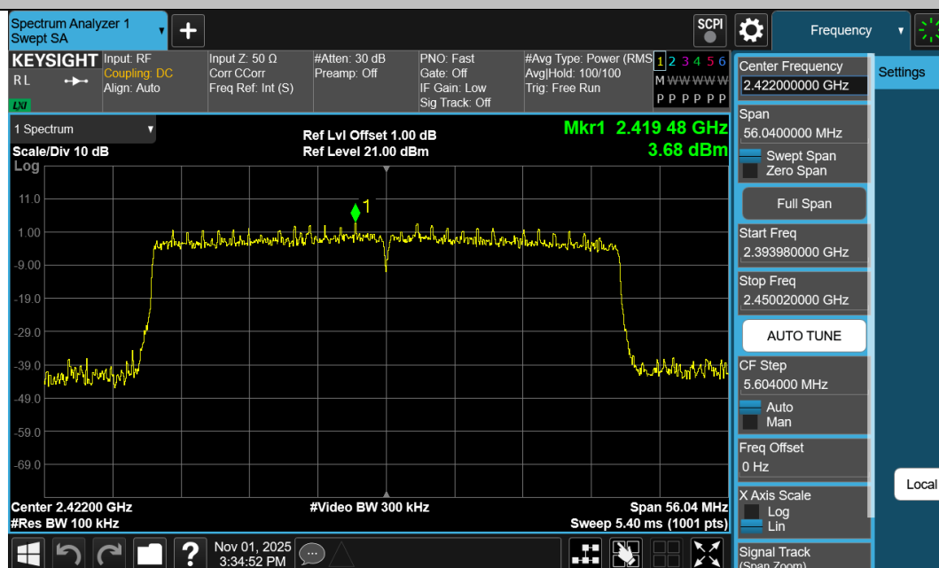
11BE40SISO-Ant1-2422-PASS
