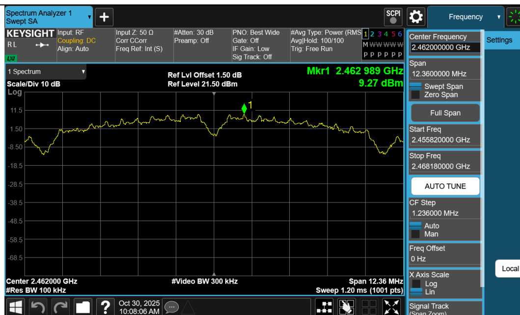
11B-Ant1-2462-PASS
