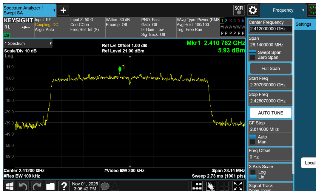
11BE20SISO-Ant1-2412-PASS
