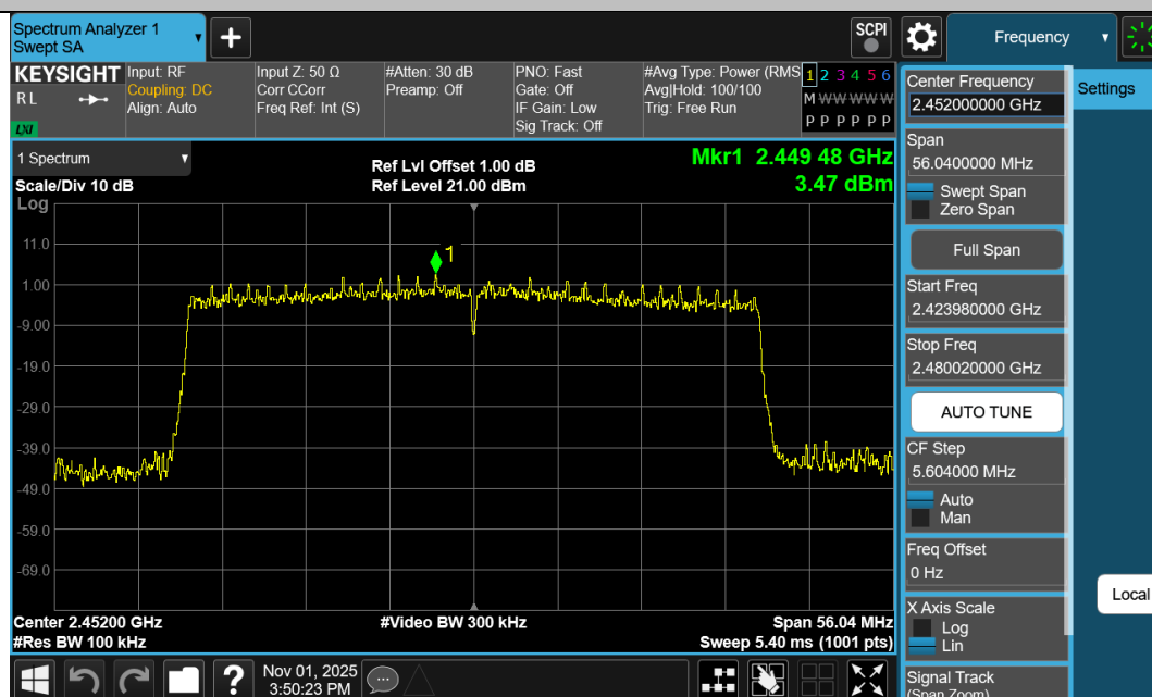
11BE40SISO-Ant1-2452-PASS
