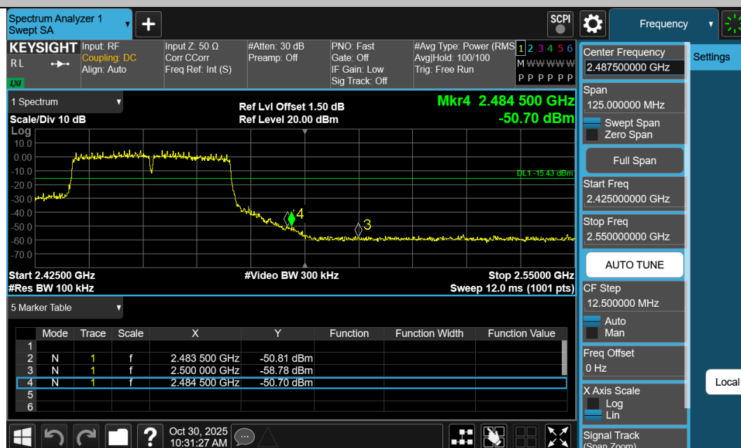
11N40SISO-Ant1-2452-PASS
