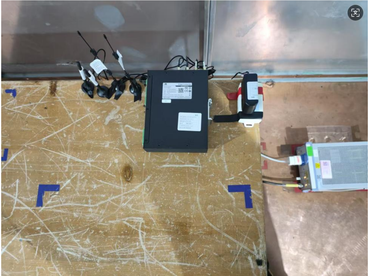
Power line conducted emission setup photo
