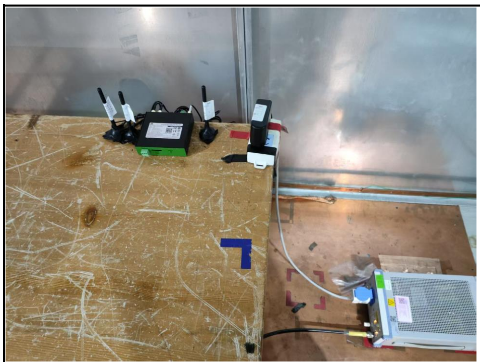
Power line conducted emission setup photo
