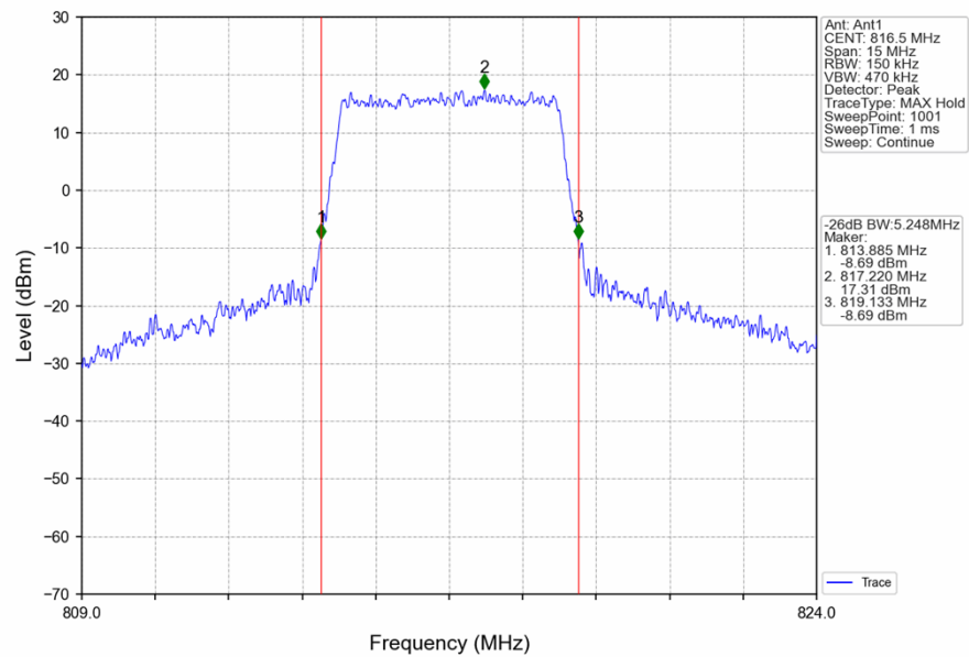
Band26a_5MHz_16QAM_LCH_816.5MHz_RB_25_0_NTNV
