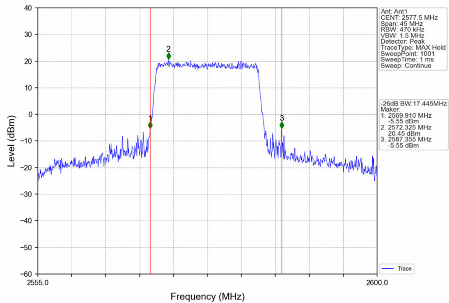
Band38_15MHz_16QAM_LCH_2577.5MHz_RB_75_0_NTNV
