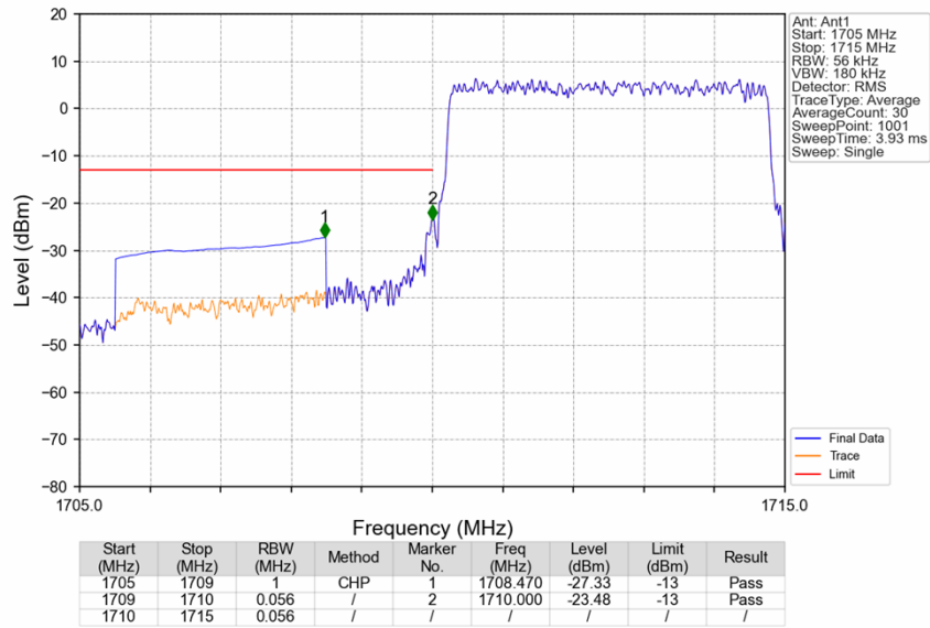
Band4_5MHz_QPSK_LCH_1712.5MHz_RB_25_0_NTNV
