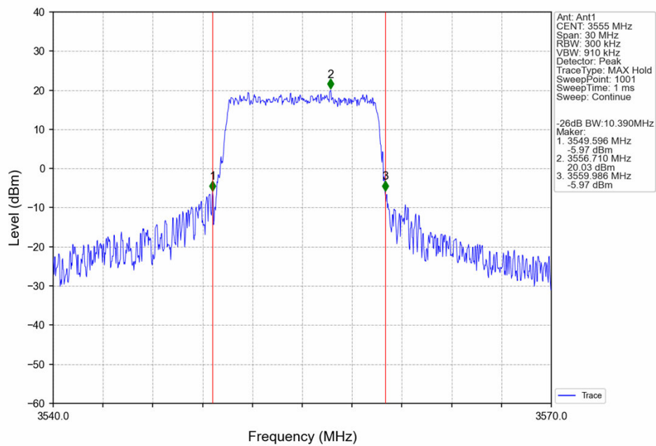
Band42c_10MHz_16QAM_LCH_3555MHz_RB_50_0_NTNV
