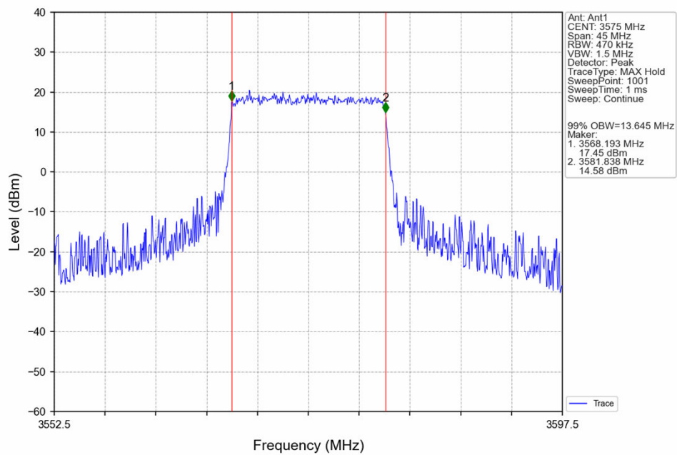
Band42c_15MHz_QPSK_MCH_3575MHz_RB_75_0_NTNV
