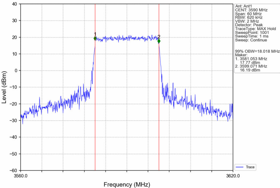
Band42c_20MHz_16QAM_HCH_3590MHz_RB_100_0_NTNV
