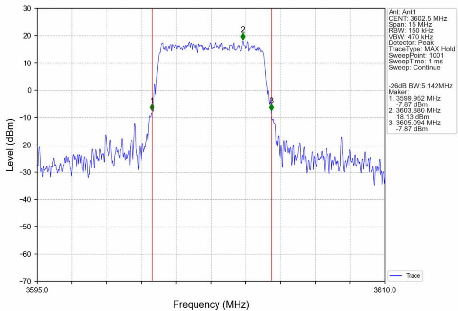
Band43c_5MHz_16QAM_LCH_3602.5MHz_RB_25_0_NTNV
