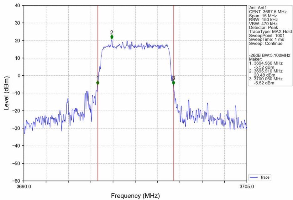
Band43c_5MHz_16QAM_HCH_3697.5MHz_RB_25_0_NTNV
