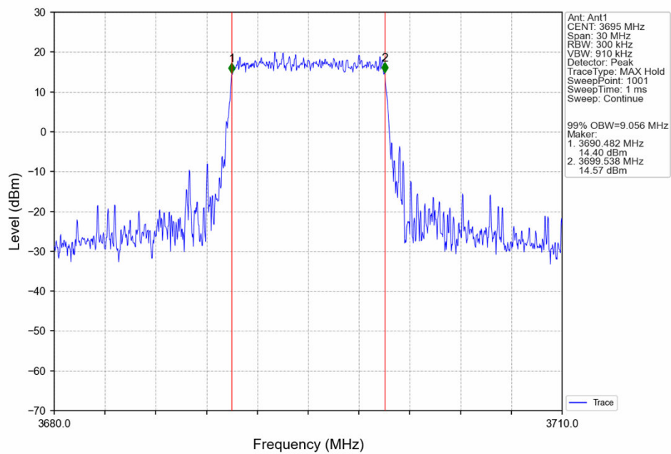
Band43c_10MHz_16QAM_HCH_3695MHz_RB_50_0_NTNV
