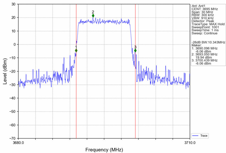
Band43c_10MHz_16QAM_HCH_3695MHz_RB_50_0_NTNV
