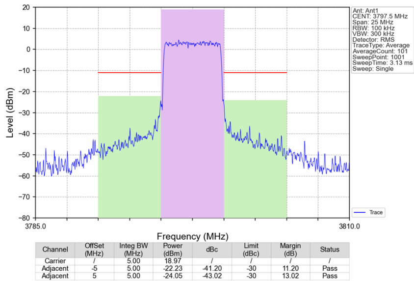
Band43d_5MHz_16QAM_HCH_3797.5MHz_RB_25_0_NTNV
