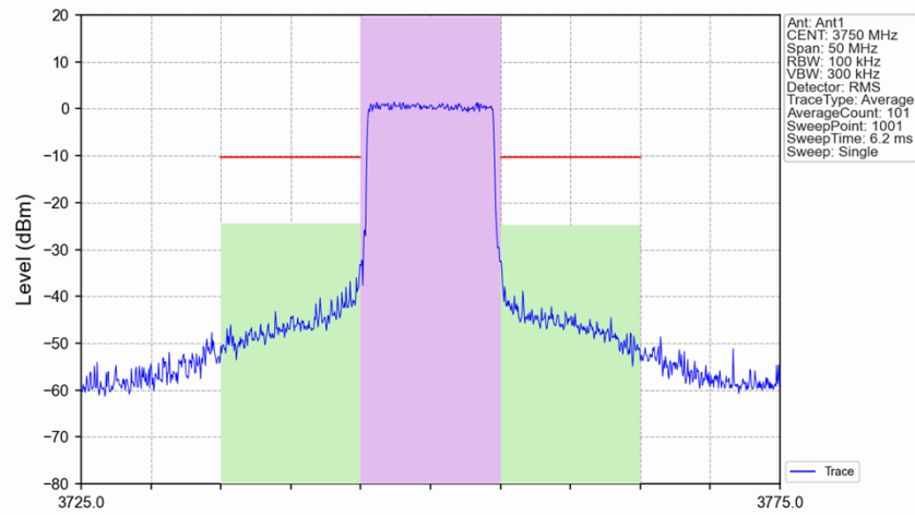
Band43d_10MHz_16QAM_MCH_3750MHz_RB_50_0_NTNV
