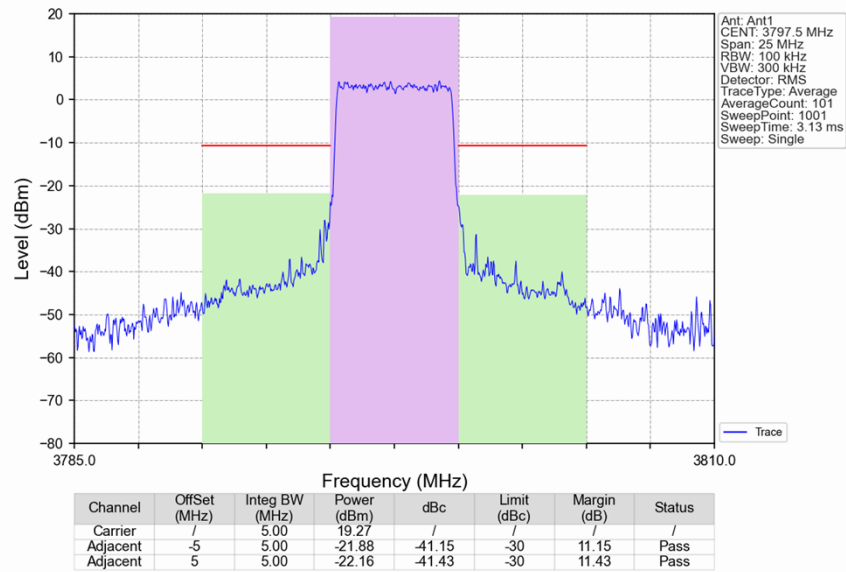
Band43d_5MHz_QPSK_HCH_3797.5MHz_RB_25_0_NTNV
