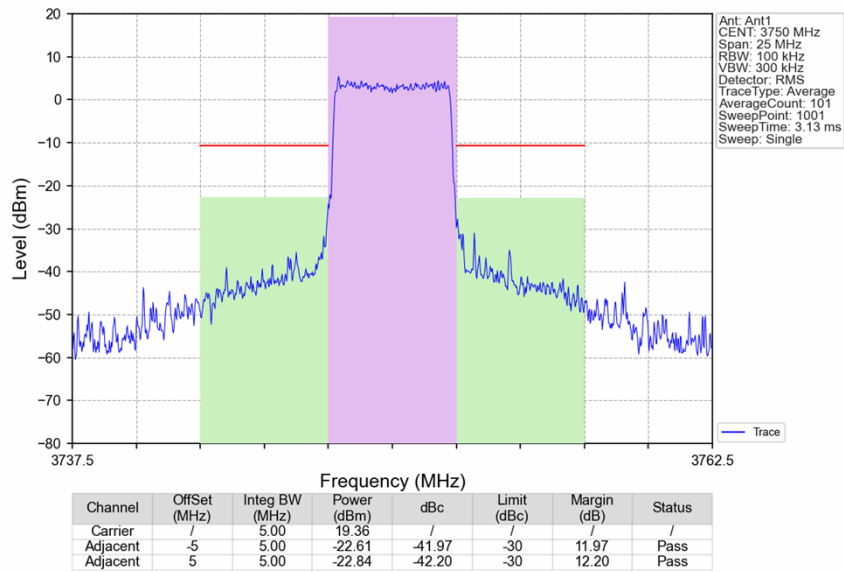
Band43d_5MHz_16QAM_MCH_3750MHz_RB_25_0_NTNV
