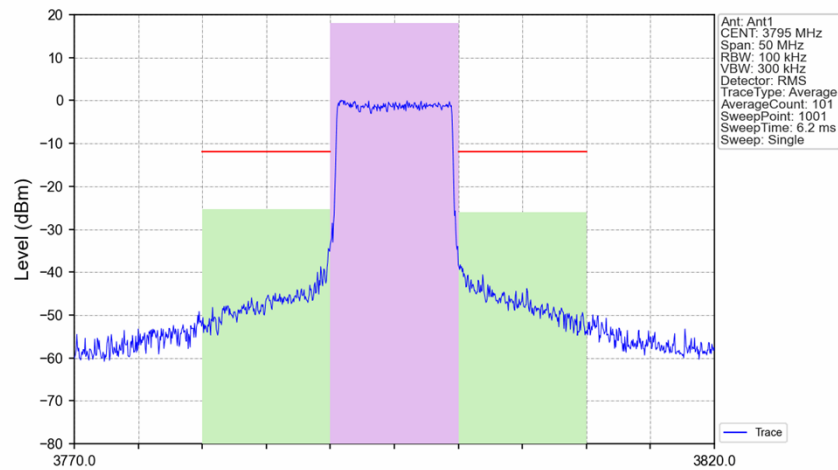
Band43d_10MHz_16QAM_HCH_3795MHz_RB_50_0_NTNV
