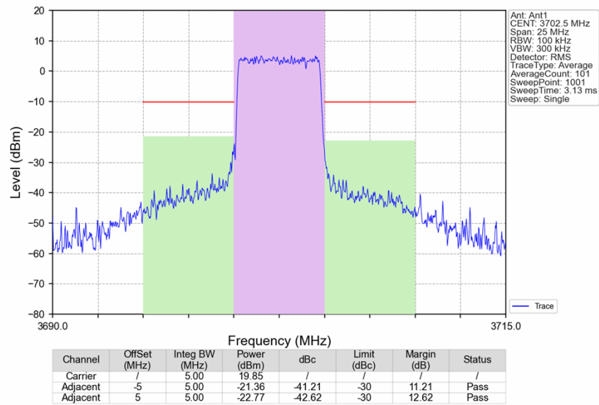
Band43d_5MHz_16QAM_LCH_3702.5MHz_RB_25_0_NTNV
