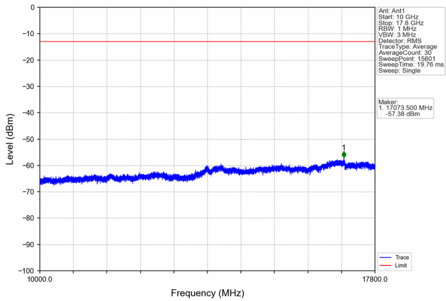
Band66_5MHz_QPSK_LCH_1712.5MHz_RB_25_0_NTNV
