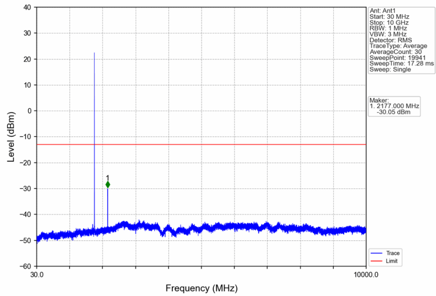
Band66_5MHz_QPSK_HCH_1777.5MHz_RB_1_0_NTNV
