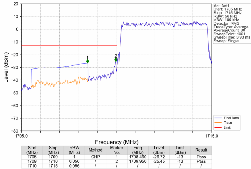
Band66_5MHz_QPSK_LCH_1712.5MHz_RB_25_0_NTNV
