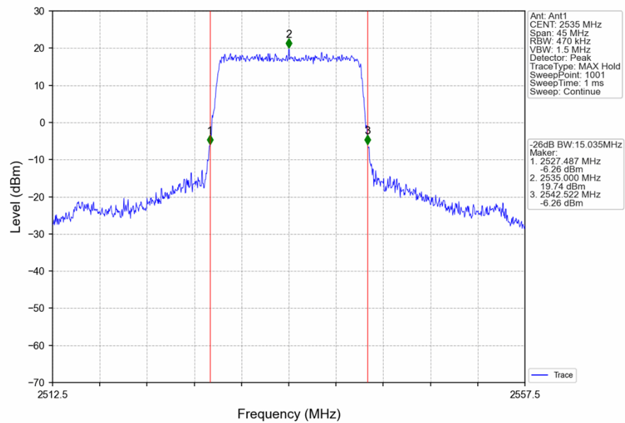
Band7_15MHz_QPSK_MCH_2535MHz_RB_75_0_NTNV
