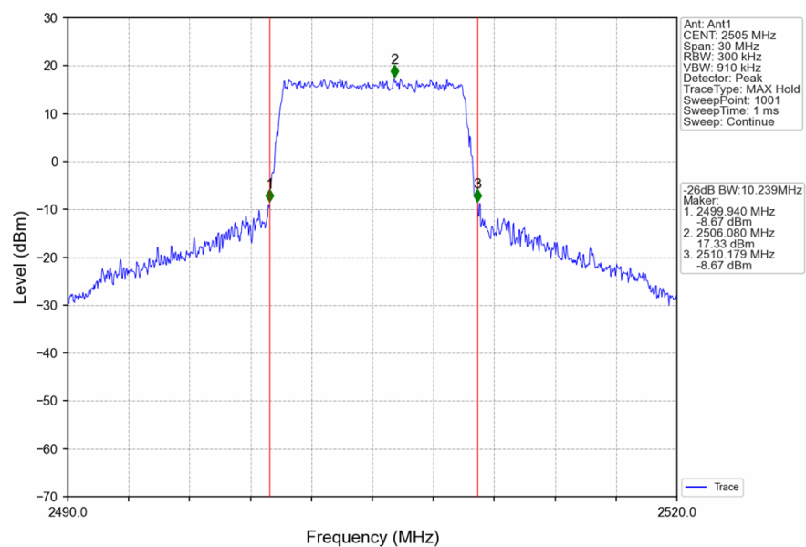
Band7_10MHz_16QAM_LCH_2505MHz_RB_50_0_NTNV
