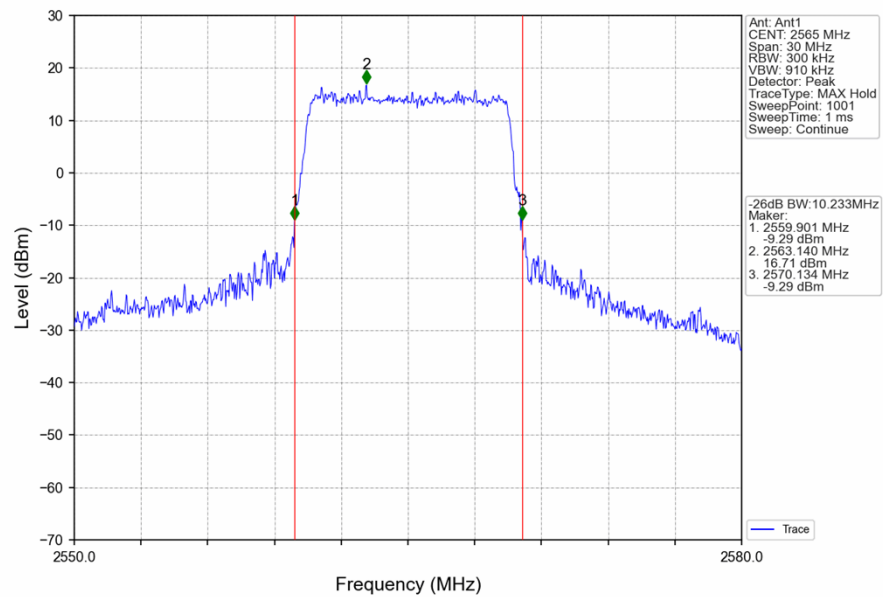
Band7_10MHz_16QAM_HCH_2565MHz_RB_50_0_NTNV
