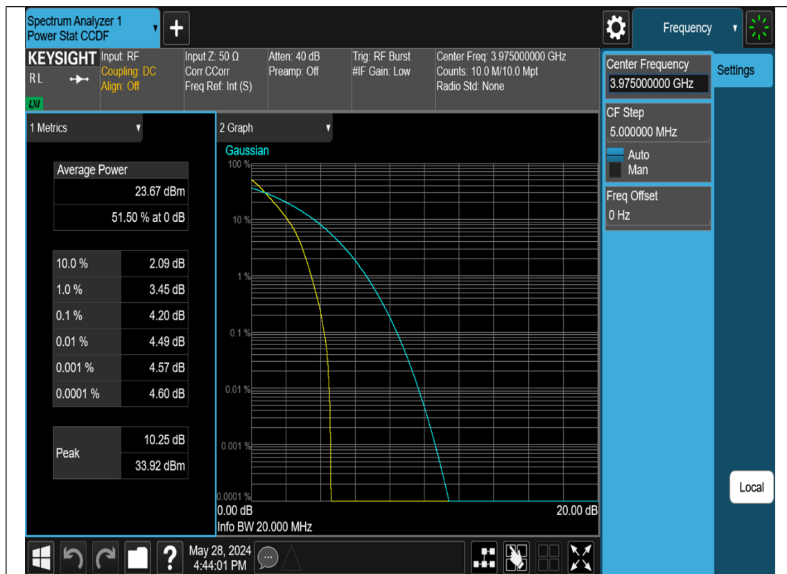
N77b(3700-3980MHz)-10M-PAPR-H-CP-OFDM-QPSK-Outer_Full
