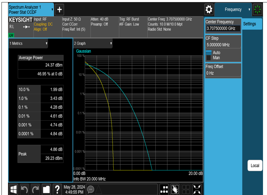
N77b(3700-3980MHz)-15M-PAPR-L-CP-OFDM-QPSK-Outer_Full
