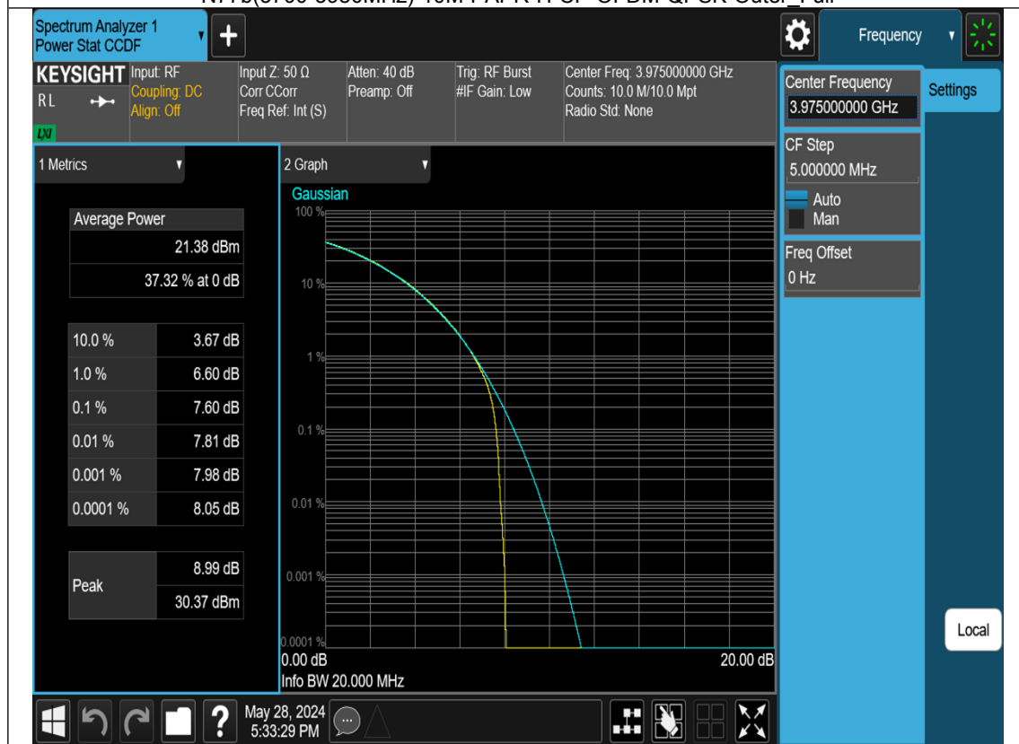
N77b(3700-3980MHz)-15M-PAPR-L-DFT-s-OFDM-Pi2 BPSK-Outer_Full
