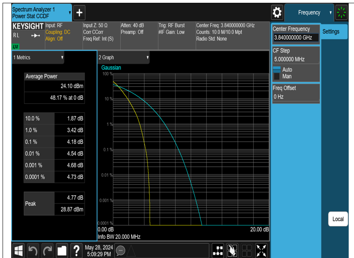
N77b(3700-3980MHz)-20M-PAPR-M-CP-OFDM-QPSK-Outer_Full
