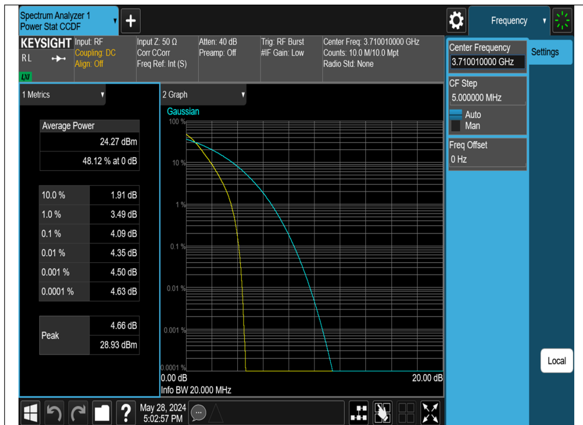
N77b(3700-3980MHz)-20M-PAPR-L-CP-OFDM-QPSK-Outer_Full
