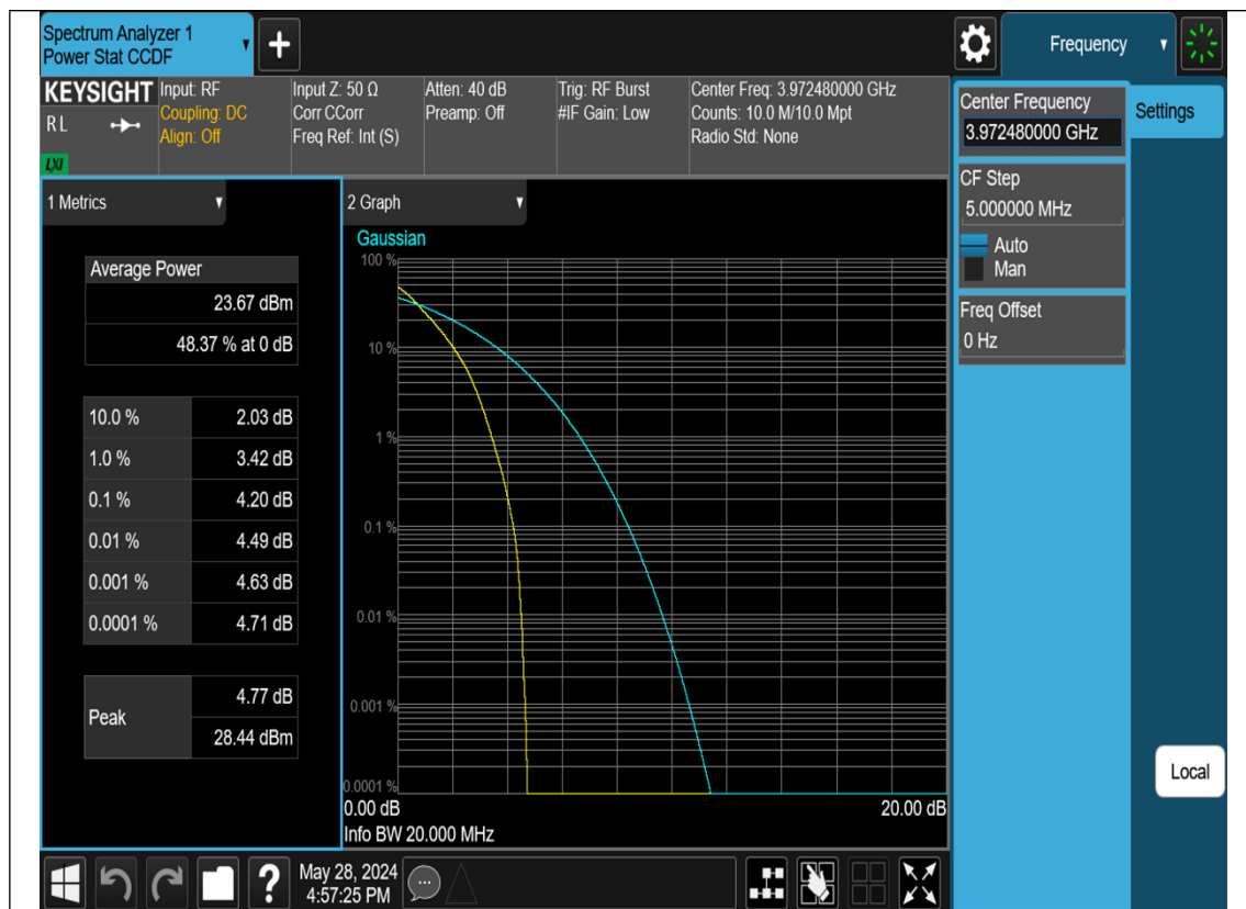
N77b(3700-3980MHz)-15M-PAPR-H-CP-OFDM-QPSK-Outer_Full
