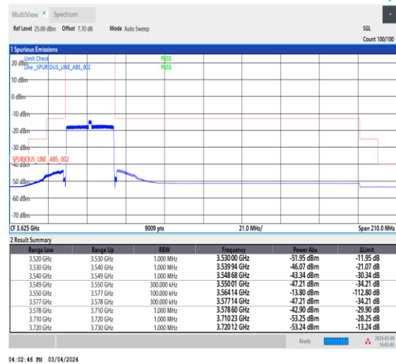
NTNV_CA_n48B_PC3_30+30_15+15_L+L_TID6_1_#1
