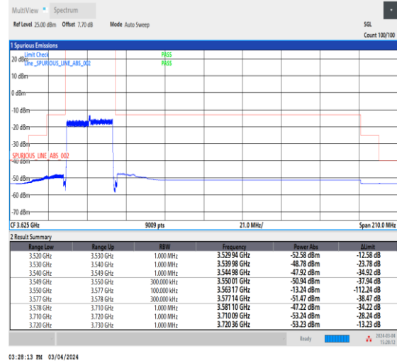
NTNV_CA_n48B_PC3_30+30_15+15_L+L_TID3_1_#1
