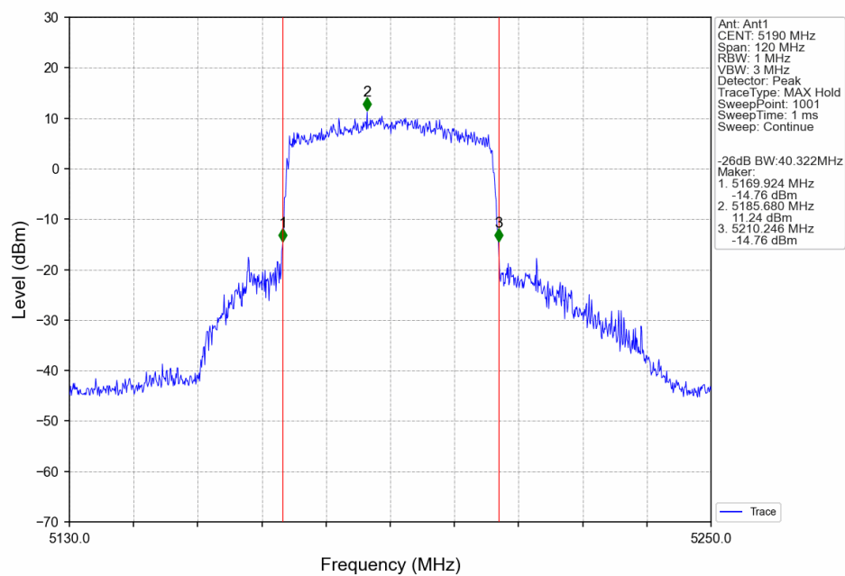
802.11ax(HEW40)_LCH_5190MHz_SU_ / _Ant1_NTNV
