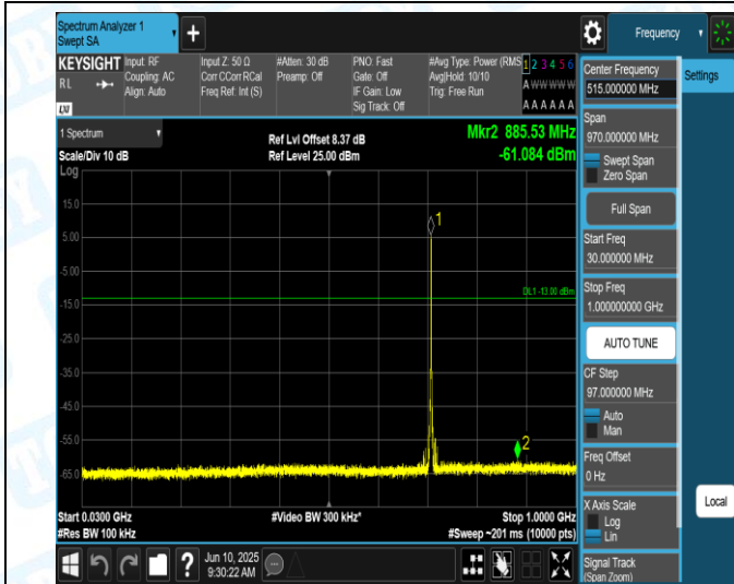
Band 12 - 1.4 MHz - QPSK - 23173 - PASS
