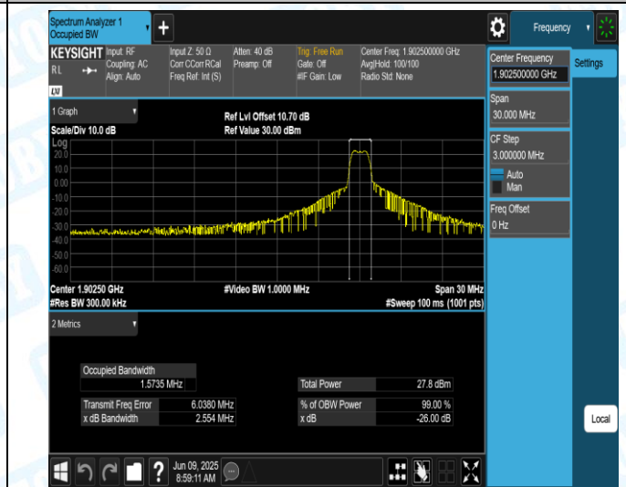
Band 2 - 15 MHz - 16QAM - 19125 - PASS
