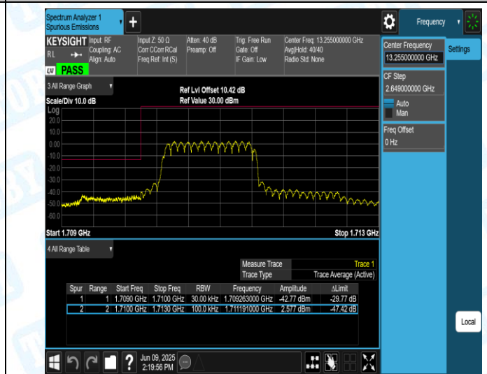
Band 4_3 MHz_16QAM_19965_1_Low
