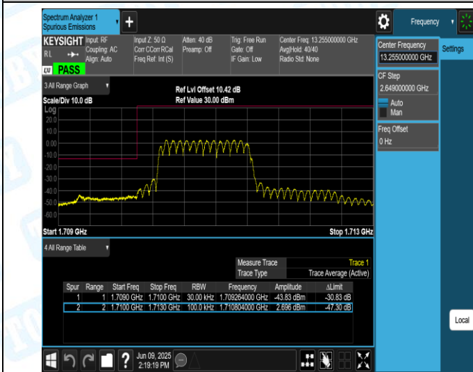
Band 4_3 MHz_QPSK_19965_1_Low
