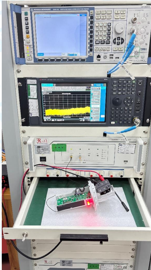
Photo of Setup for RF Conducted
