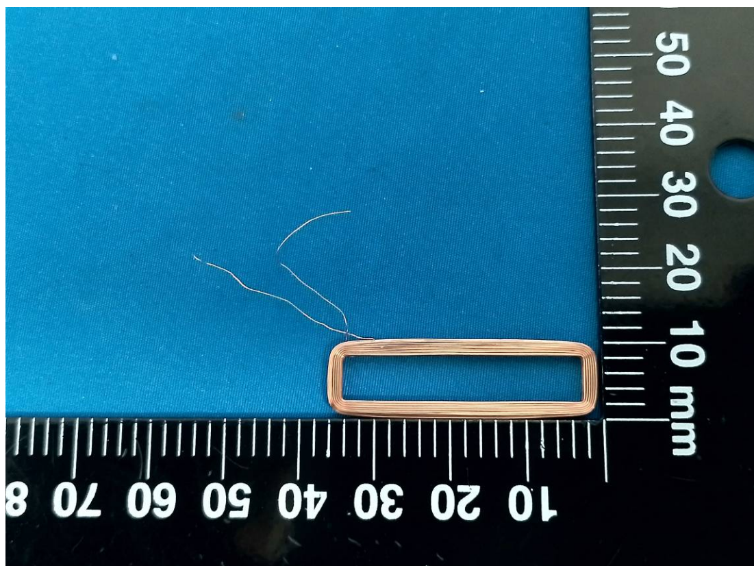
RFID_125kHz Antenna
