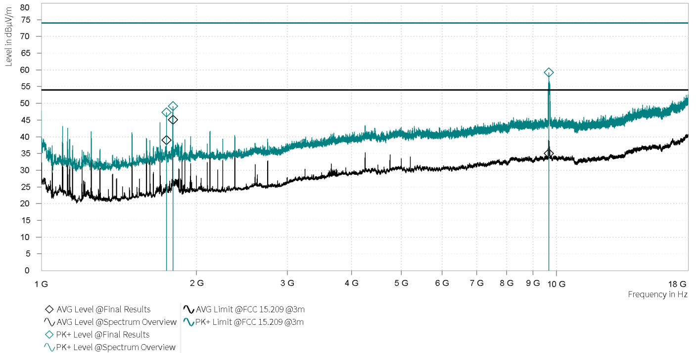
Plot no. 45: OP 1 - radiated spurious emissions 1 GHz – 18 GHz, hor./vert. polarization
