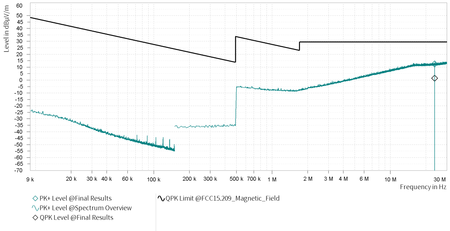
Plot no. 43: OP 1 - radiated spurious emissions 9 kHz – 30 MHz, hor./vert. polarization
