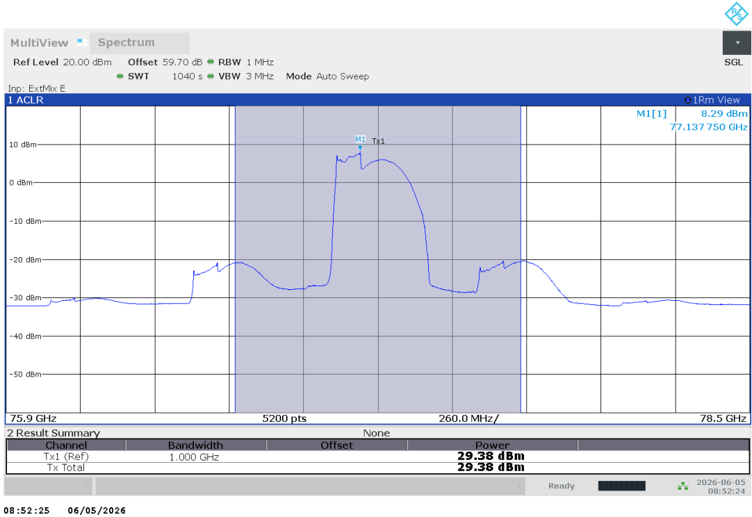
Plot no.1 : OP 1 – Mean Power – RMS detector – 20.0 °C – V nom – RBW = 1 MHz
