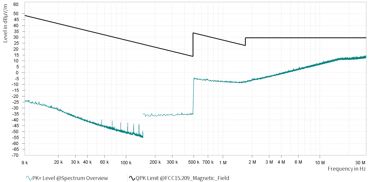
Plot no. 31: OP 1 - radiated spurious emissions 9 kHz – 30 MHz, hor./vert. polarization
