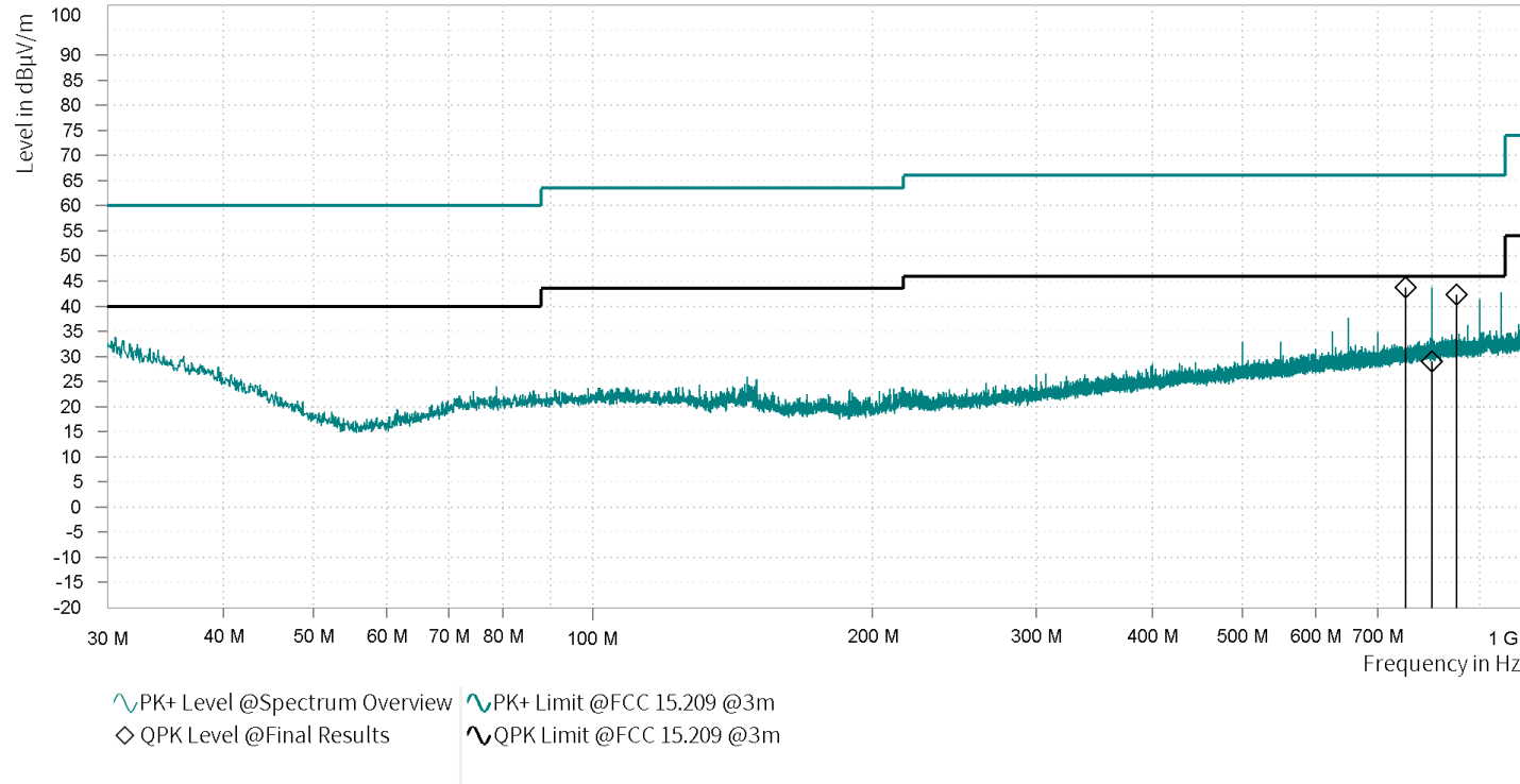
Plot no. 44: OP 1 - radiated spurious emissions 30 MHz – 1 GHz, hor./vert. polarization
