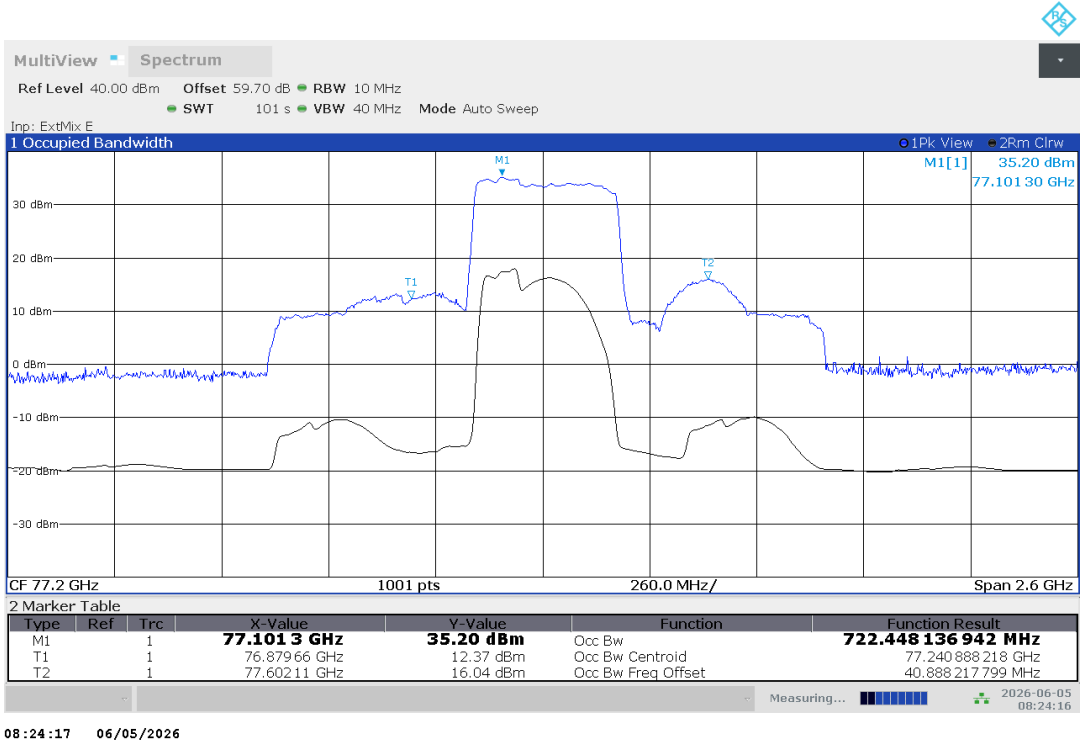
Plot no.8 : OP 1 – OBW – Peak detector – -10.0 °C – V nom – RBW = 10 MHz
