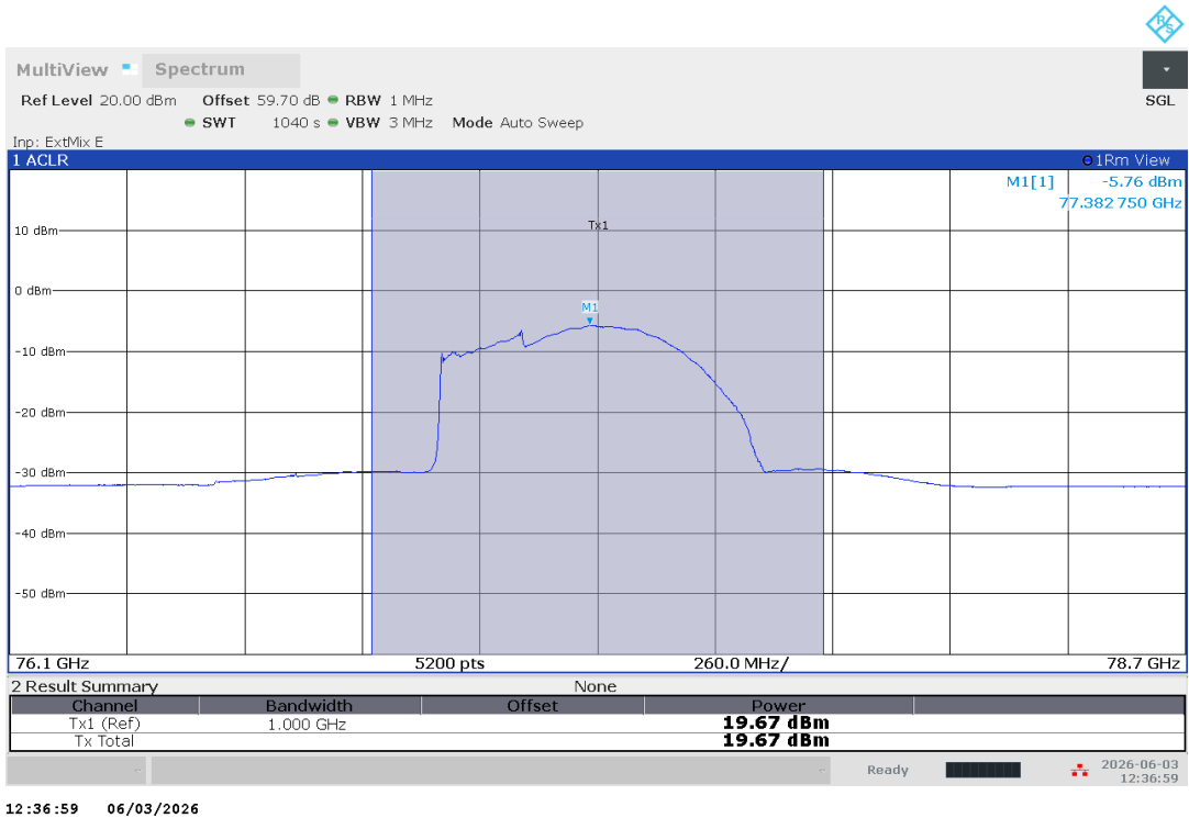
Plot no.2 : OP 2 – Mean Power – RMS detector – 20.0 °C – V nom – RBW = 1 MHz
