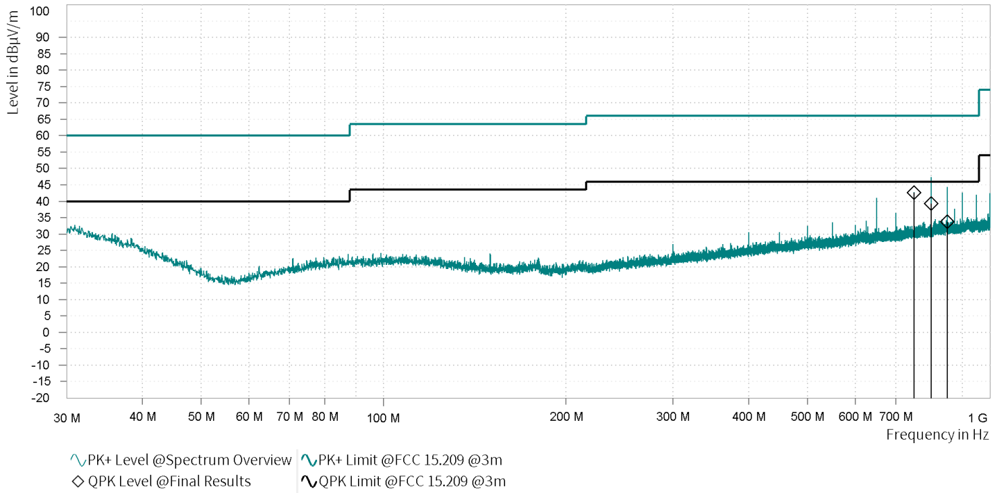
Plot no. 32: OP 1 - radiated spurious emissions 30 MHz – 1 GHz, hor./vert. polarization
