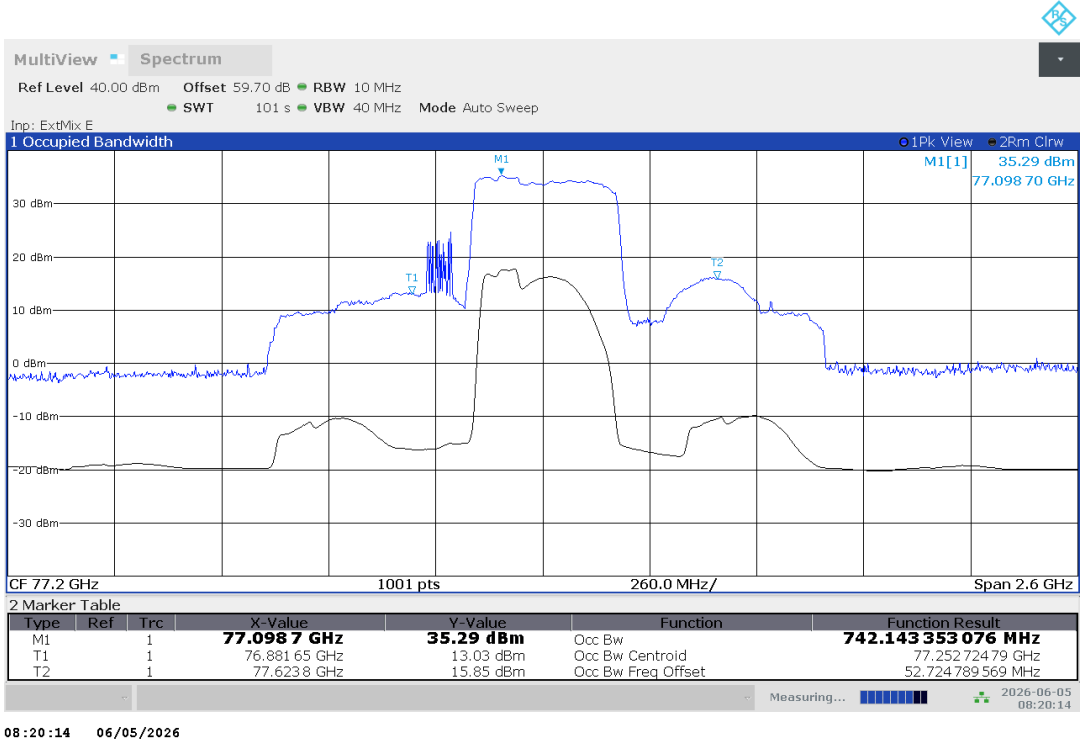
Plot no.7 : OP 1 – OBW – Peak detector – -20.0 °C – V nom – RBW = 10 MHz
