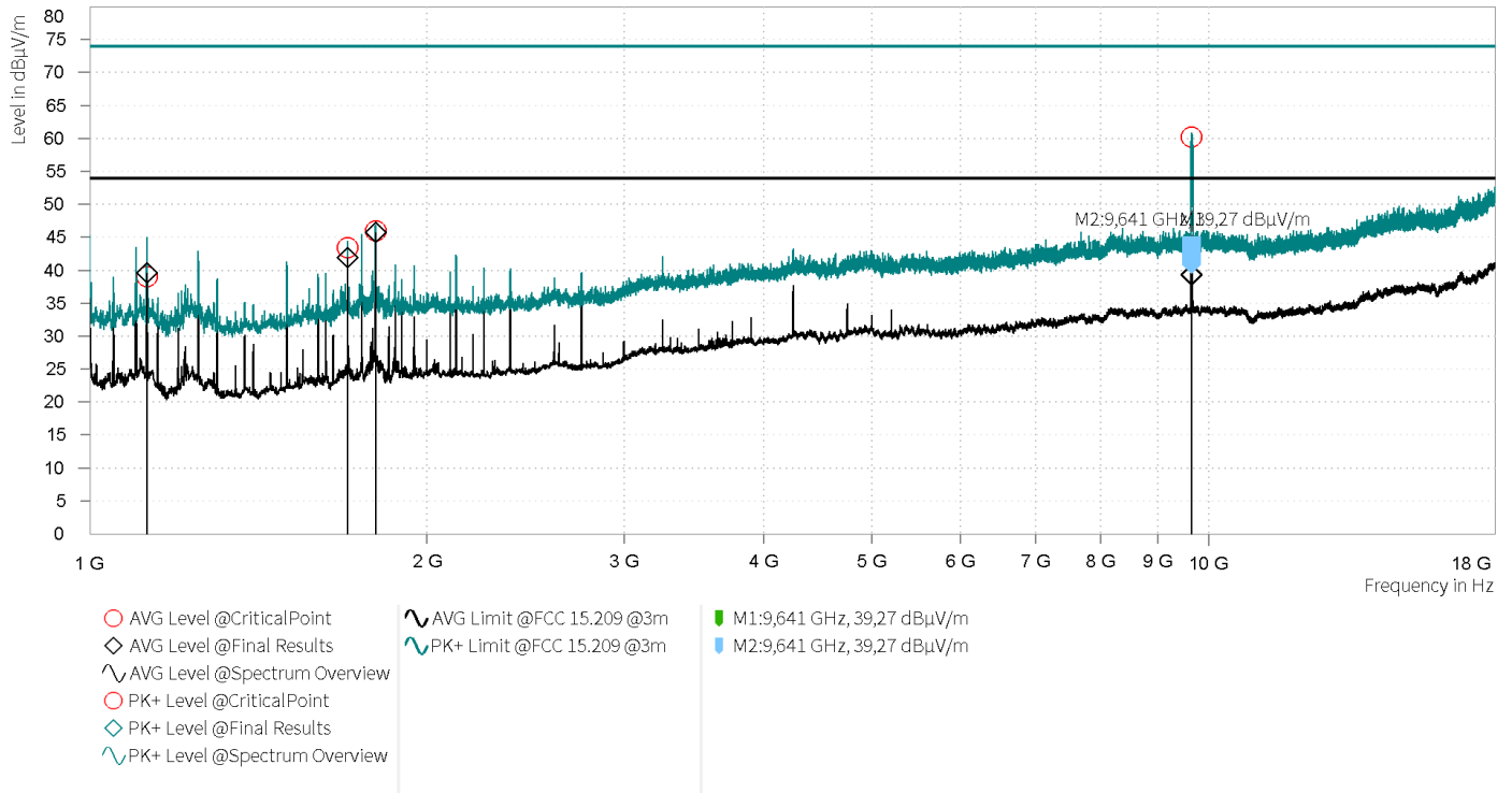
Plot no. 33: OP 1 - radiated spurious emissions 1 GHz – 18 GHz, hor./vert. polarization
