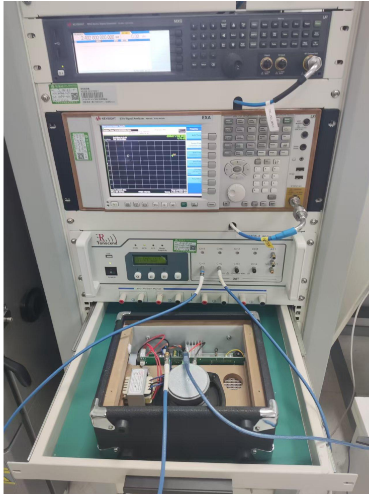
Antenna Terminal Test View
