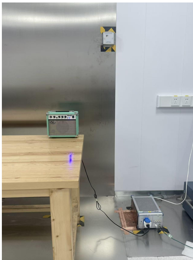
Conducted Emission View
