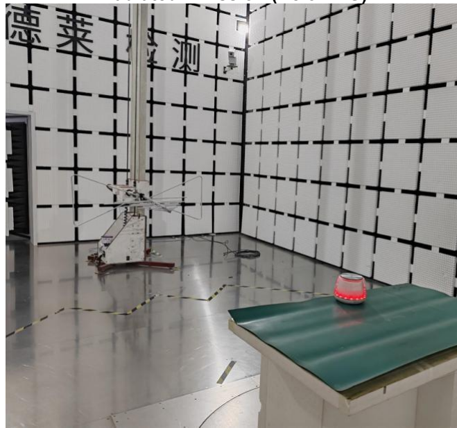
Radiated Emission (Below 1G)
