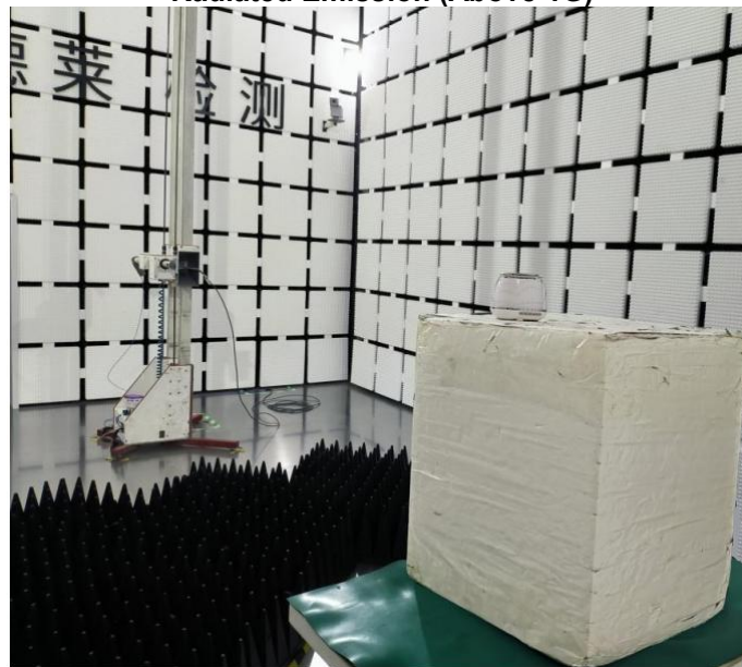
Radiated Emission (Above 1G)
