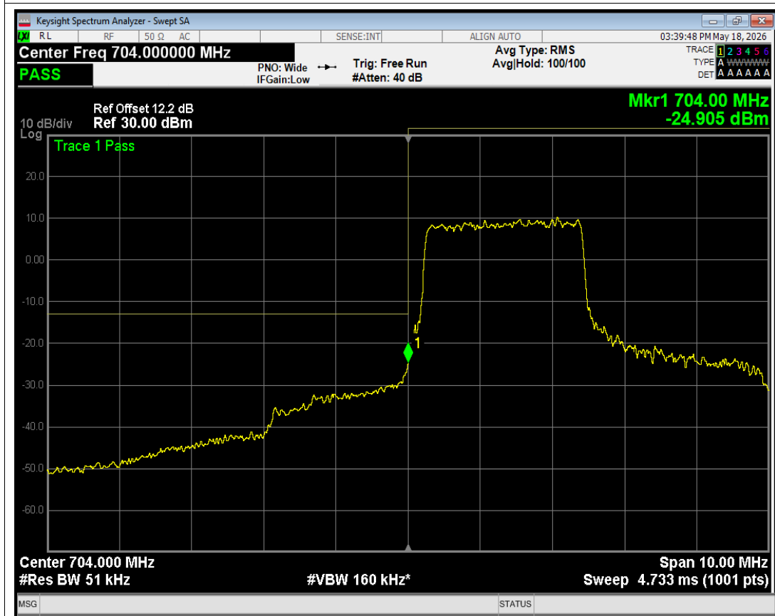
Band17 QPSK BW=5MHz Channel=23755 RB Size=12 Position=#0 NVNT
