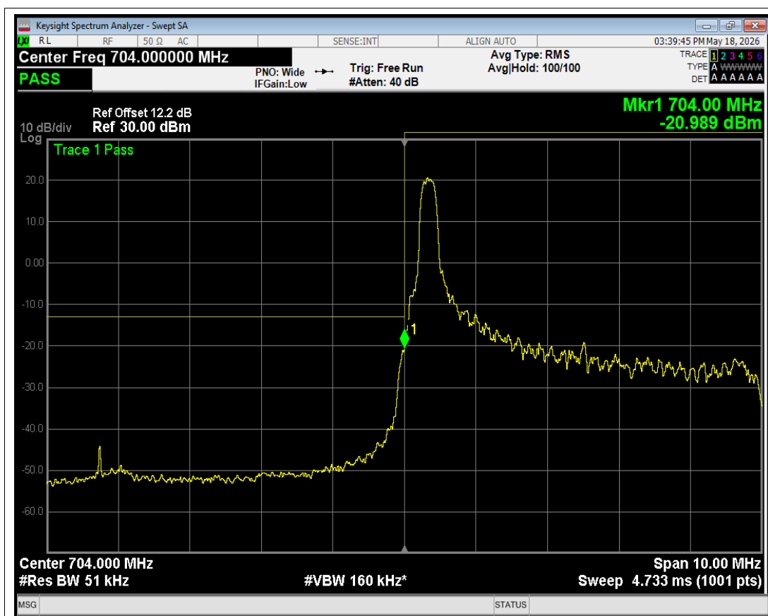
Band17 QPSK BW=5MHz Channel=23755 RB Size=1 Position=#0 NVNT
