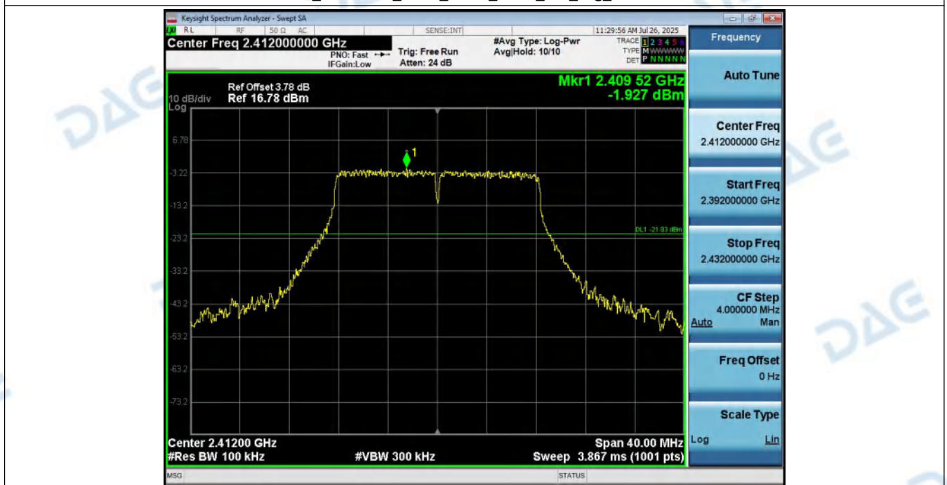
2_Bandedge_NVNT_ANT1_802_11g_2412
