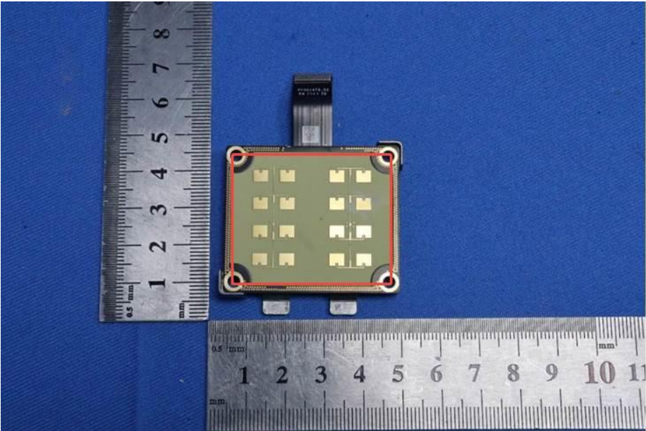
24GHz Behind Radar Antenna
