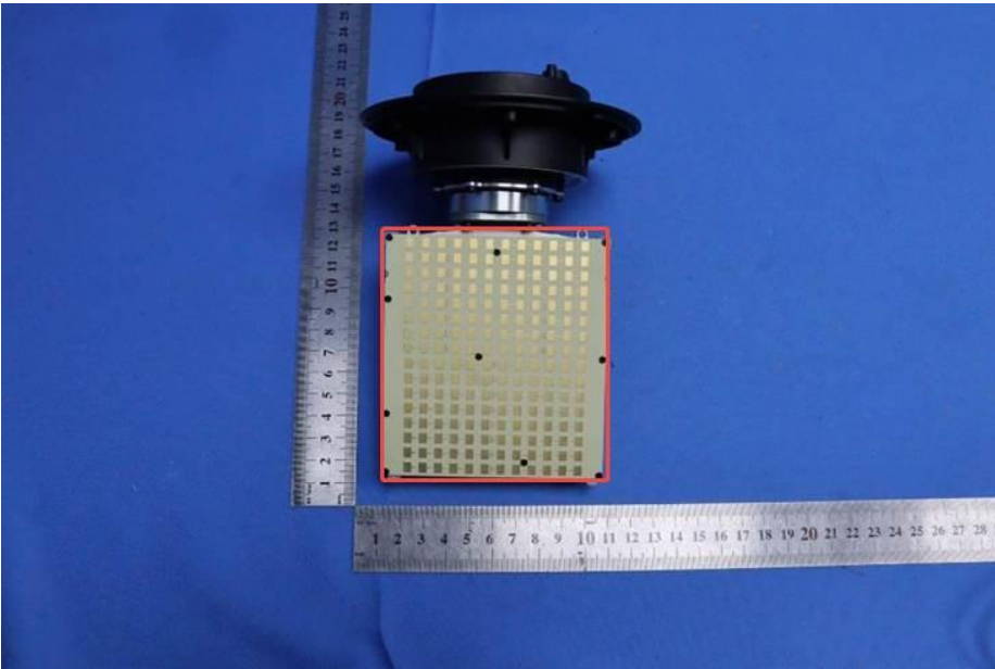
24GHz Front Radar Antenna
