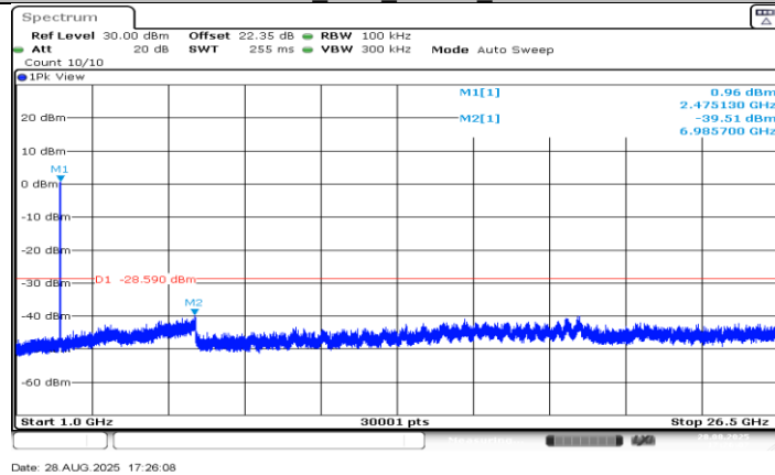
SRD 20M_Ant1_2470.5_1000~26500
