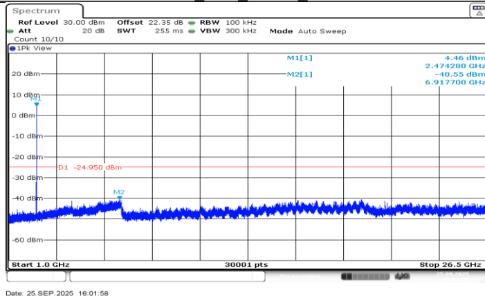
SRD 10M_Ant0_2474.5_1000~26500
