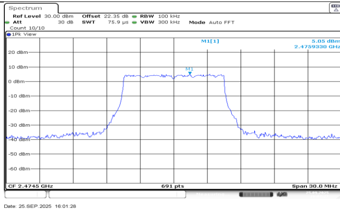
SRD 10M_Ant0_2474.5_0~Reference
