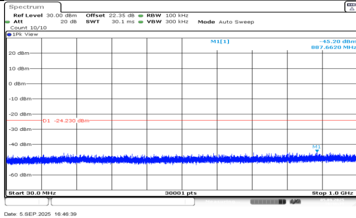
SRD 10M_Ant1_2473.5_30~1000
