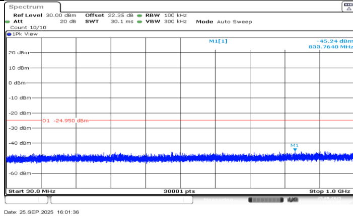
SRD 10M_Ant0_2474.5_30~1000
