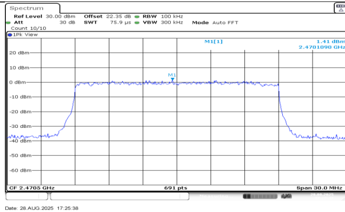
SRD 20M_Ant1_2470.5_0~Reference
