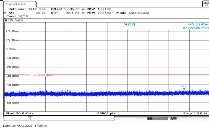
SRD 20M_Ant1_2470.5_30~1000
