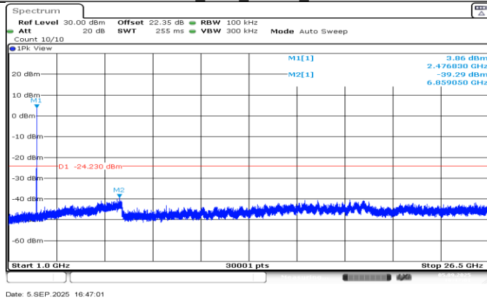
SRD 10M_Ant1_2473.5_1000~26500
