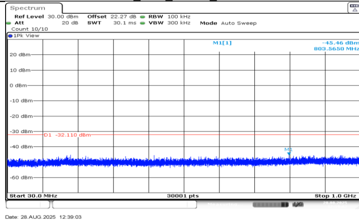
SRD 40M_Ant1_2422.5_30~1000
