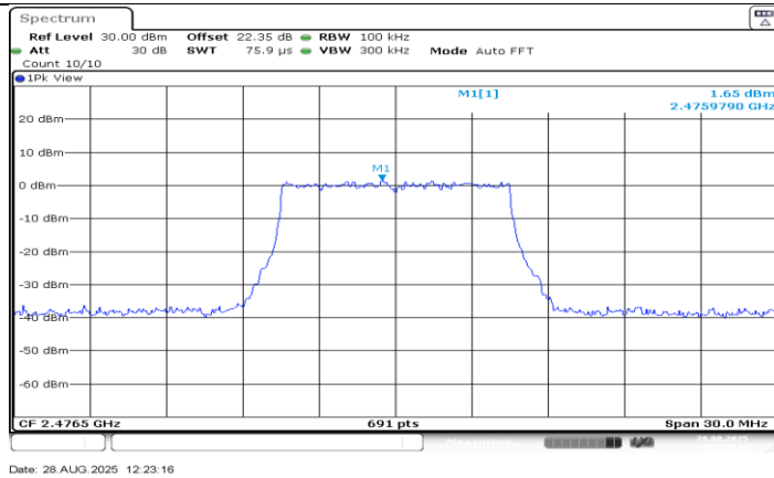
SRD 10M_Ant0_2476.5_0~Reference
