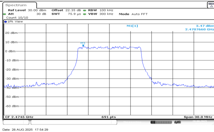
SRD 10M_Ant1_2474.5_0~Reference
