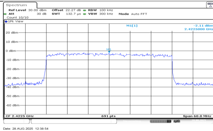
SRD 40M_Ant1_2422.5_0~Reference
