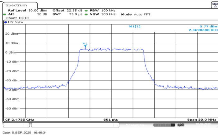
SRD 10M_Ant1_2473.5_0~Reference
