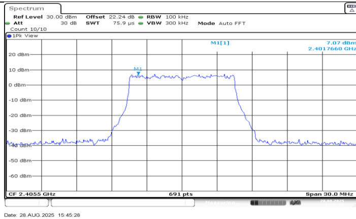
SRD 10M_Ant0_2405.5_0~Reference
