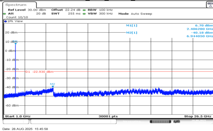
SRD 10M_Ant0_2405.5_1000~26500
