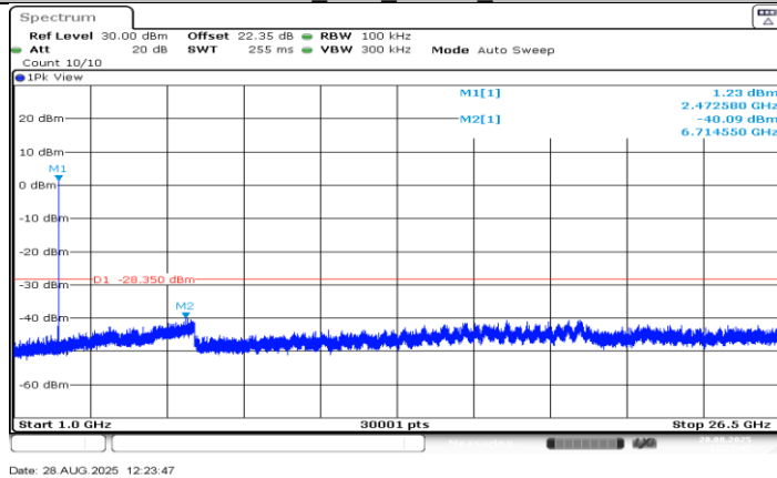
SRD 10M_Ant0_2476.5_1000~26500
