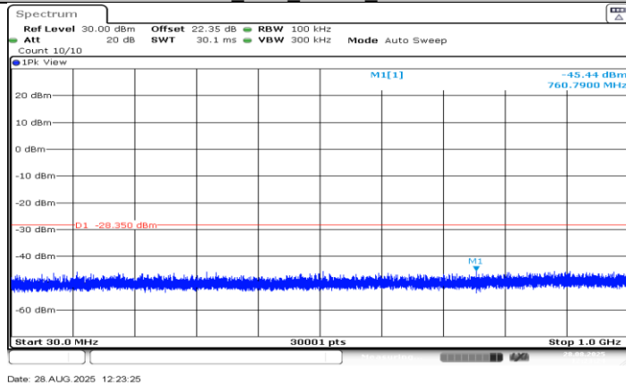
SRD 10M_Ant0_2476.5_30~1000
