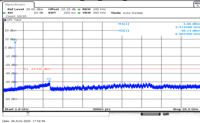
SRD 10M_Ant1_2474.5_1000~26500
