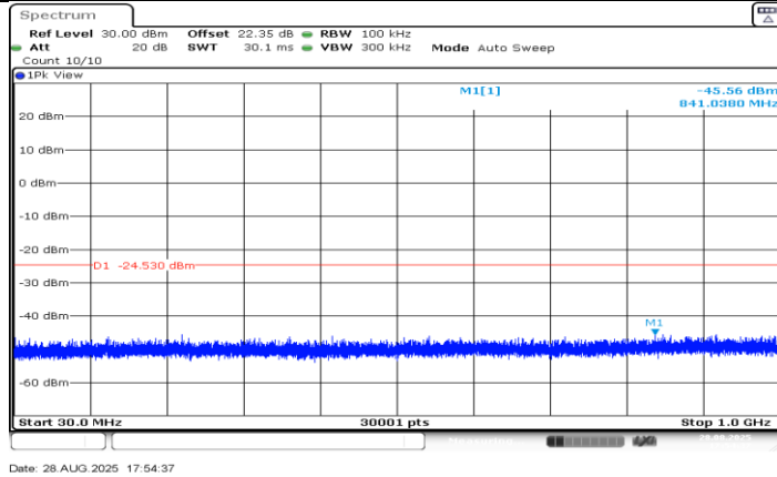
SRD 10M_Ant1_2474.5_30~1000
