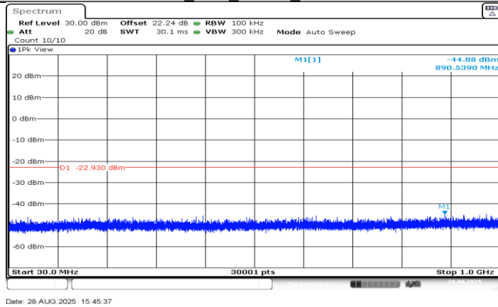
SRD 10M_Ant0_2405.5_30~1000
