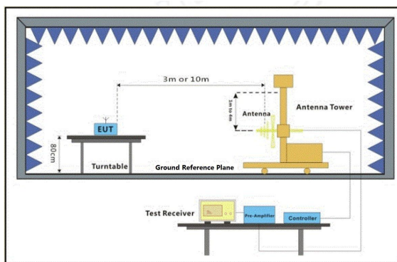
30MHz-1GHz
