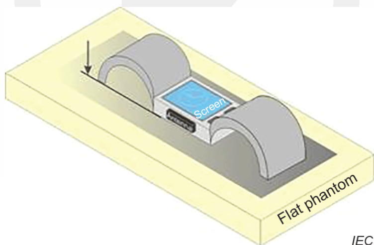
Fig-4.1 Test position for limb-worn devices
