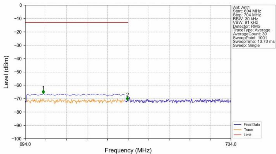
Band12_5MHz_QPSK_LCH_701.5MHz_RB_25_0_NTNV
