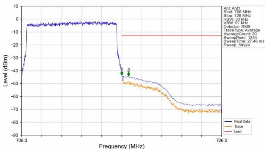
Band12_10MHz_QPSK_HCH_711MHz_RB_50_0_NTNV
