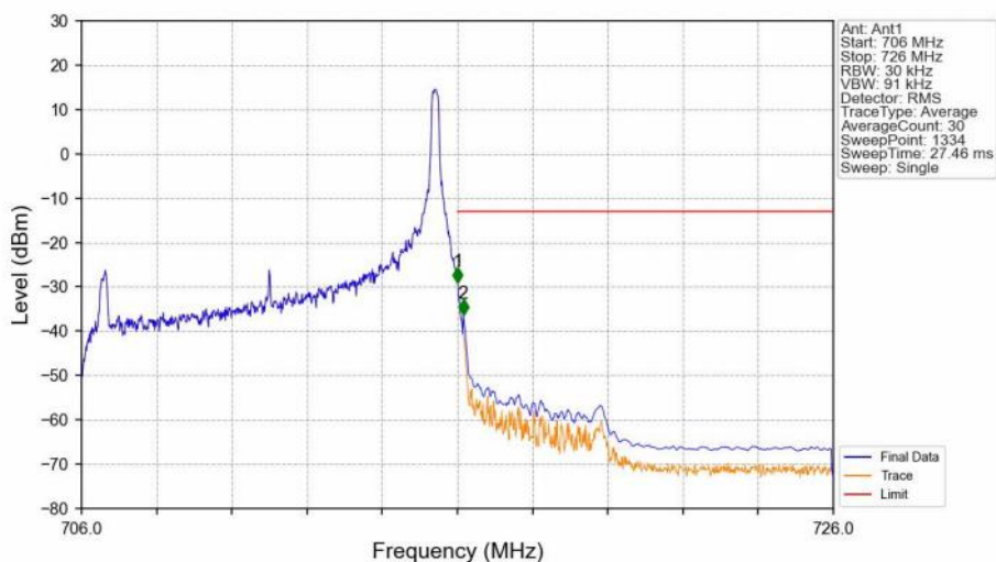
Band12_10MHz_QPSK_HCH_711MHz_RB_1_49_NTNV
