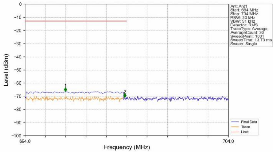
Band12_5MHz_16QAM_LCH_701.5MHz_RB_1_0_NTNV
