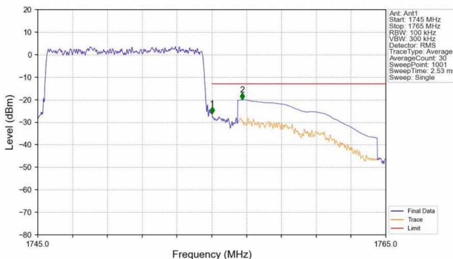
Band4_10MHz_16QAM_HCH_1750MHz_RB_50_0_NTNV
