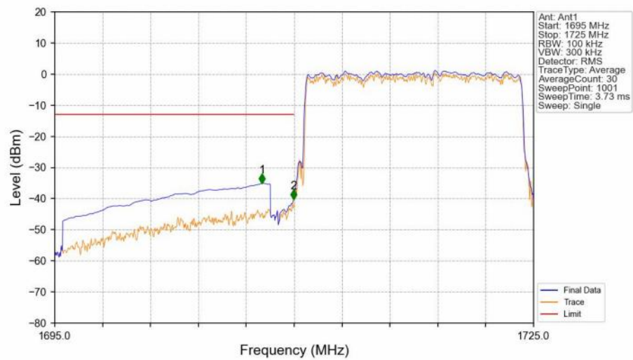
Band4_15MHz_16QAM_LCH_1717.5MHz_RB_75_0_NTNV
