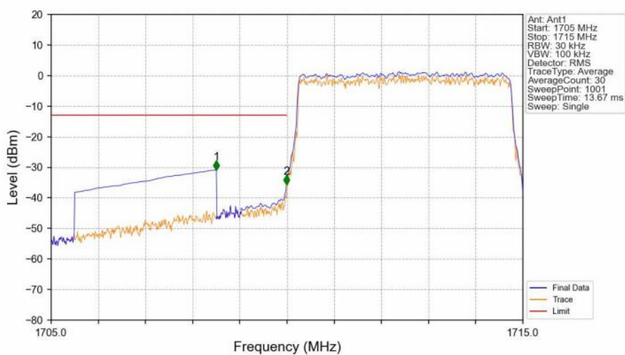
Band4_5MHz_16QAM_LCH_1712.5MHz_RB_25_0_NTNV
