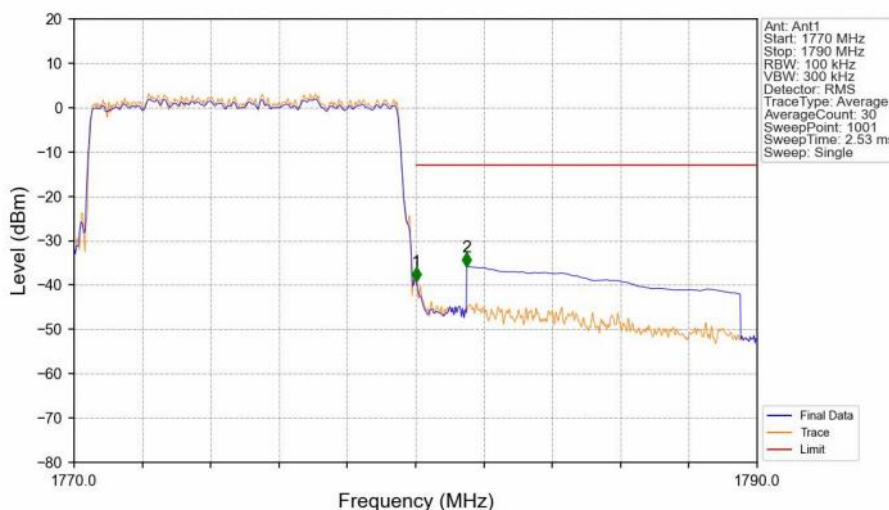
Band66_10MHz_16QAM_HCH_1775MHz_RB_50_0_NTNV
