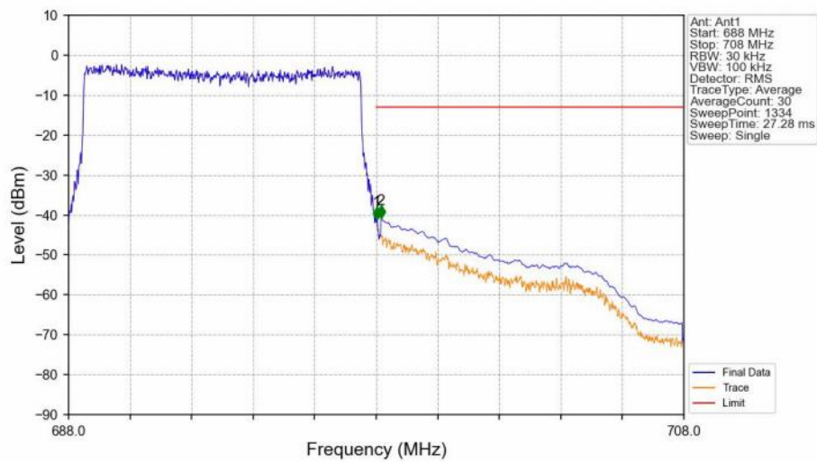
Band71_10MHz_16QAM_HCH_693MHz_RB_50_0 NTNv
