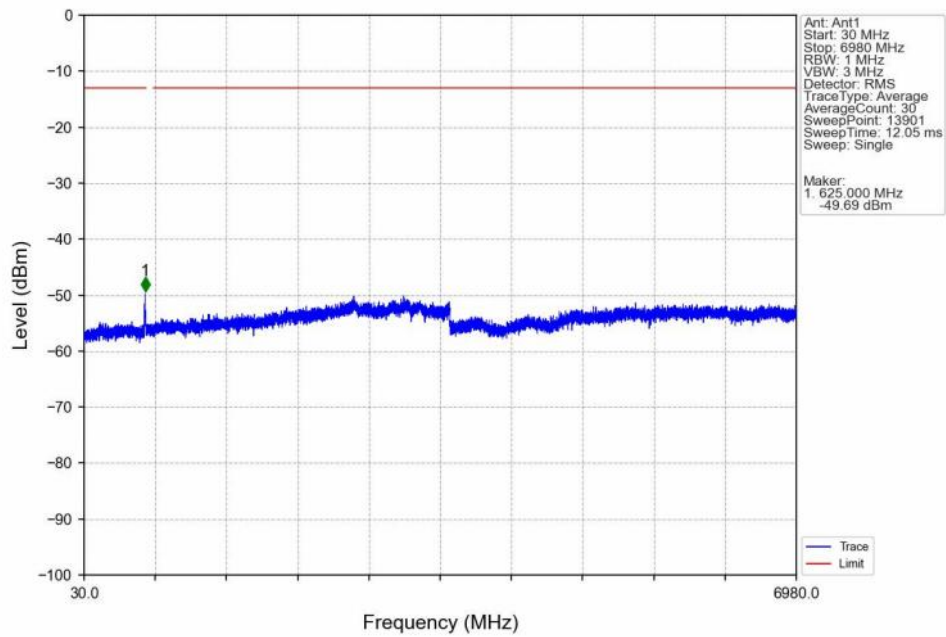
Band71_15MHz_QPSK_LCH_670.5MHz_RB_75_0_NTNV
