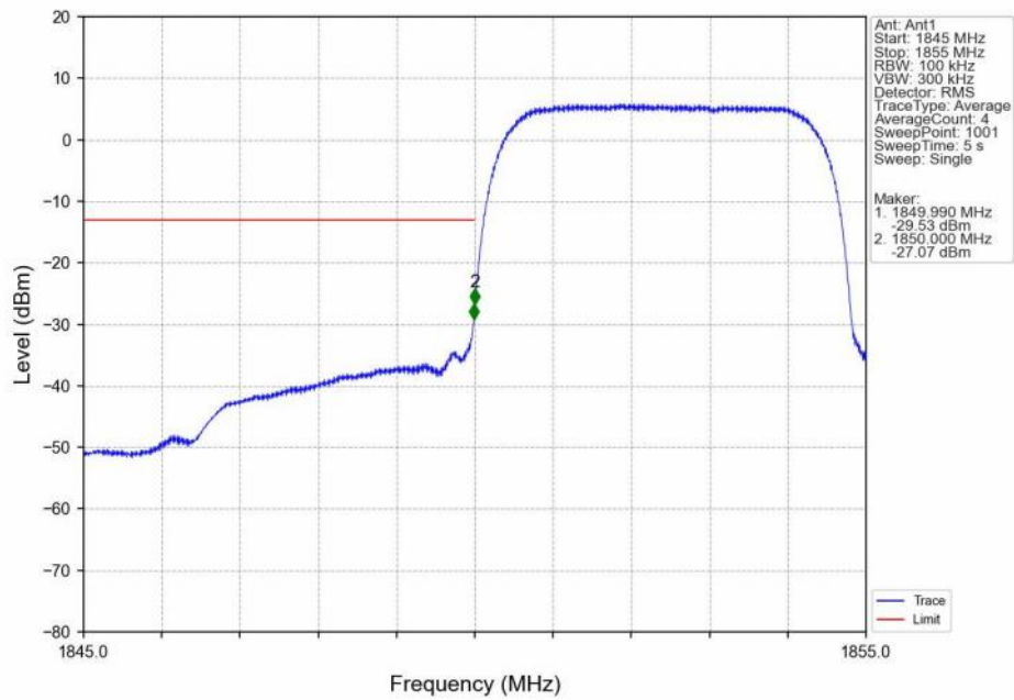
Band2_HSUPA_LCH_1852.4MHz_Subtest 1_NTNV
