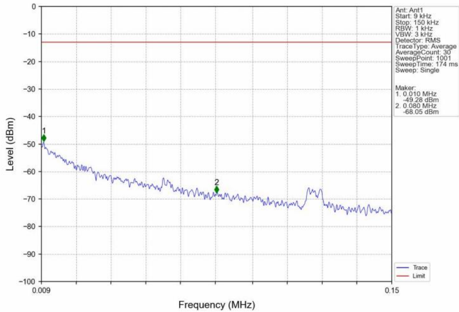
Band2_15MHz_16QAM_MCH_1880MHz_RB_1_0_NTNV
