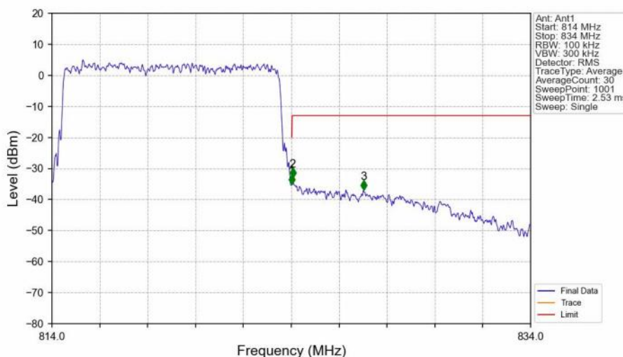
Band26a_10MHz_QPSK_HCH_819MHz_RB_50_0_NTNV
