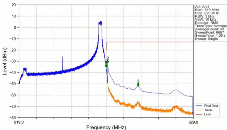
Band26a_5MHz_16QAM_HCH_821.5MHz_RB_1_24_NTNV
