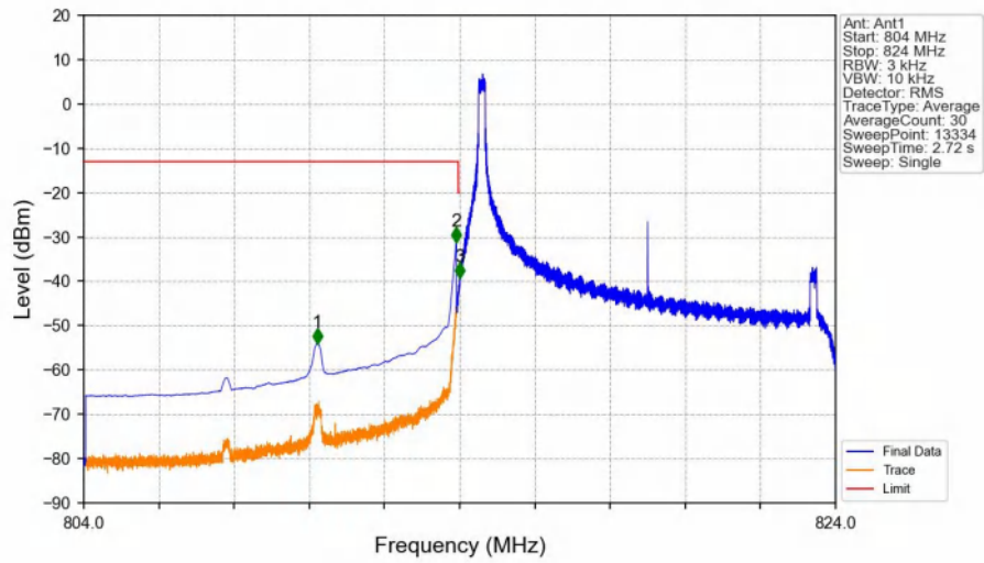
Band26a_10MHz_16QAM_LCH_819MHz_RB_1_0_NTNV
