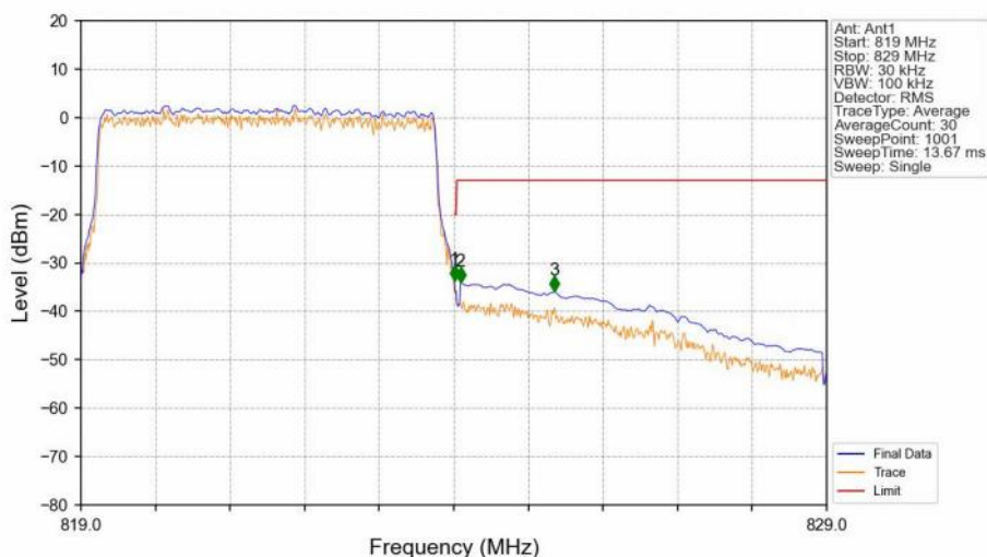
Band26a_5MHz_16QAM_HCH_821.5MHz_RB_25_0_NTNV
