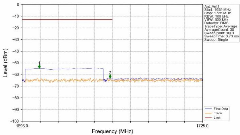
Band66_15MHz_16QAM_LCH_1717.5MHz_RB_75_0_NTNV
