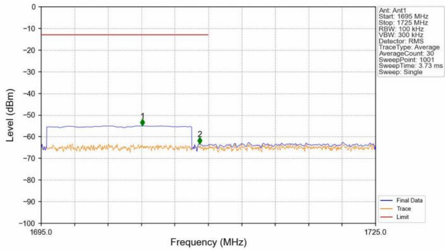
Band66_15MHz_QPSK_LCH_1717.5MHz_RB_75_0_NTNV
