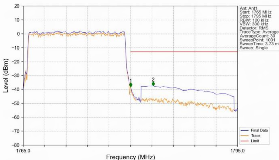
Band66_15MHz_16QAM_HCH_1772.5MHz_RB_75_0_NTNV
