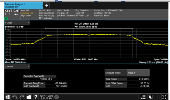
IEEE 802.11g Channel 11 20MHz Antenna 0
